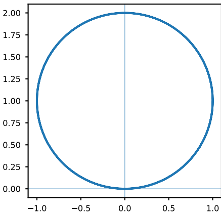
Circle: r = 2a \sin \theta ( a = 1 )
