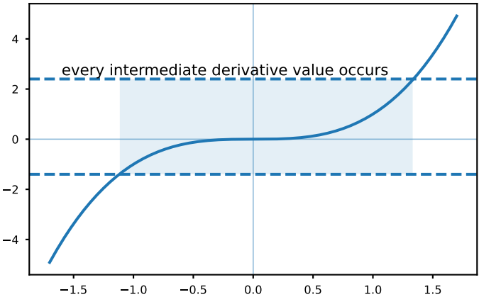
Darboux property of derivatives
