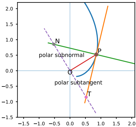
Polar tangent, normal, subtangent, and subnormal
