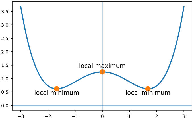
Local maxima and minima
