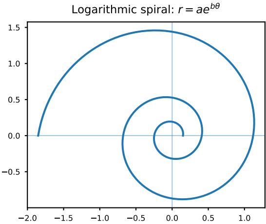
Fig. 25. Logarithmic spiral
