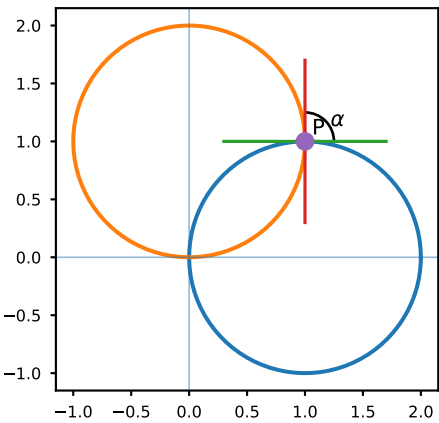
Angle of intersection of two polar curves
