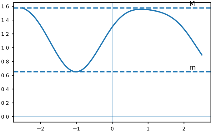
Bounded continuous function on a closed interval
