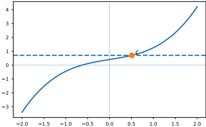
Intermediate Value Theorem
