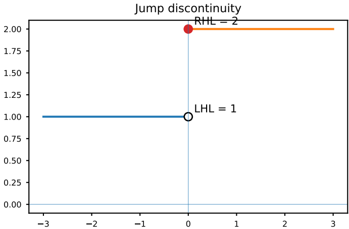
Fig. 2. Jump discontinuity
