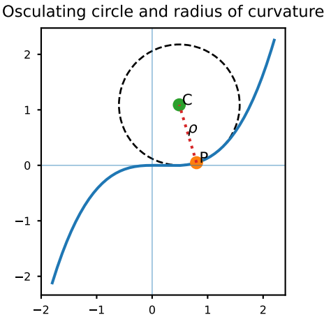
Fig. 28. Osculating circle and radius of curvature
