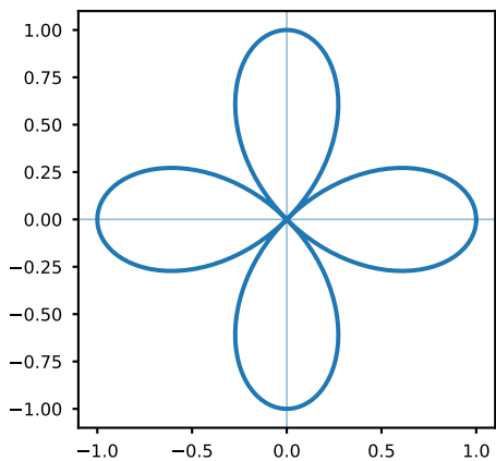
Four-petalled rose: r = a \cos 2\theta
