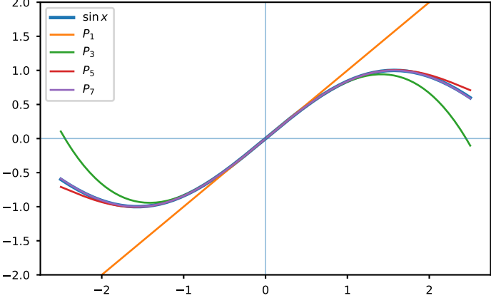
Maclaurin polynomials approximating \sin x
