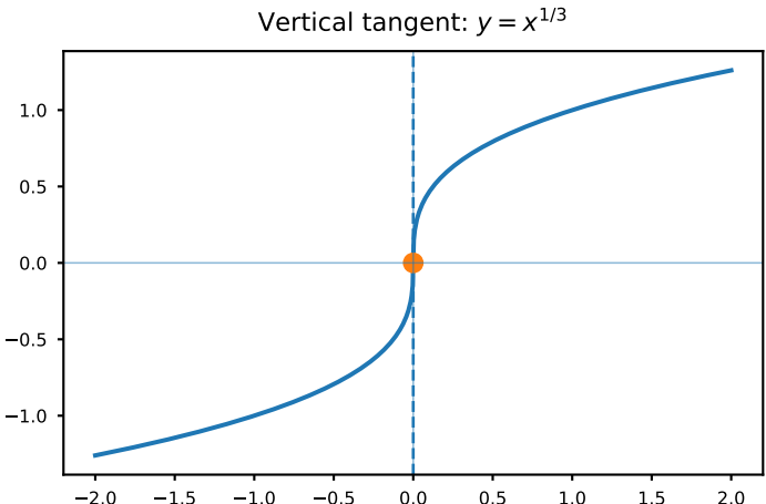
Fig. 8. Vertical tangent
