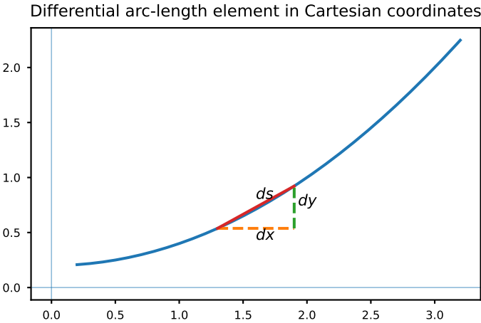
Fig. 29. Cartesian arc-length element
