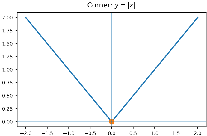
Fig. 6. Corner point
