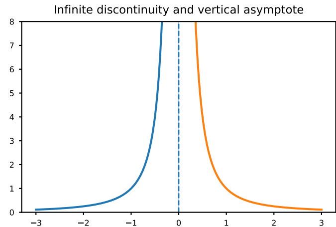
Fig. 3. Infinite discontinuity
