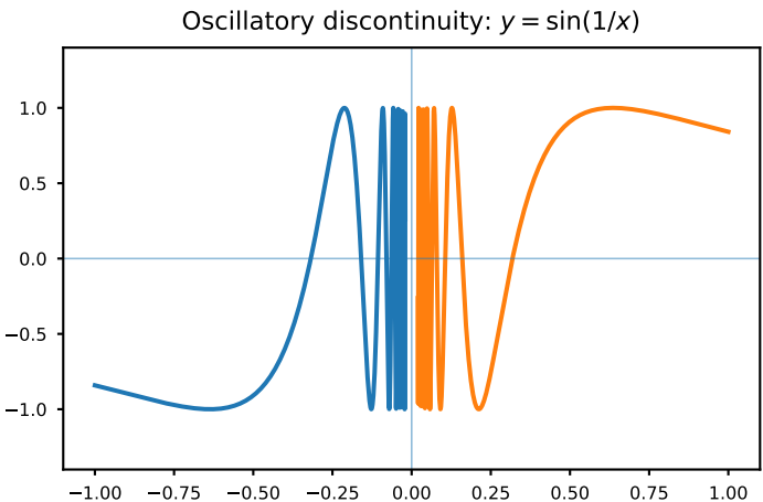
Fig. 4. Oscillatory discontinuity
