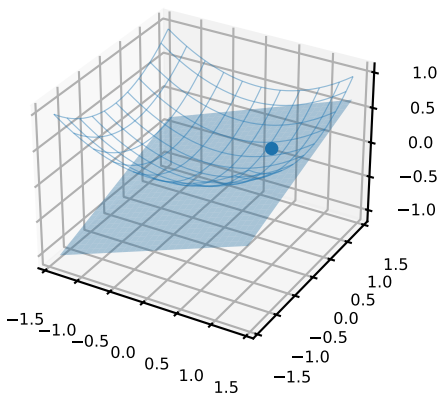
Fig. 10. Tangent plane and total differential
