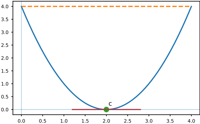
Rolle's Theorem
