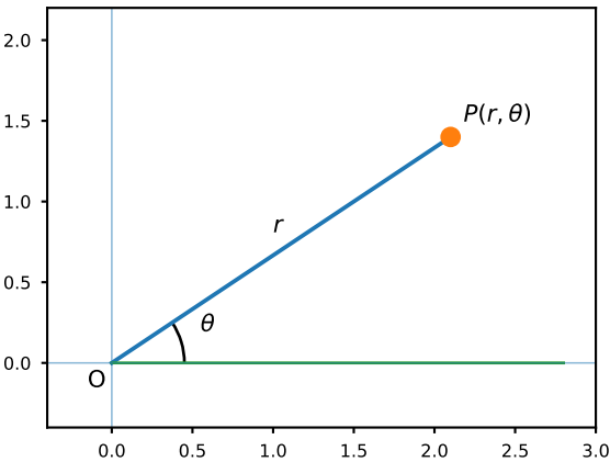
Basic polar-coordinate geometry
