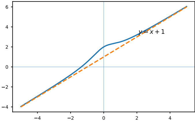
Oblique asymptote
