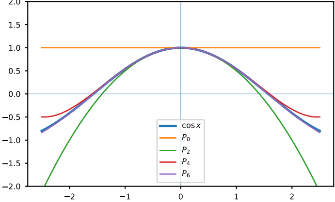
Maclaurin polynomials approximating \cos x
