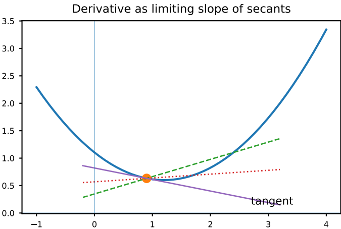
Fig. 5. Derivative: secant to tangent
