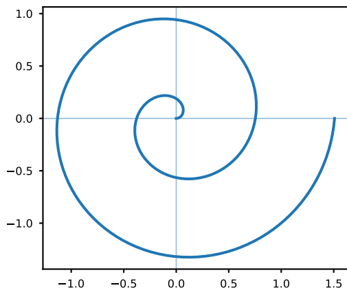
Archimedean spiral: r = a\theta
