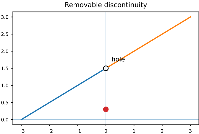
Fig. 1. Removable discontinuity
