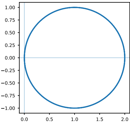
Circle: r = 2a \cos \theta ( a = 1 )
