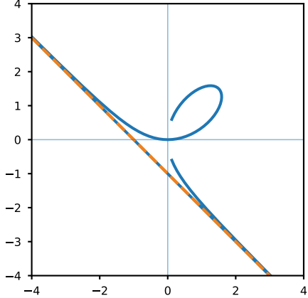
Folium of Descartes: x^3 + y^3 = 3axy ( a = 1 )
