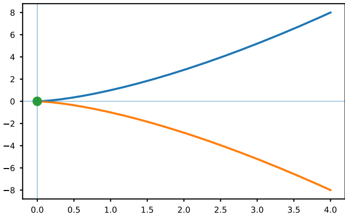
Cusp: y^2 = x^3
