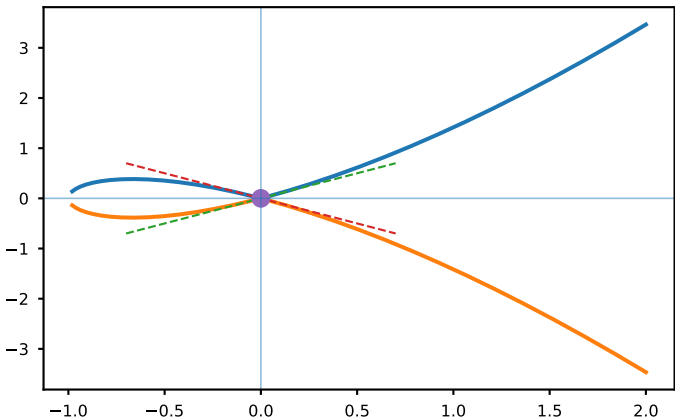
Node: y^2 = x^2(x + 1) with two distinct tangents
