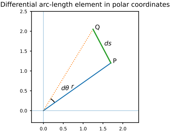
Fig. 30. Polar arc-length element
