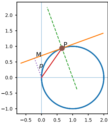
Polar tangent, normal, and perpendicular from the pole
