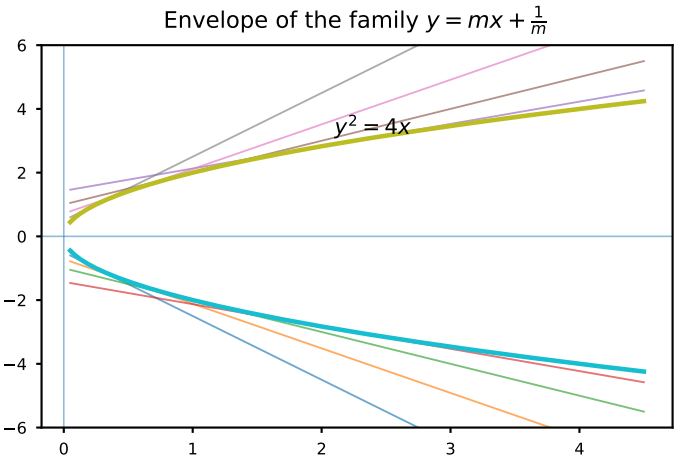
Fig. 49. Envelope of y = mx + 1/m
