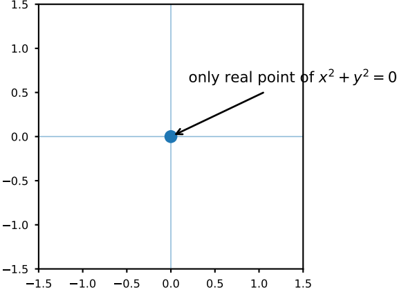
Isolated (conjugate) point
