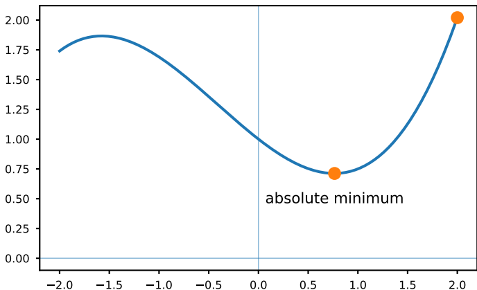
Extreme Value Theorem absolute maximum
