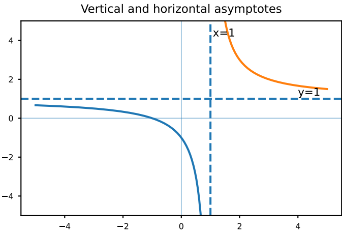
Fig. 32. Vertical and horizontal asymptotes
