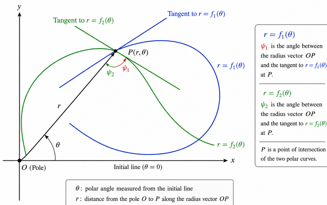
Figure 2.7: Angle of Intersection in Polar coordinates
