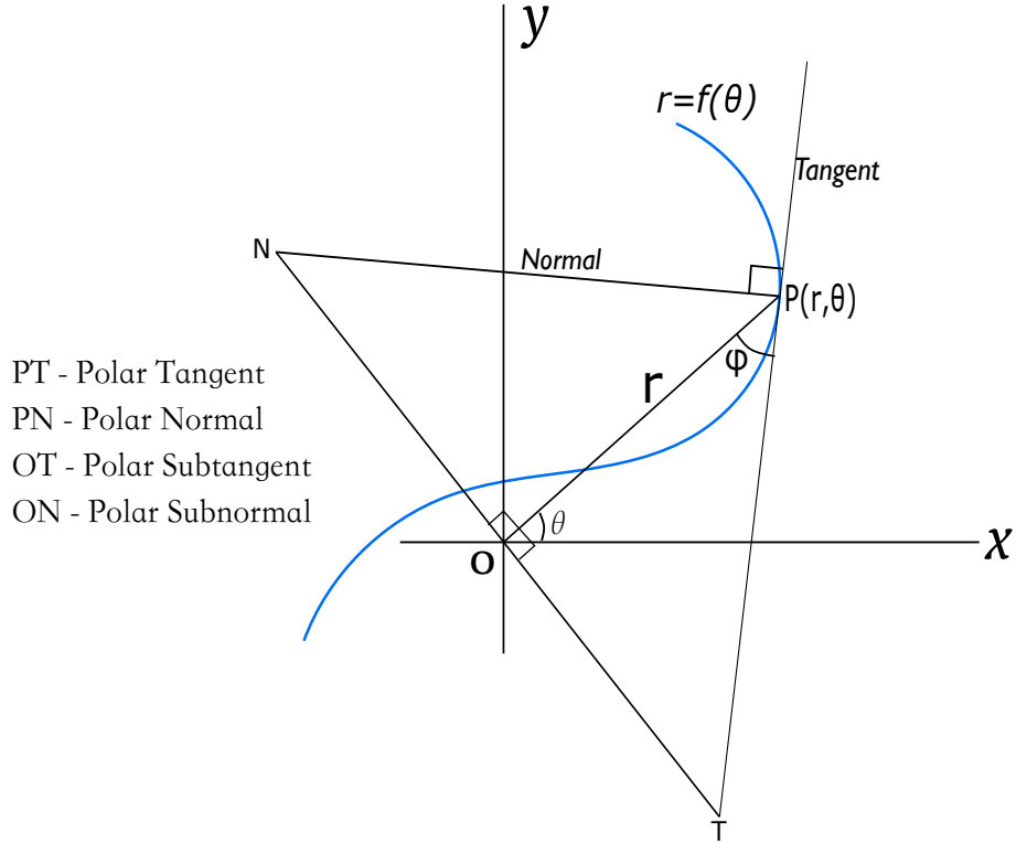
Figure 2.8: Polar Tangent, Polar Normal, Polar Subtangent and Polar Subnormal.
