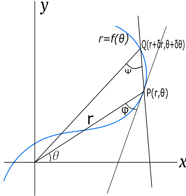
Figure 2.5: Angle \psi \rightarrow \phi as point Q \rightarrow P .
