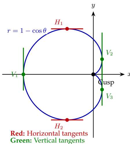
Figure 2.6: The cardioid r = 1 - \cos \theta showing its horizontal tangents, vertical tangents, and cusp.
