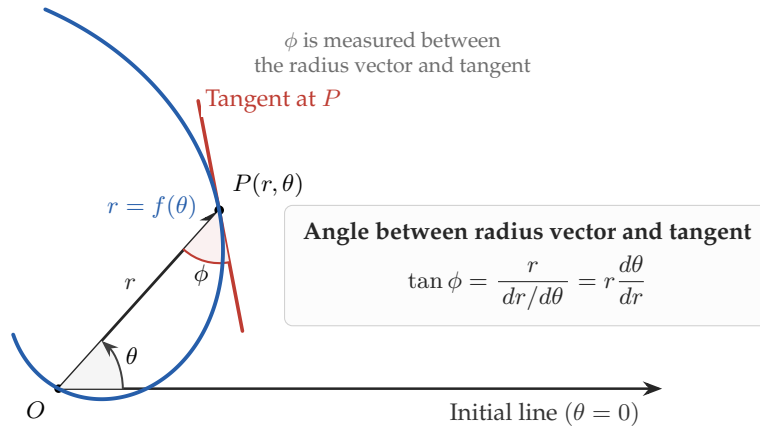
Figure 2.3: Angle \phi between the radius vector OP and the tangent to the polar curve r = f(\theta) at the point P(r, \theta) .
