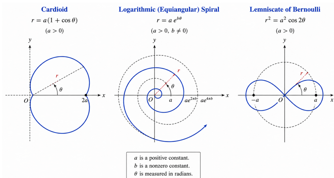
Figure 2.4: The Cardioid, the Logarithmic Spiral and the Lemniscate of Bernoulli
