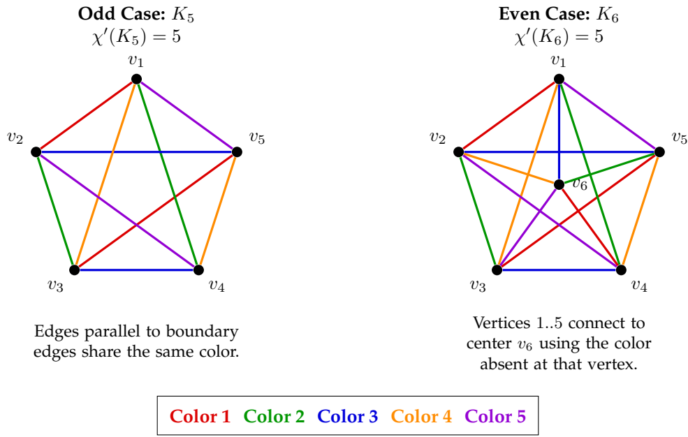
Figure 1.4: Coloring of K_5 and K_6
