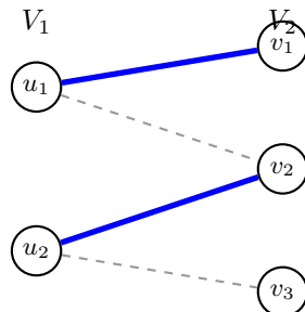
Figure 2.6: Complete Matching of V_1 into V_2 . All vertices in V_1 are blue-connected. Vertex v_3 is left over, which is fine.
