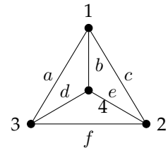
Figure 4.11: * K_4 \eta = (b\ f)(d)(e)(a)(c)
