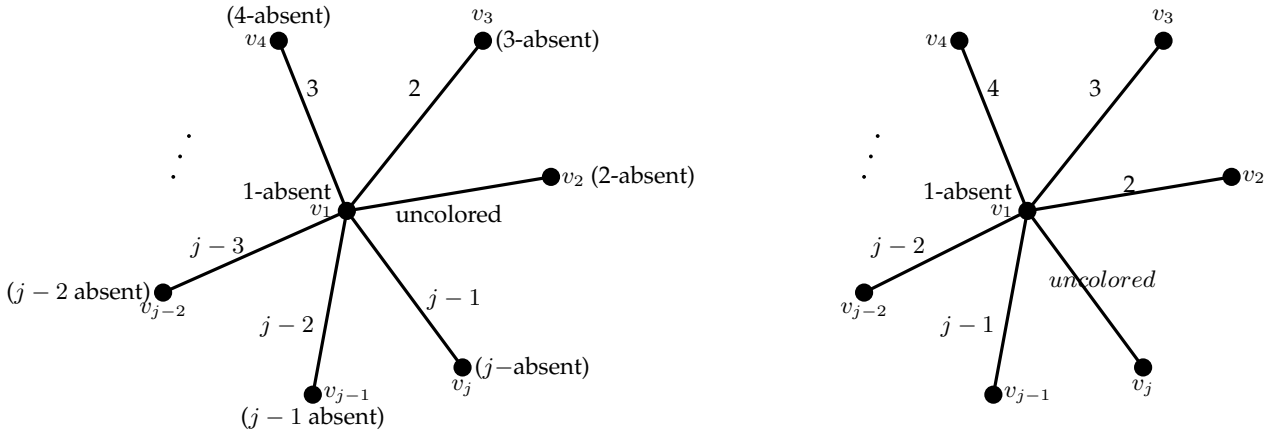
Figure 1.5: Vizing's Theorem
