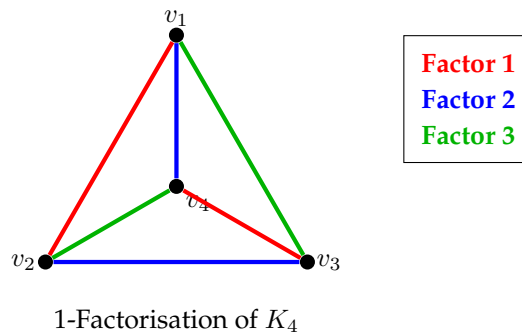
Figure 2.15: A 1-factorisation of the complete graph K_4 . The edges are partitioned into three distinct perfect matchings (Red, Blue, Green).
