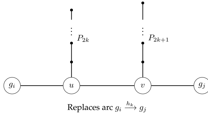
Figure 4.13: Frucht Graph: The subgraph replacing the directed edge from g_i to g_j with color h_k . The asymmetry of the paths P_{2k} and P_{2k+1} enforces the direction and color preservation.
