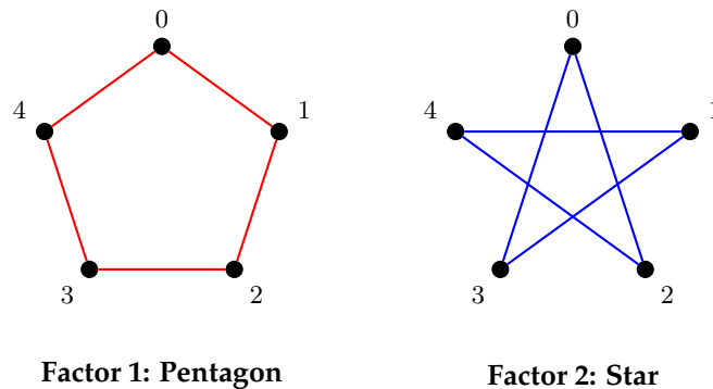
Figure 2.20: Decomposition of K_5 into 2 Hamiltonian Cycles.
