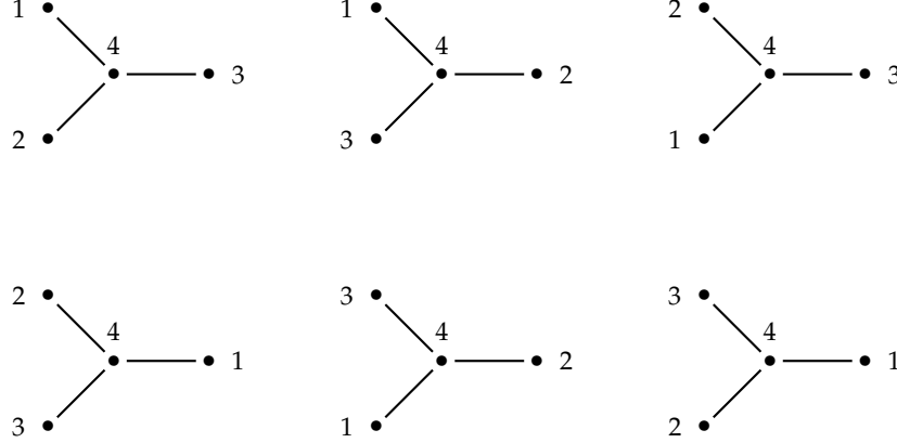
Figure 4.5: Automorphisms of star graph S_4 .
