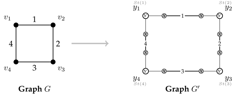
Figure 2.16: Transformation of C_4 into G' with f(v) = 1 .
