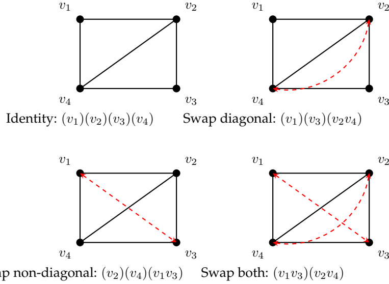
Figure 4.7: Automorphisms of K_4 - e
