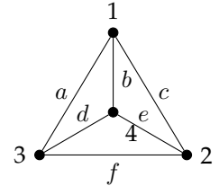
Figure 4.11: * K_4 \eta = (b\ f)(d)(e)(a)(c)
