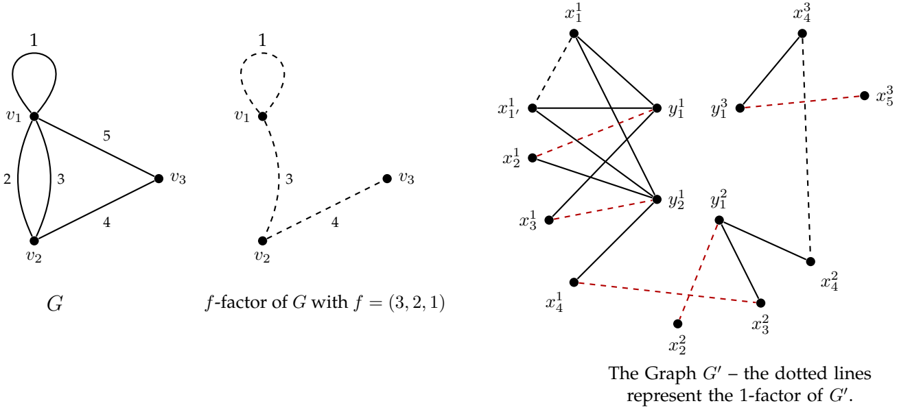
Figure 2.17: Dark dotted edges in G' represent edges induced by f -factor of G for a 1-factor of G' and red dotted edges are additional edges required to produce a 1-factor of G' .
