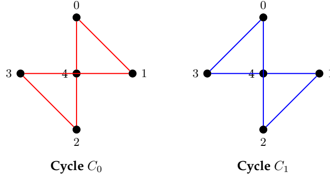
Figure 2.19: Decomposition of K_5 ( n = 2 ). The vertex labeled 4 is the fixed center ( 2n ). Cycle C_0 connects 4 to 0 and 2 (where 2 = n ). Cycle C_1 is the rotation of C_0 .
