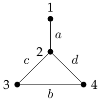
Figure 4.9: * K_{1,3} + e \eta = (a\ b)(c\ d)
