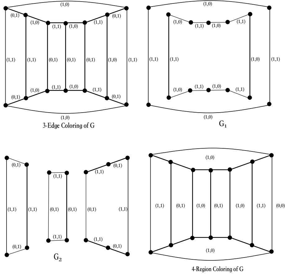
Figure 1.2: Tait's Theorem: \chi'(G) = 3 implies G is 4-region colorable.
