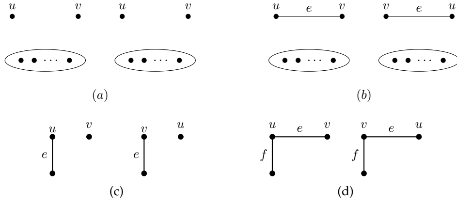
Figure 4.8: Theorem 3.4.5
