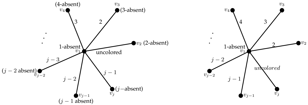
Figure 1.1: Vizing's Theorem
