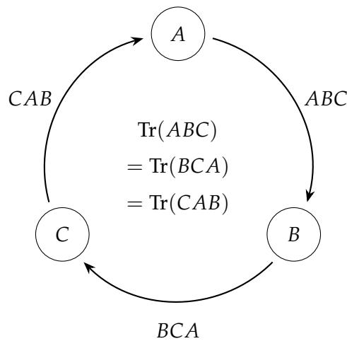
Figure 3.1: Cyclic property of trace. Moving clockwise from any factor preserves the cyclic order and hence the trace.
