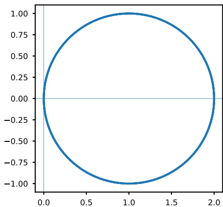
Fig. 15. Circle: r = 2a \cos \theta
