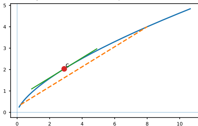
Cauchy Mean Value Theorem: parametric-curve view
