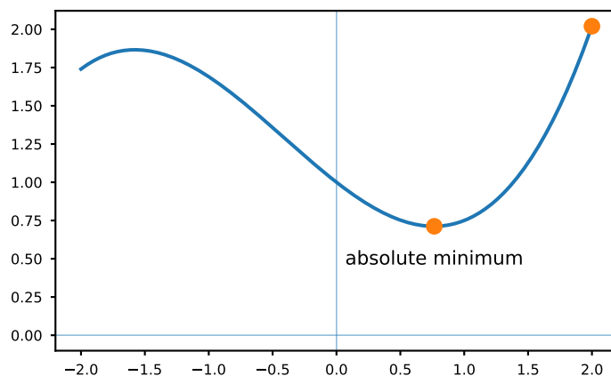
Fig. 40. Extreme Value Theorem
