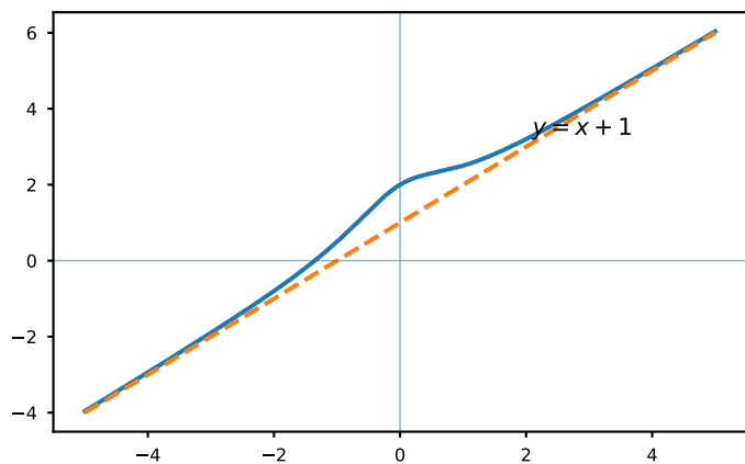
Oblique asymptote
