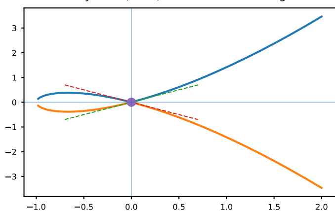
Fig. 35. Singular point: node
