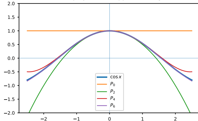
Fig. 48. Maclaurin approximation to \cos x
