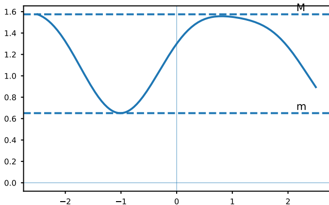
Fig. 39. Boundedness theorem
