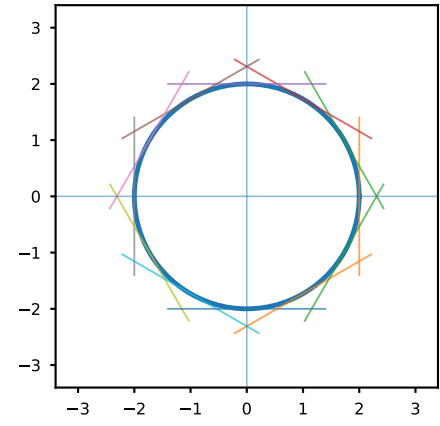
Fig. 50. Envelope of tangent lines to a circle
