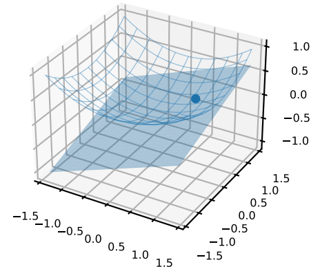
Fig. 10. Tangent plane and total differential
