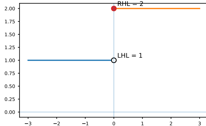
Fig. 2. Jump discontinuity
