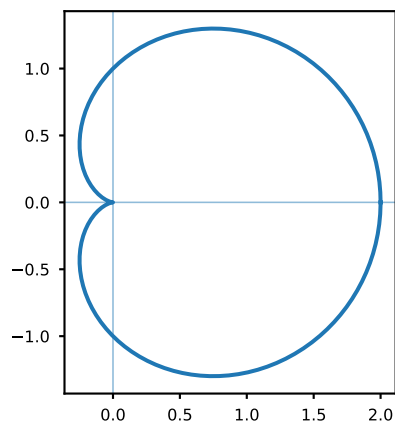
Cardioid: r = a(1 + \cos \theta)
