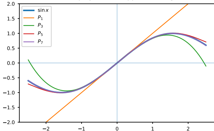
Fig. 47. Maclaurin approximation to \sin x
