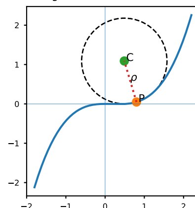
Osculating circle and radius of curvature
