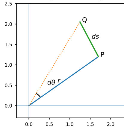
Fig. 30. Polar arc-length element
