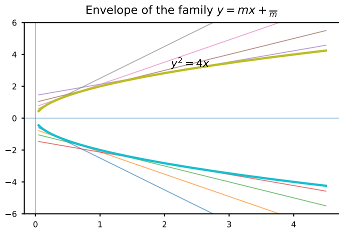
Fig. 49. Envelope of y = mx + 1/m
