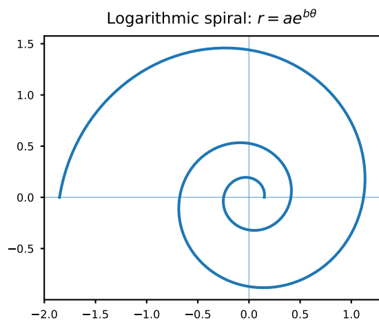
Fig. 25. Logarithmic spiral
