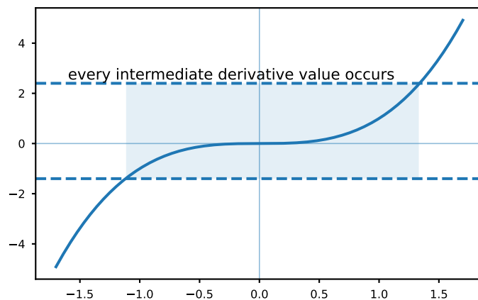
Fig. 42. Darboux theorem
