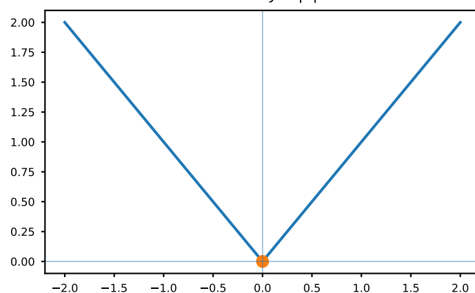
Fig. 6. Corner point
