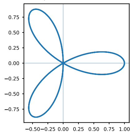
Three-petalled rose: r = a \cos 3\theta
