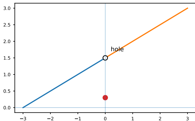
Fig. 1. Removable discontinuity
