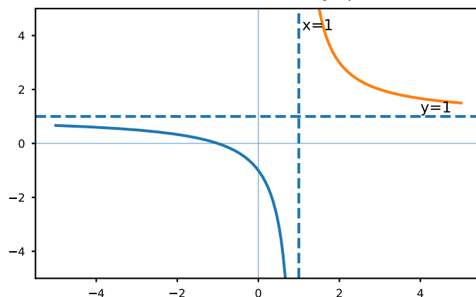
Fig. 32. Vertical and horizontal asymptotes
