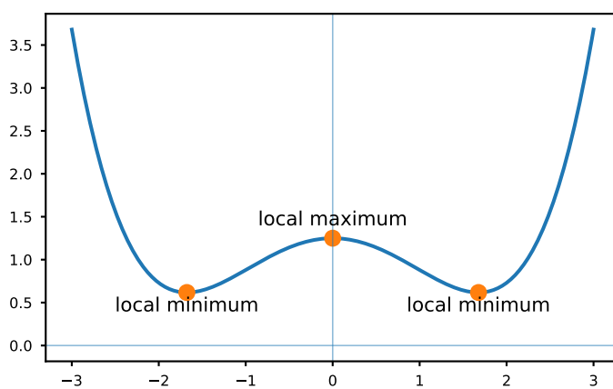
Fig. 38. Local maxima and minima
