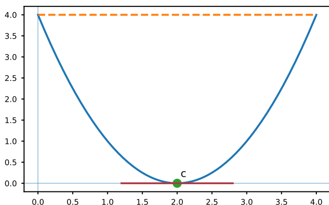
Fig. 43. Rolle's Theorem
