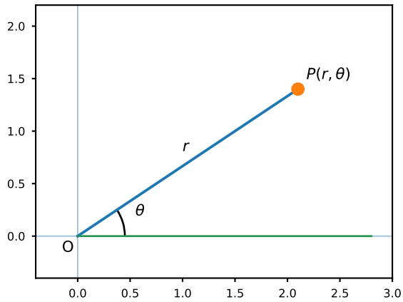
Fig. 11. Basic polar-coordinate geometry
