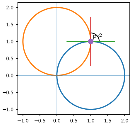
Fig. 13. Angle of intersection of polar curves
