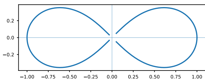
Fig. 21. Lemniscate: r^2 = a^2 \cos 2\theta
