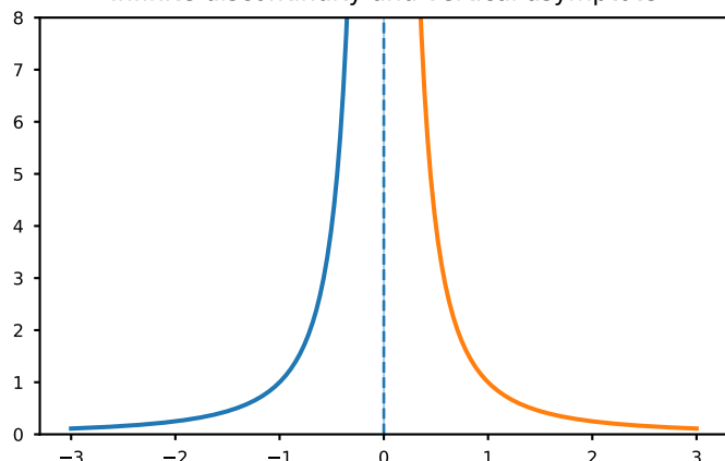
Infinite discontinuity and vertical asymptote
