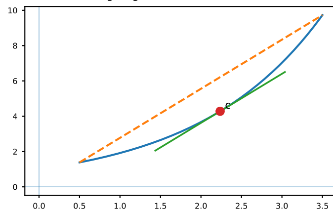
Lagrange Mean Value Theorem
