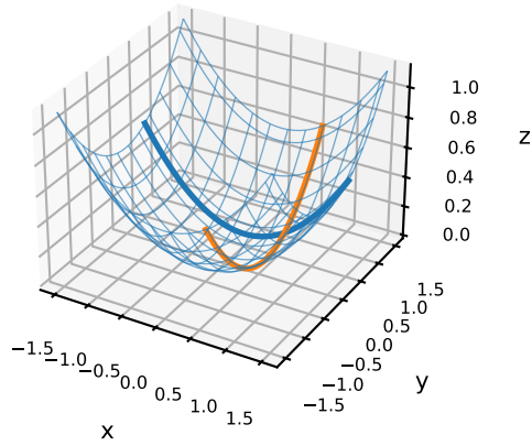
Fig. 9. Partial derivatives on a surface
