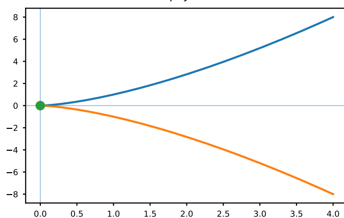
Fig. 36. Singular point: cusp
