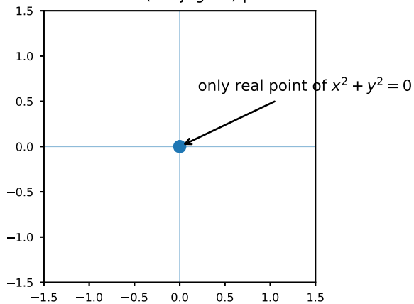
Fig. 37. Singular point: isolated/conjugate point
