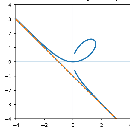
Folium of Descartes: x^3 + y^3 = 3axy ( a = 1 )
