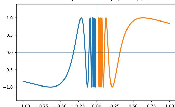
Oscillatory discontinuity: y = \sin(1/x)
