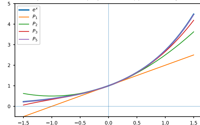
Taylor/Maclaurin polynomials approximating e^x
