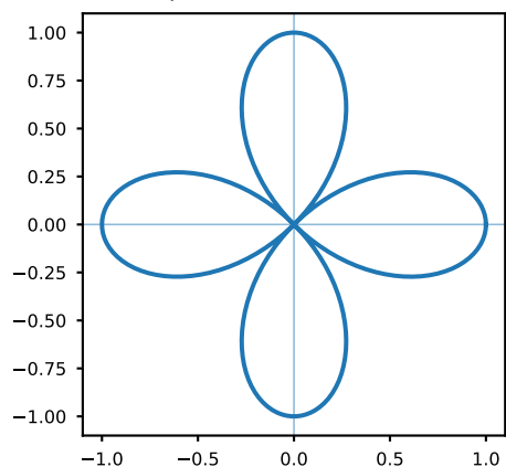
Fig. 23. Four-petalled rose
