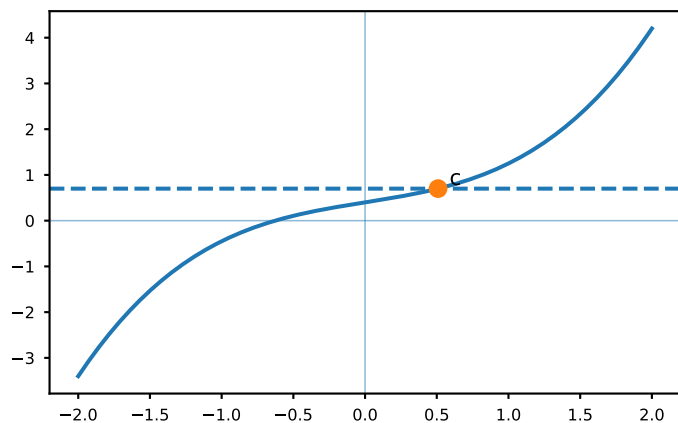
Fig. 41. Intermediate Value Theorem
