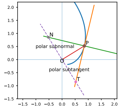
Fig. 14. Polar tangent, normal, subtangent and subnormal
