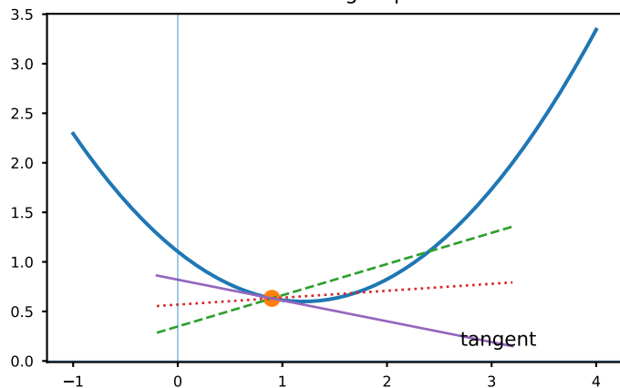
Fig. 5. Derivative: secant to tangent
