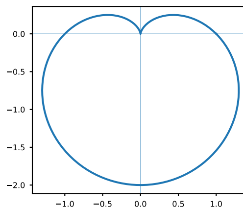
Cardioid: r = a(1 - \sin \theta)
