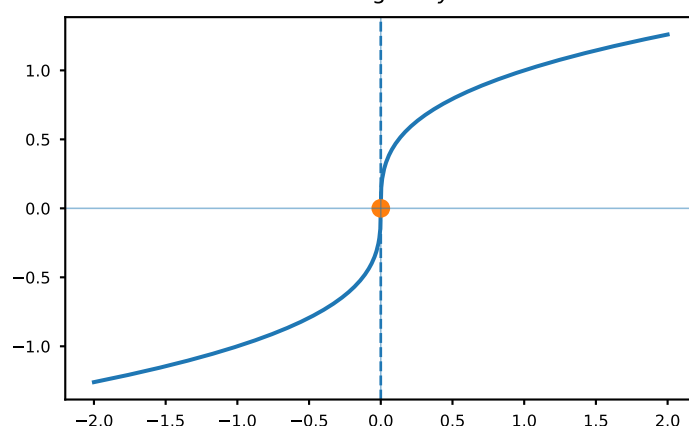
Fig. 8. Vertical tangent
