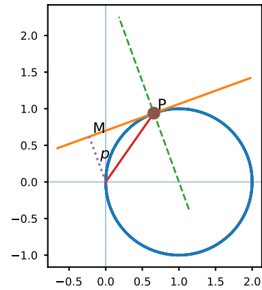
Fig. 12. Polar tangent, normal and perpendicular
