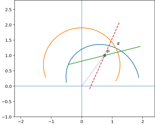
Fig. 13. Angle of intersection of polar curves
