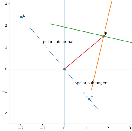
Fig. 14. Polar tangent, normal, subtangent and subnormal
