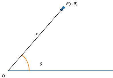
Fig. 11. Basic polar-coordinate geometry
