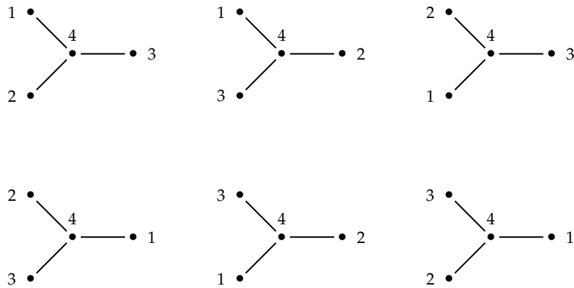
Figure 4.5: Automorphisms of star graph S_4 .
