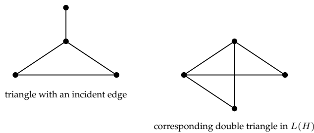
Figure 3.7: A triangle in an edge graph generated by a triangle in the original graph.
