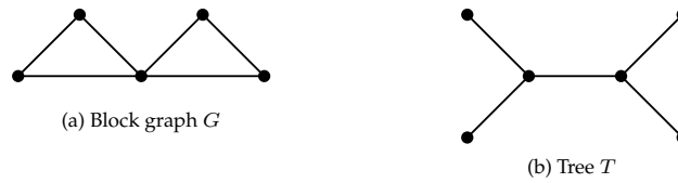
Figure 3.14: A block graph formed by two triangles sharing one vertex, and a tree T whose edge graph is isomorphic to it.
