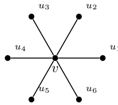
Figure 3.21: The neighbourhood of the central vertex of a star.
