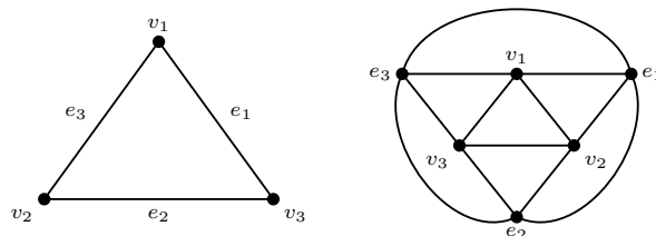
Figure 3.19: A graph G = K_3 and its total graph T(G) .
