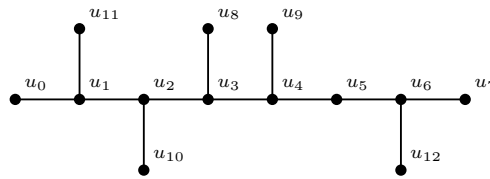
Figure 3.20: A tree realizing the eccentricity sequence [4^2, 5^4, 6^3, 7^4] .
