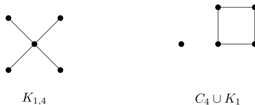
Figure 4.2: A pair of non-isomorphic cospectral graphs.
