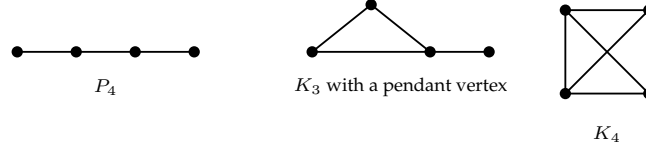
Figure 3.6: Edge graphs of the three tree possibilities in Figure 3.4.
