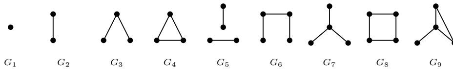
Figure 3.2: The connected graphs used in the proof of Whitney's theorem.
