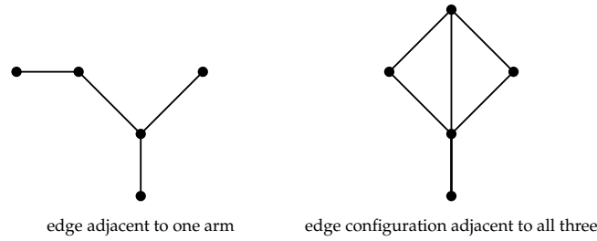
Figure 3.3: The configurations used in the proof of Whitney's theorem.
