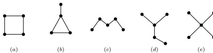
Figure 3.4: Examples of connected graphs with four edges.
