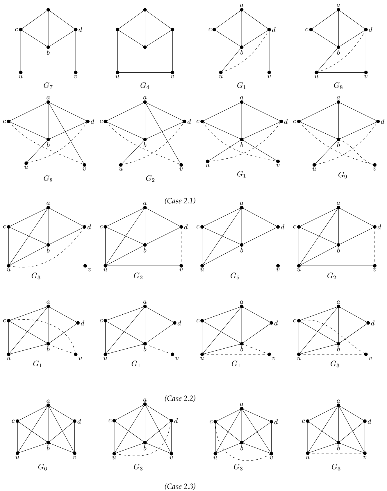
Figure 3.13: Bieleke's Theorem
