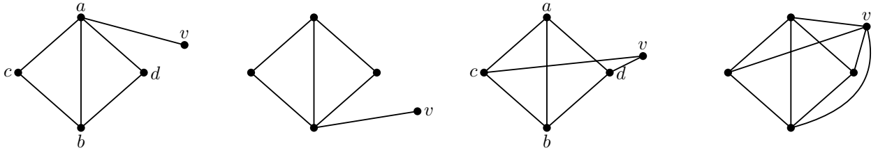
Figure 3.11: The configurations arising in Case 1 of the proof of Beineke's theorem.
