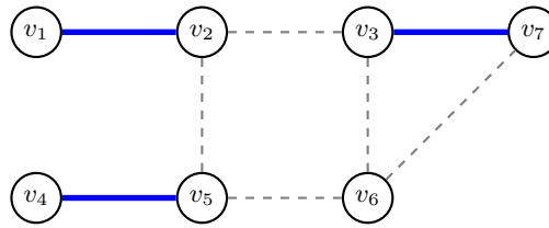
Figure 2.1: Visual representation of the matching M . The blue edges form the matching.
