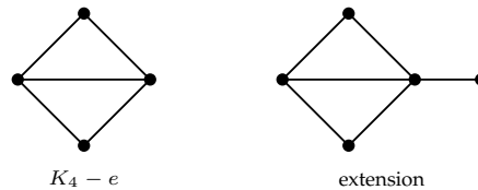
Figure 3.8: The possibilities when a K_{1,3} -free graph has a double triangle with both triangles even.
