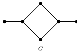
Figure 3.17: A non-Hamiltonian graph with a Hamiltonian edge graph.
