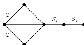
Figure 3.9: The clique configuration used in the proof of Theorem 3.1.10.
