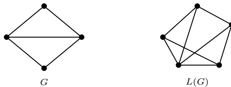
Figure 3.1: The graph G and its edge graph L(G) .
