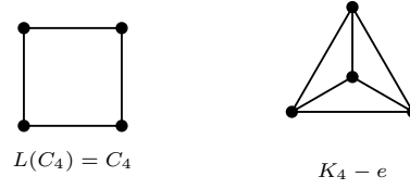
Figure 3.5: The edge graphs of the first two possibilities in Figure 3.4.
