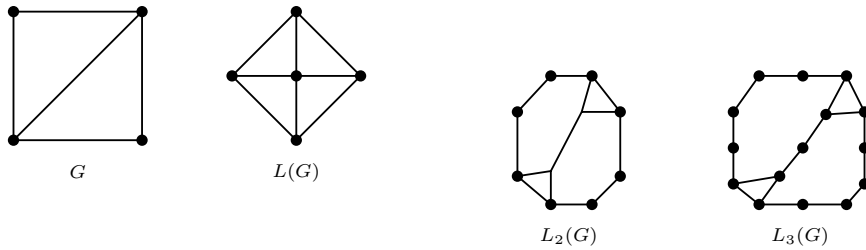
Figure 3.18: Successive subdivisions of a graph.
