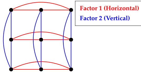
Graph G = F_1 \cup F_2
