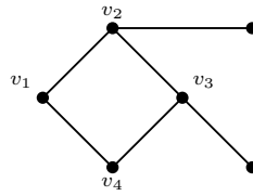
Figure 3.16: The cycle v_1v_2v_3v_4v_1 is a dominating closed trail.
