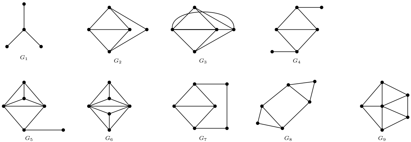
Figure 3.10: The nine forbidden induced subgraphs in Beineke's characterisation of line graphs.
