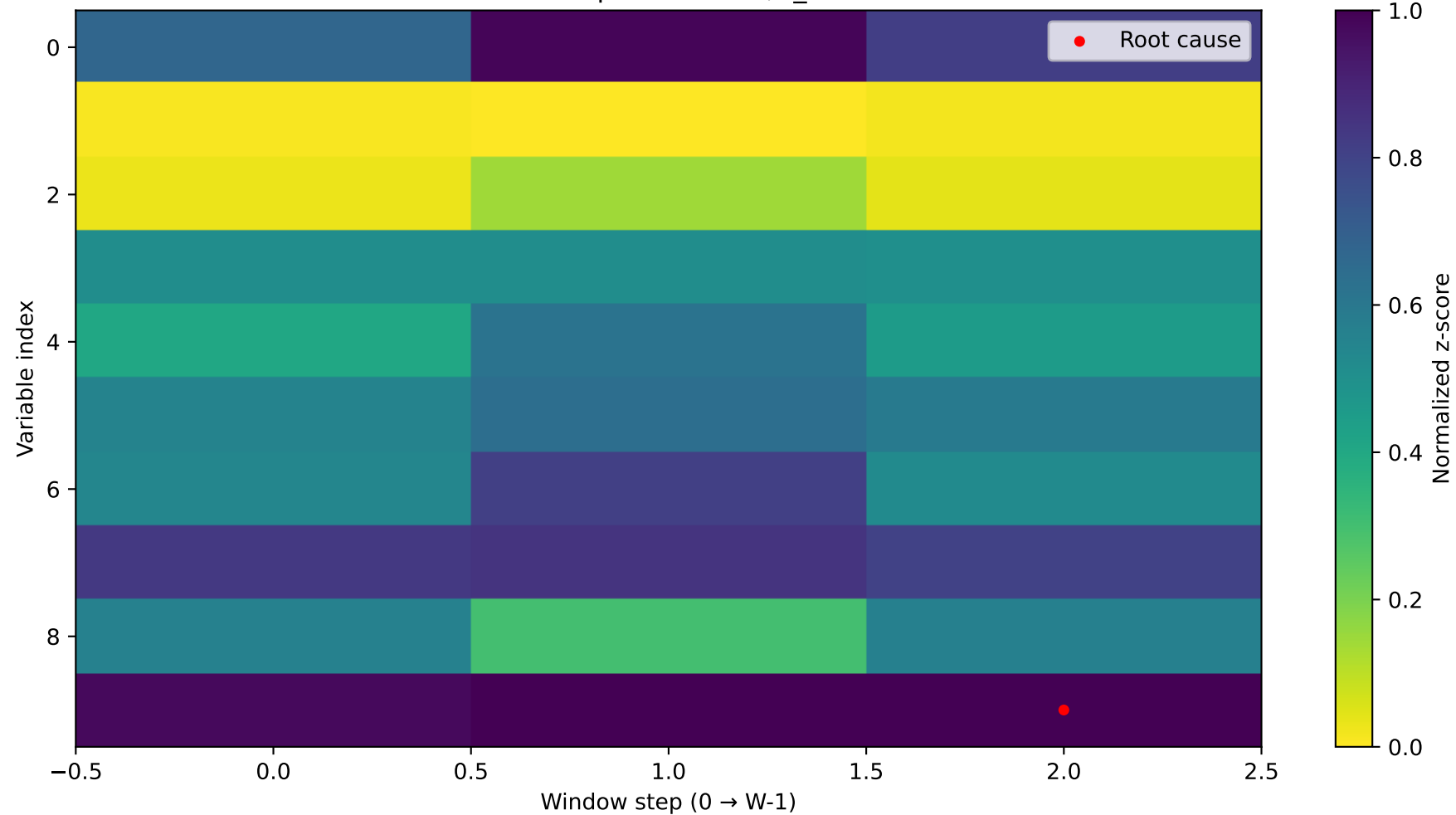
RCA Heatmap Window=3, t_start=6
