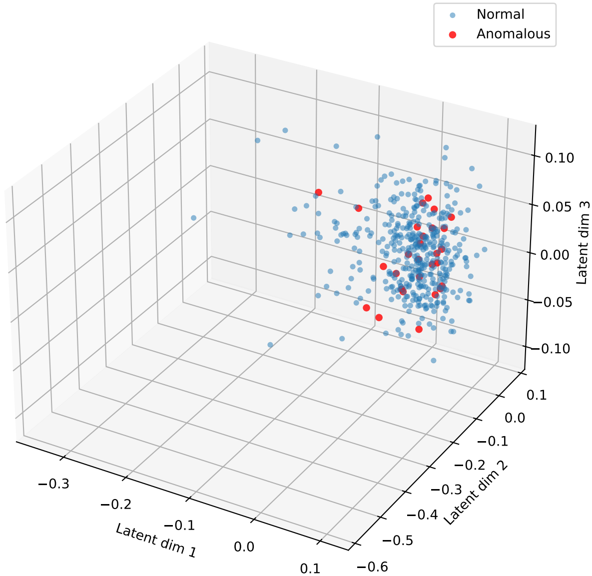
3D Latent Space Clustering (PCA)
