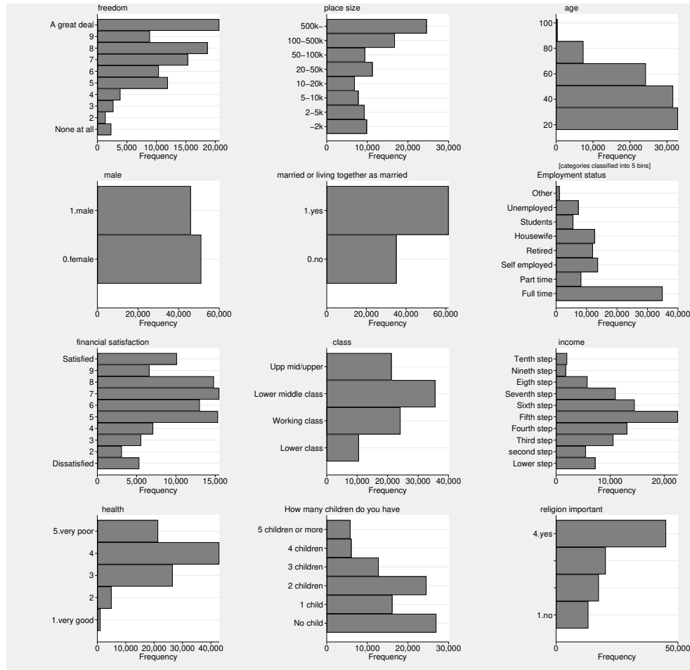
Figure 2: Variables' distribution.
