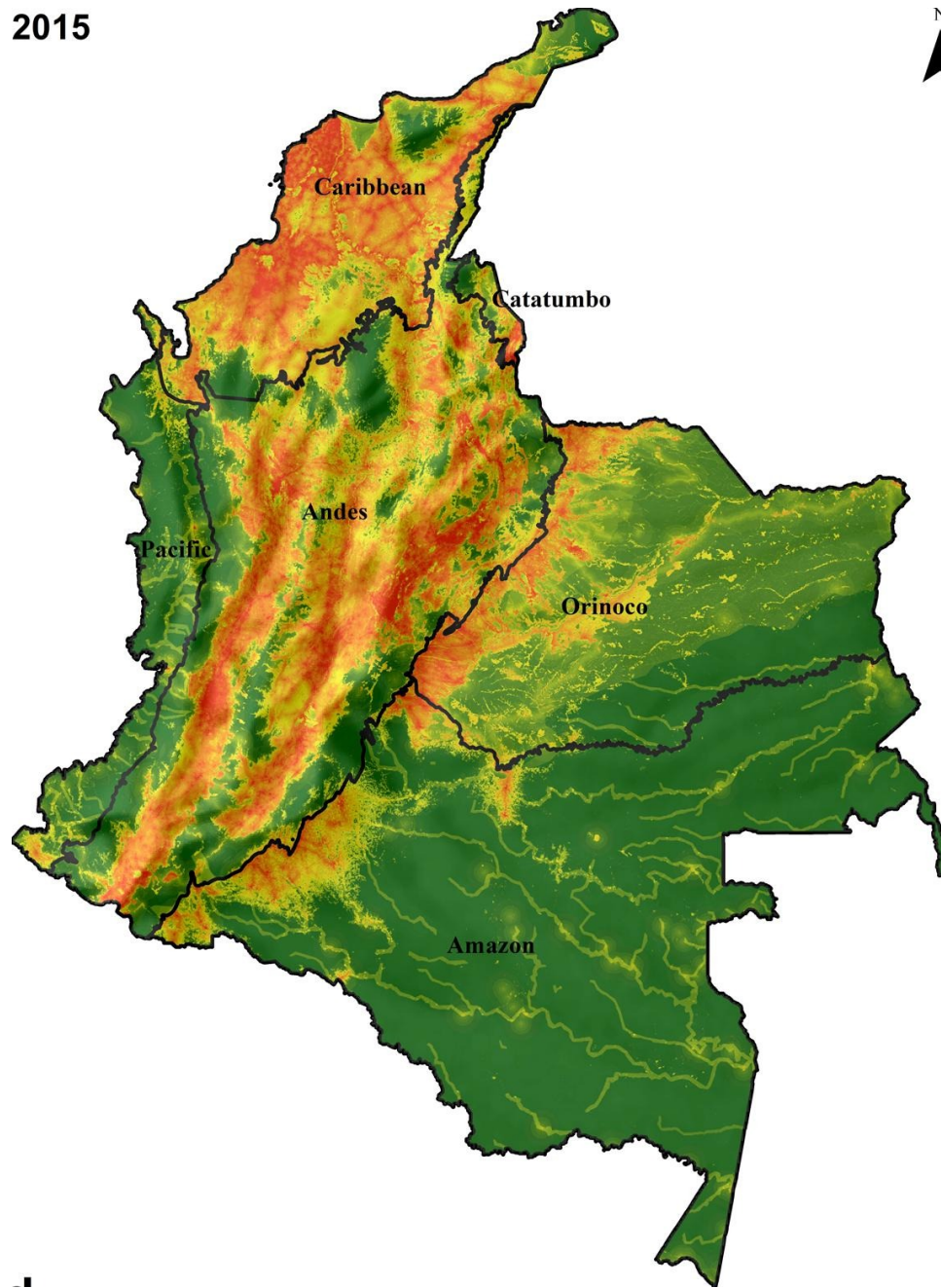
Figure 12: Human footprint. Source: https://www.sciencedirect.com/science/article/pii/S1470160X20305677
