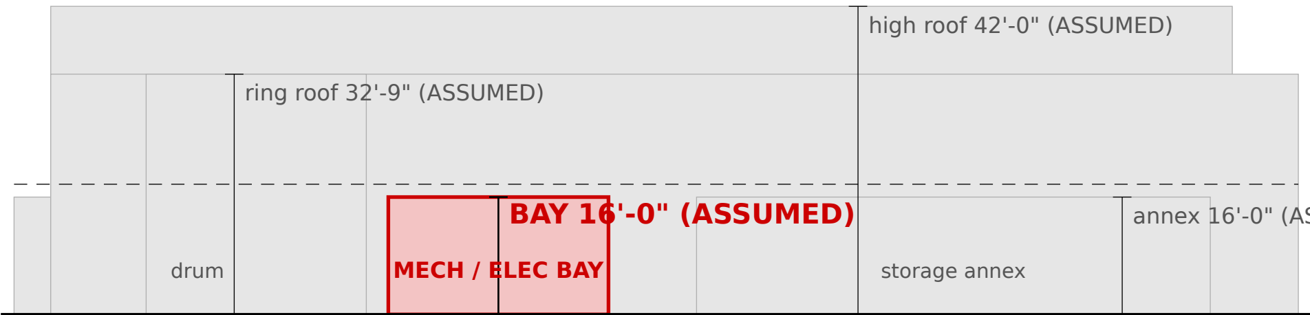
NORTH ELEVATION, CLOSE-UP (east on the left) · not to scale
