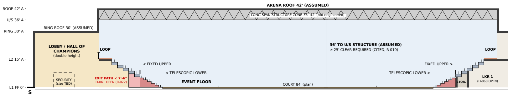
1 SECTION A-A (NORTH-SOUTH) — looking west
