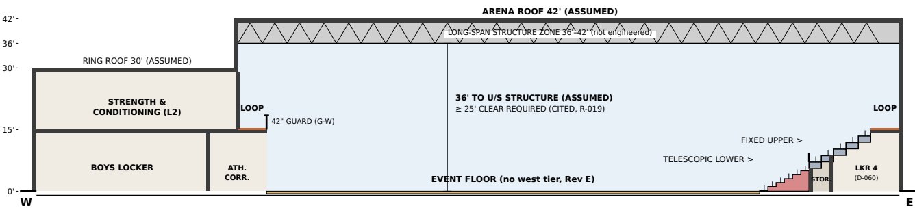
2 SECTION B-B (EAST-WEST) — looking north
