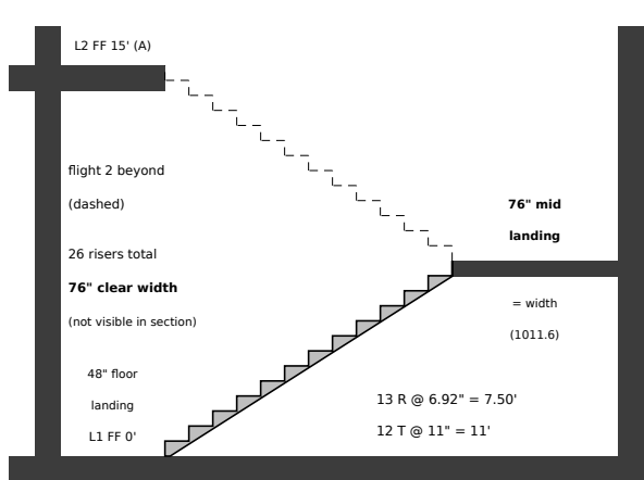
4 TYPICAL EXIT STAIR — 76" CLEAR
