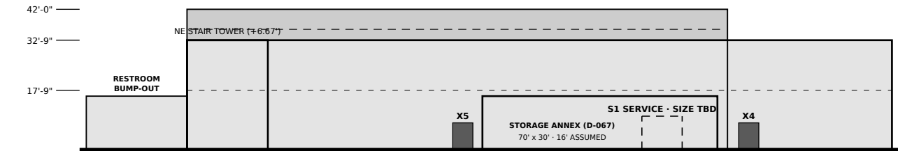
NORTH ELEVATION — 1" = 40'-0" (E ← → W)
