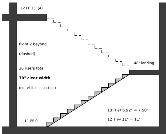
4 TYPICAL EXIT STAIR — 70" CLEAR
