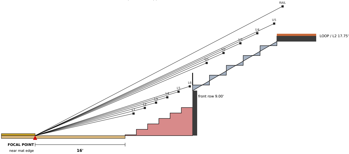
2 AS DRAWN (REV F) — EAST SIDE (seated eyes)
