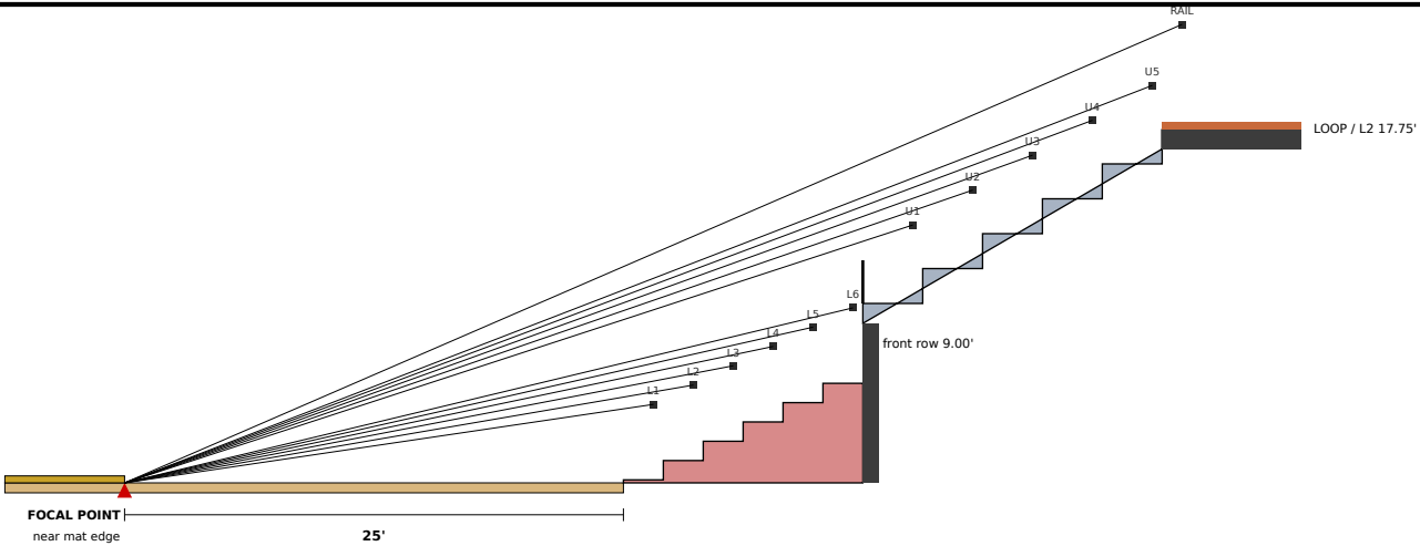
1 AS DRAWN (REV F) — NORTH / SOUTH SIDE (seated eyes)
