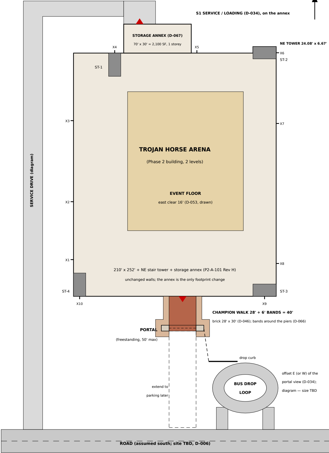
1 SITE PLAN — CAMPUS DIAGRAM (SITE TBD)
