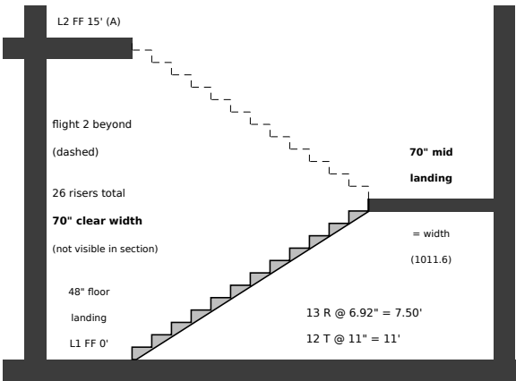
4 TYPICAL EXIT STAIR — 70" CLEAR
