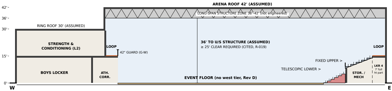
2 SECTION B-B (EAST-WEST) — looking north
