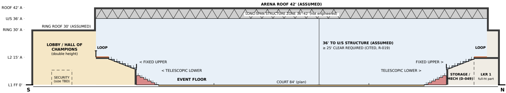
1 SECTION A-A (NORTH-SOUTH) — looking west
