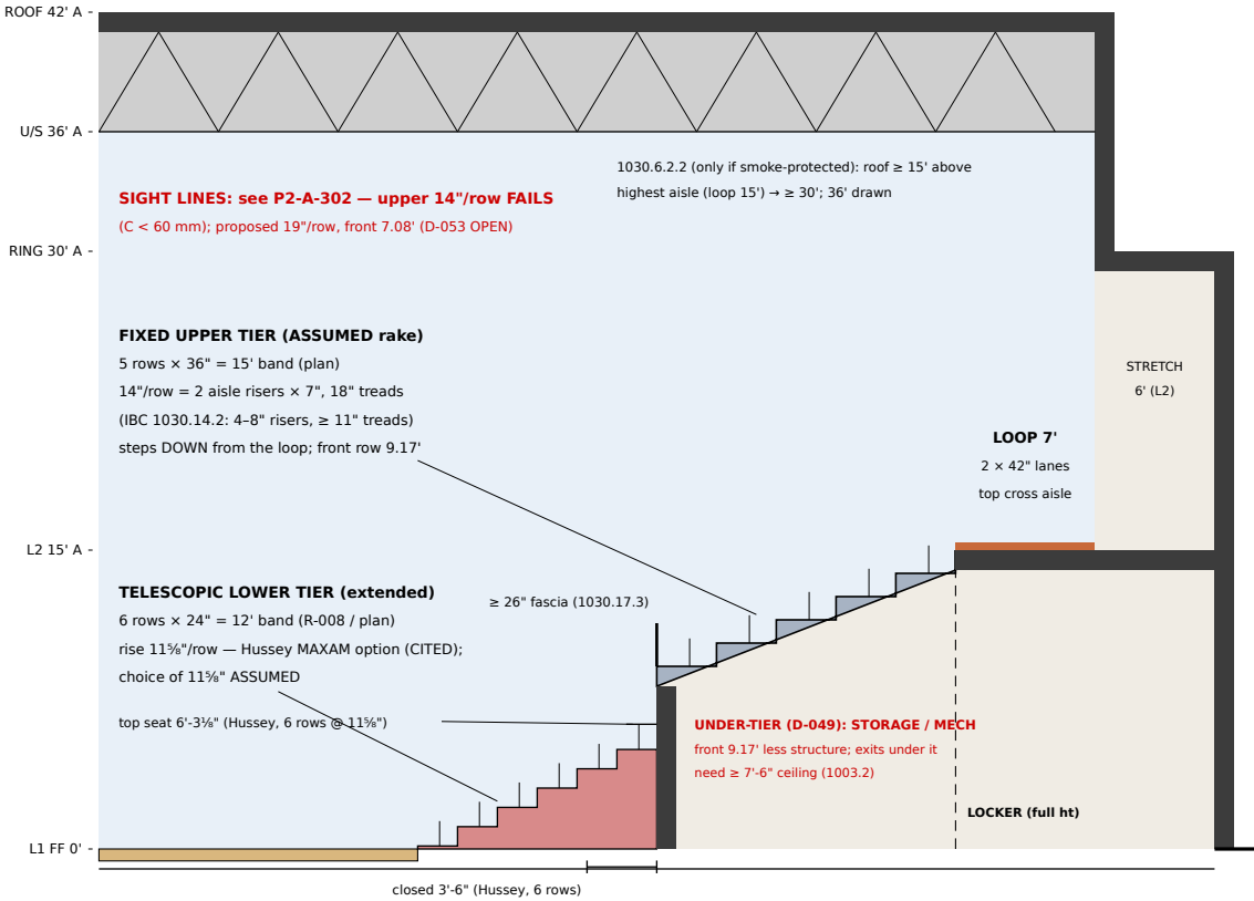
3 NORTH BOWL EDGE (ENLARGED PART OF A-A)
