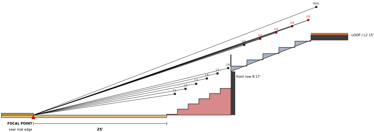
1 AS DRAWN — NORTH / SOUTH SIDE (seated eyes)
