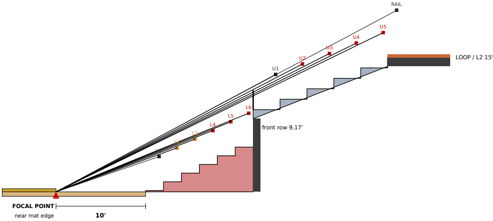
2 AS DRAWN — EAST SIDE (seated eyes)
