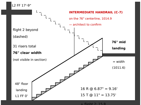
4 TYPICAL EXIT STAIR — 76" CLEAR, 31 R
