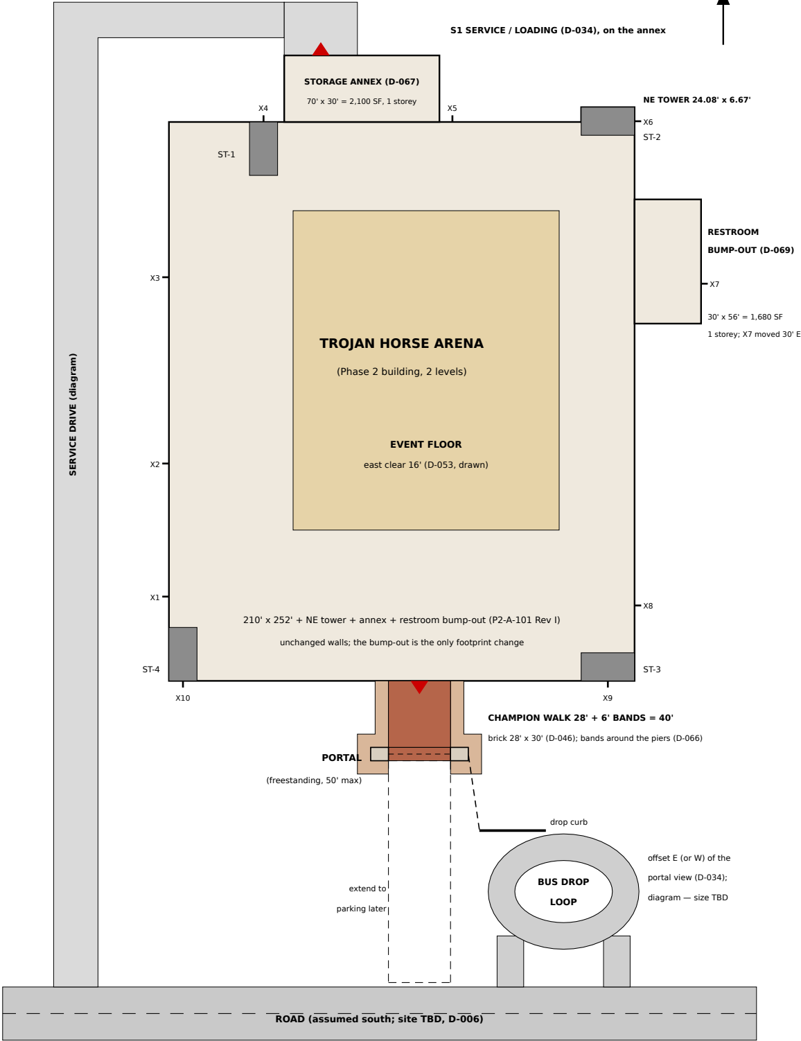
1 SITE PLAN — CAMPUS DIAGRAM (SITE TBD)
