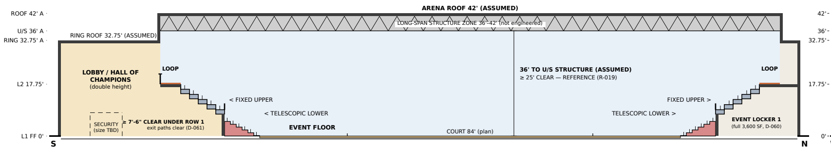
1 SECTION A-A (NORTH-SOUTH) — looking west
