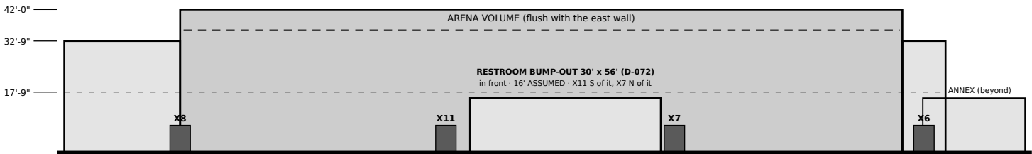
EAST ELEVATION — 1" = 40'-0" (S ← → N)
