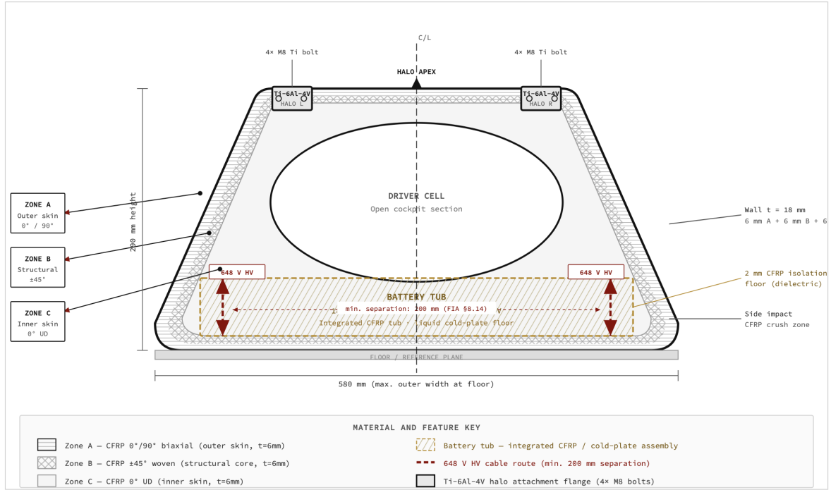
Figure 8: Monocoque Cross-Section Diagram illustrating CFRP Ply Orientation Zones, Battery Tub Integration, 648V Cable Routing limits, and Ti-6Al-4V Halo Attachment Points.
