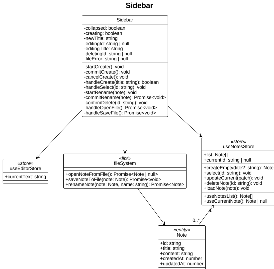
Figura 5: Diagramma UML 3.3.2-1 - Sidebar
