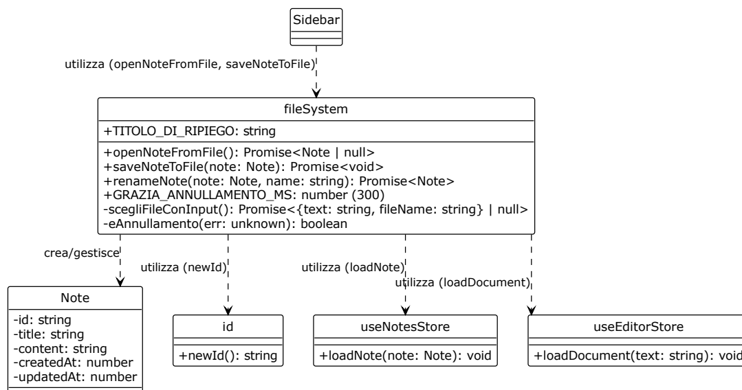
Figura 24: Diagramma UML 4.4.1-3 - openNoteFromFile
