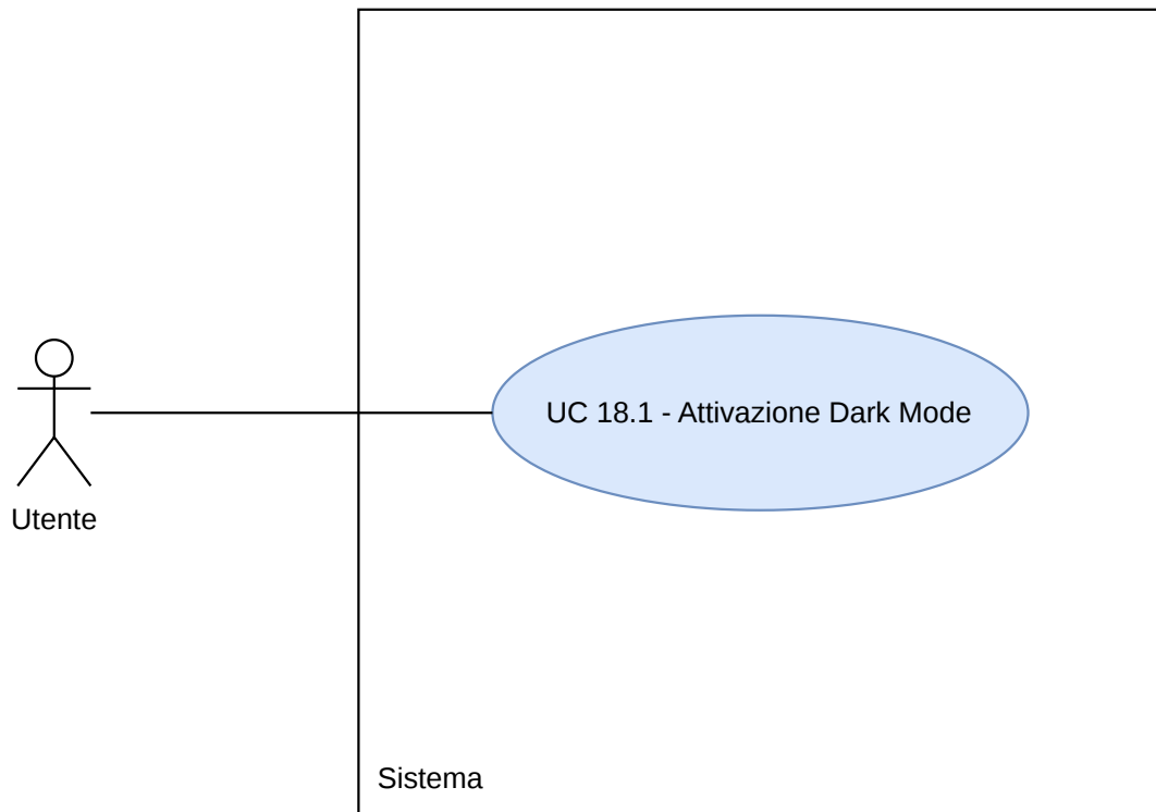
Figura 65: Diagramma UC18.1
