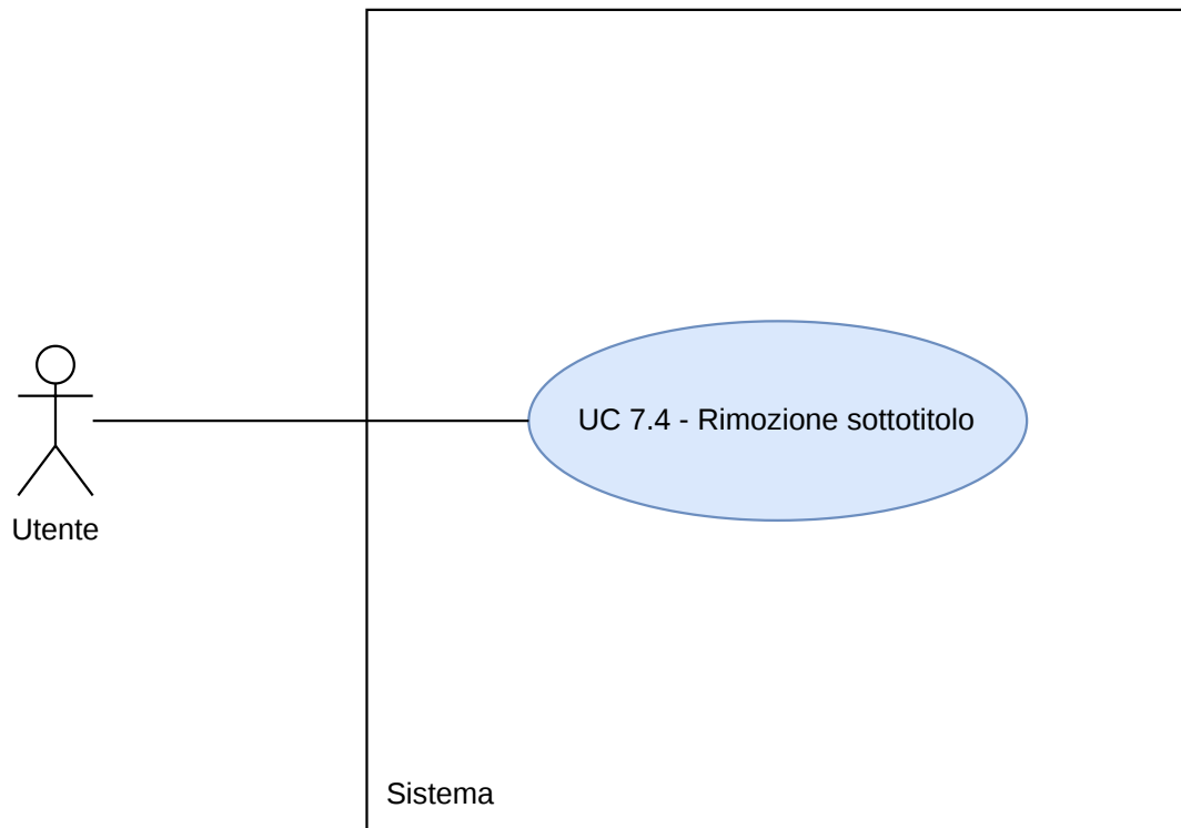
Figura 26: Diagramma UC7.4
