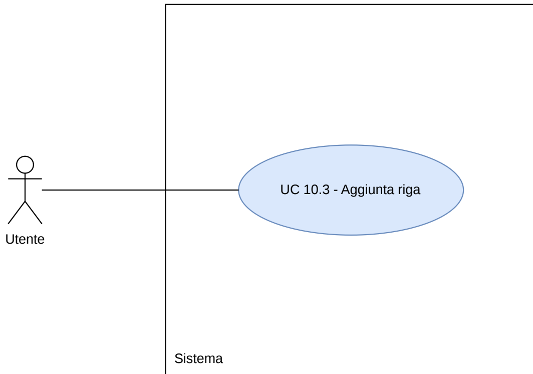
Figura 36: Diagramma UC10.3
