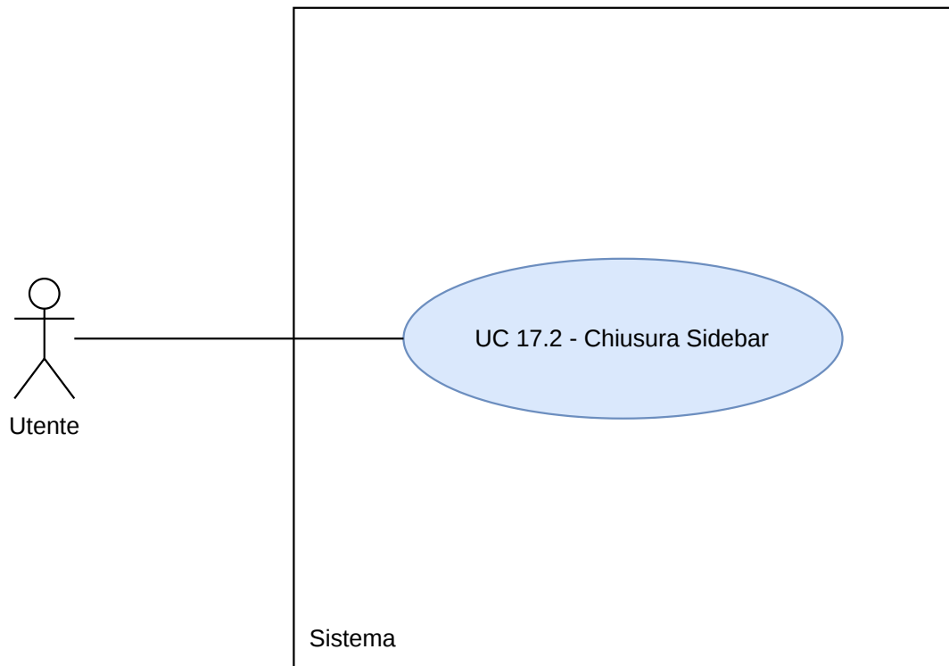
Figura 62: Diagramma UC17.2
