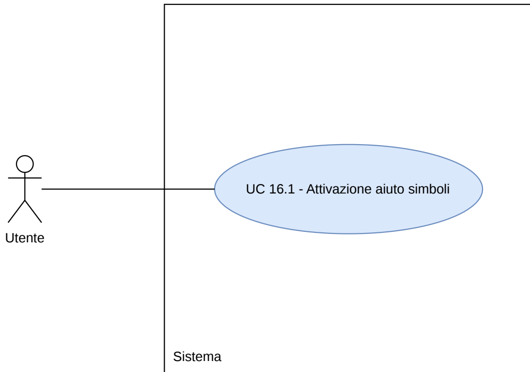
Figura 58: Diagramma UC16.1
