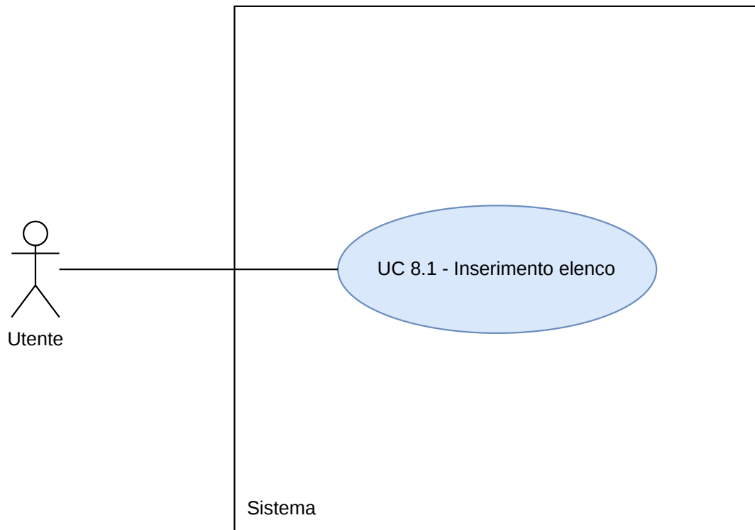
Figura 28: Diagramma UC8.1
