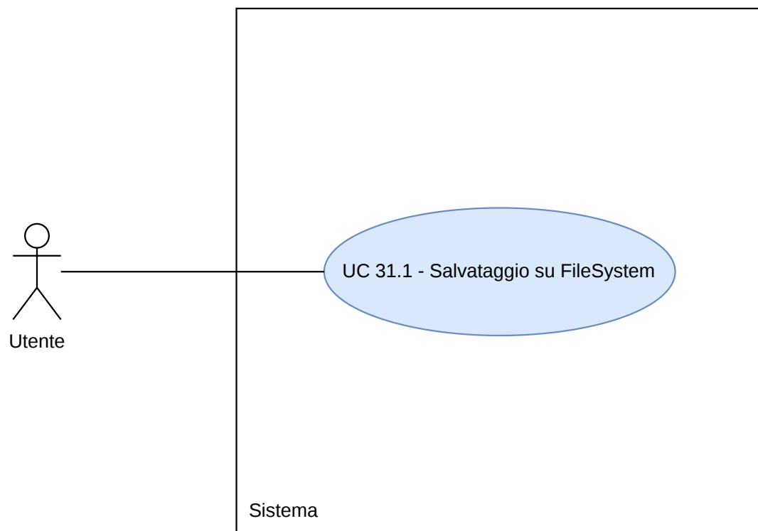
Figura 120: Diagramma UC31.1
