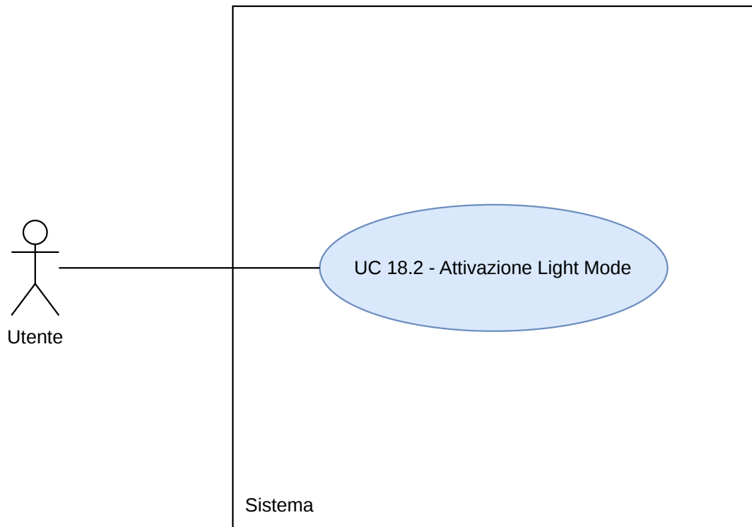
Figura 66: Diagramma UC18.2
