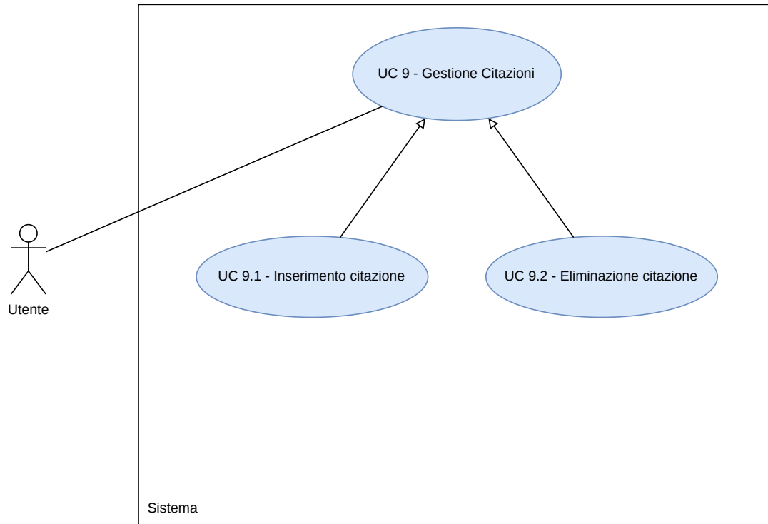
Figura 30: Diagramma UC9
