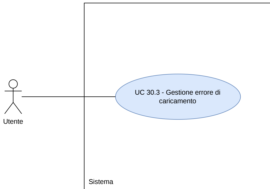
Figura 118: Diagramma UC30.3
