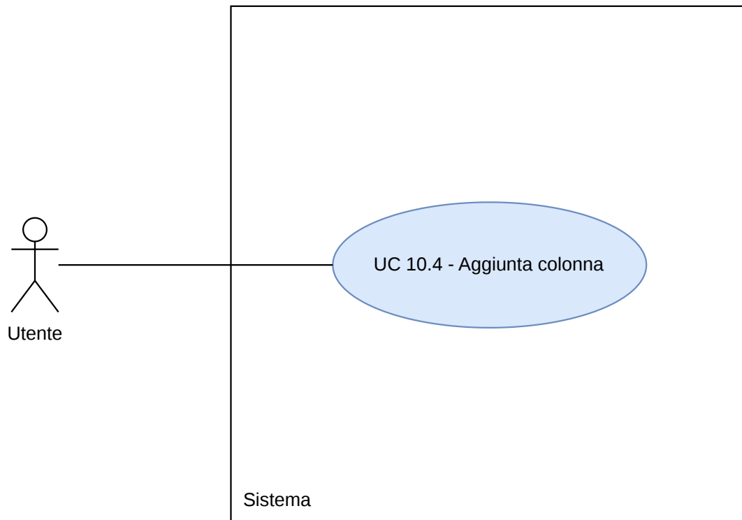
Figura 37: Diagramma UC10.4
