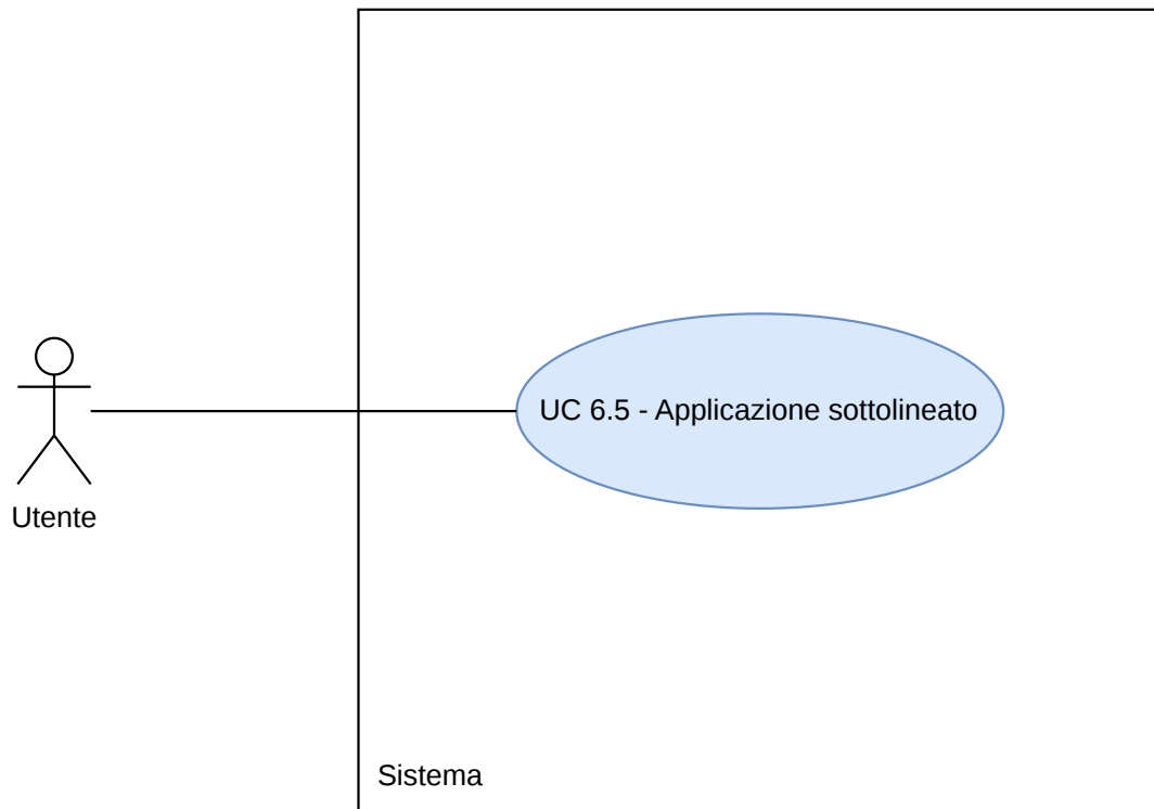
Figura 16: Diagramma UC6.5
