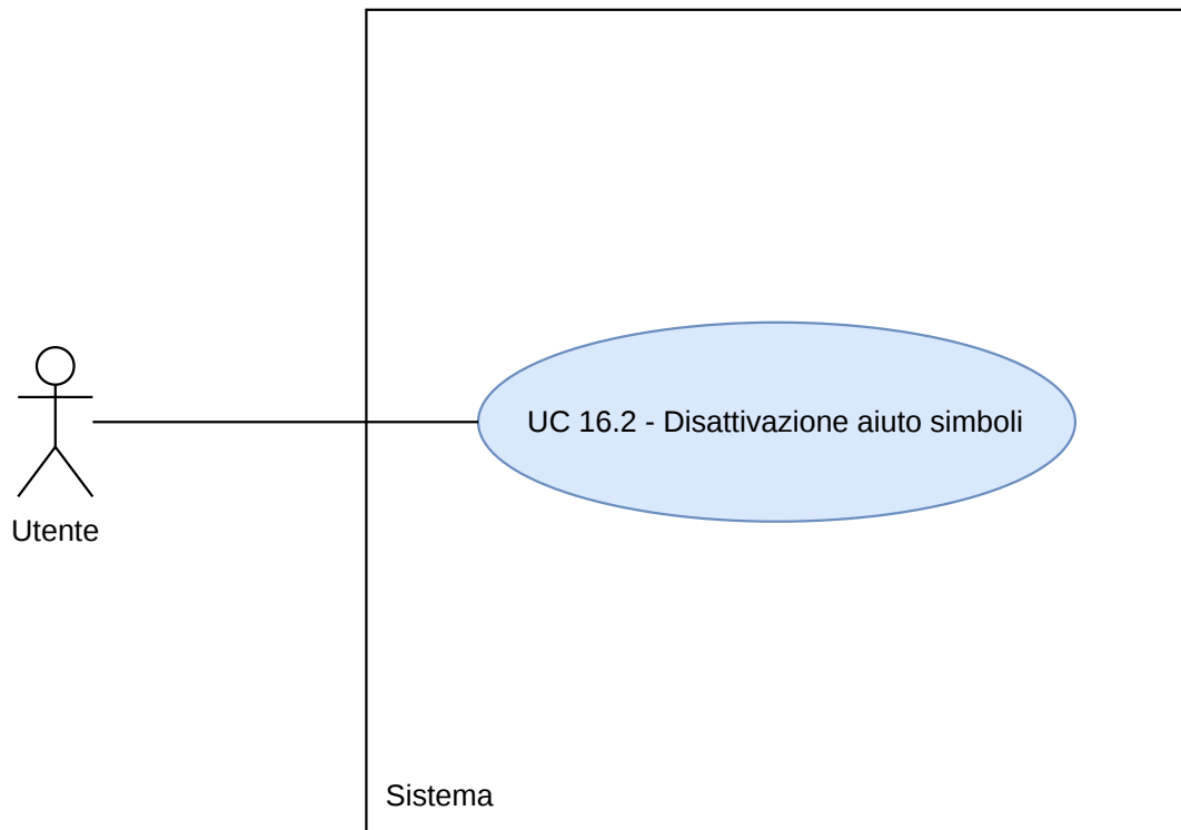
Figura 59: Diagramma UC16.2
