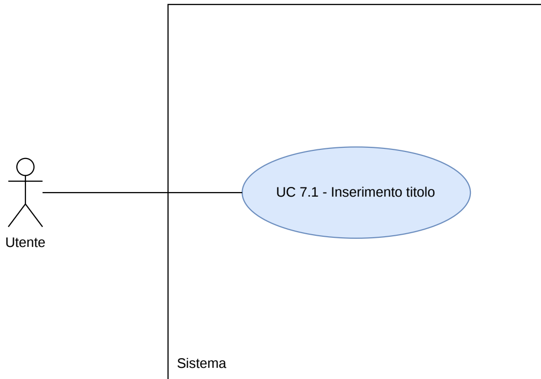
Figura 23: Diagramma UC7.1
