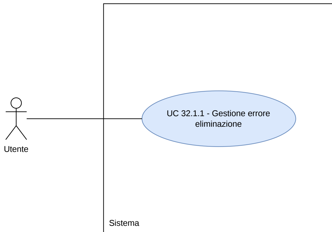
Figura 125: Diagramma UC32.1.1
