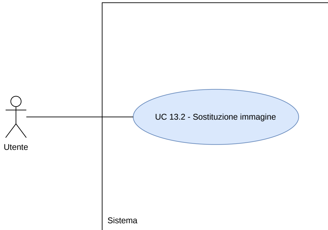
Figura 49: Diagramma UC13.2
