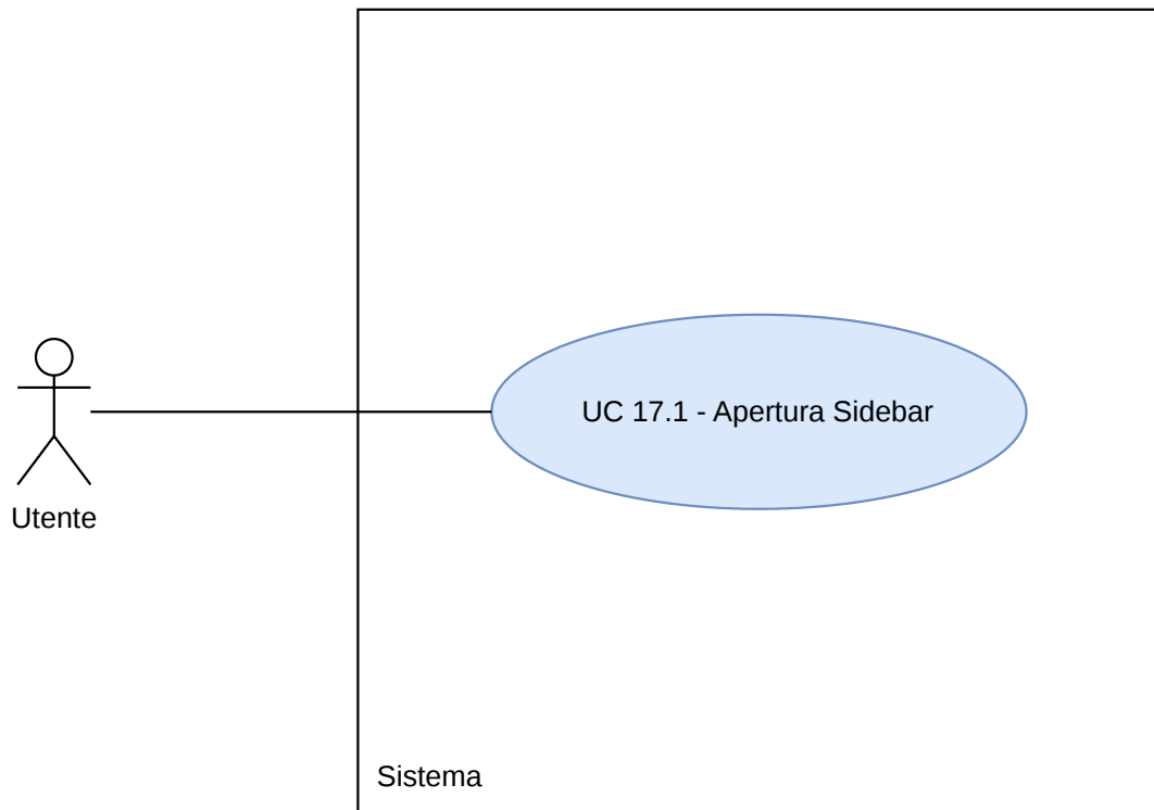
Figura 61: Diagramma UC17.1
