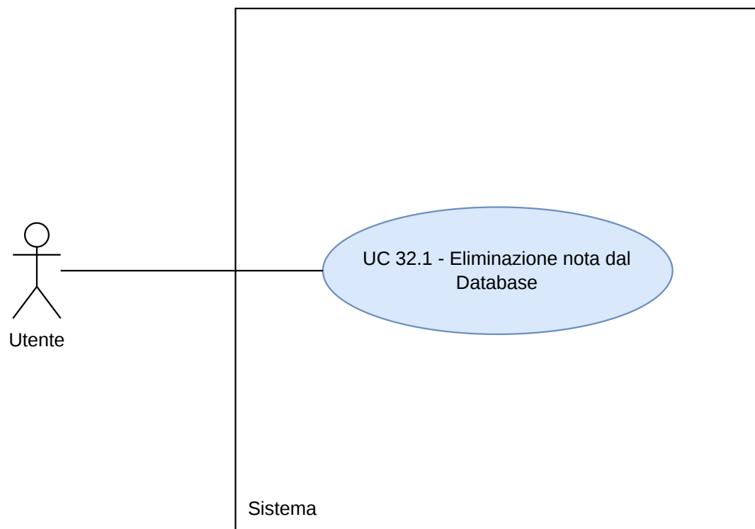
Figura 124: Diagramma UC32.1
