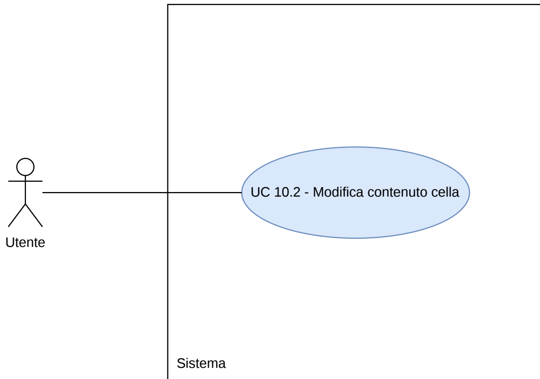
Figura 35: Diagramma UC10.2
