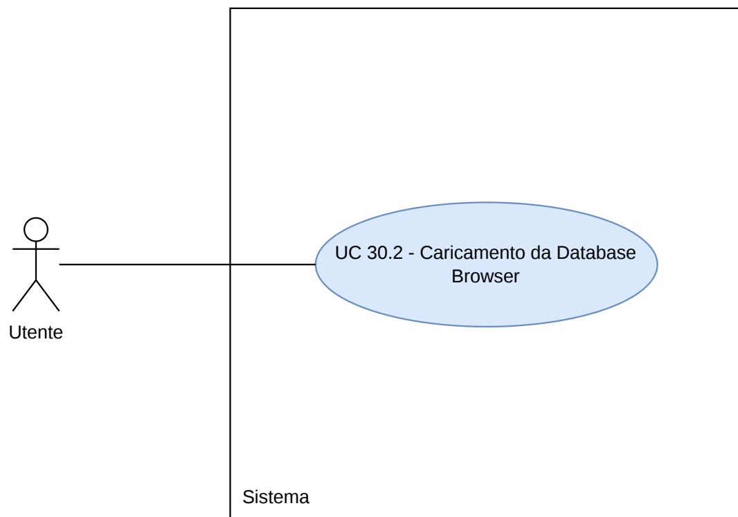
Figura 117: Diagramma UC30.2
