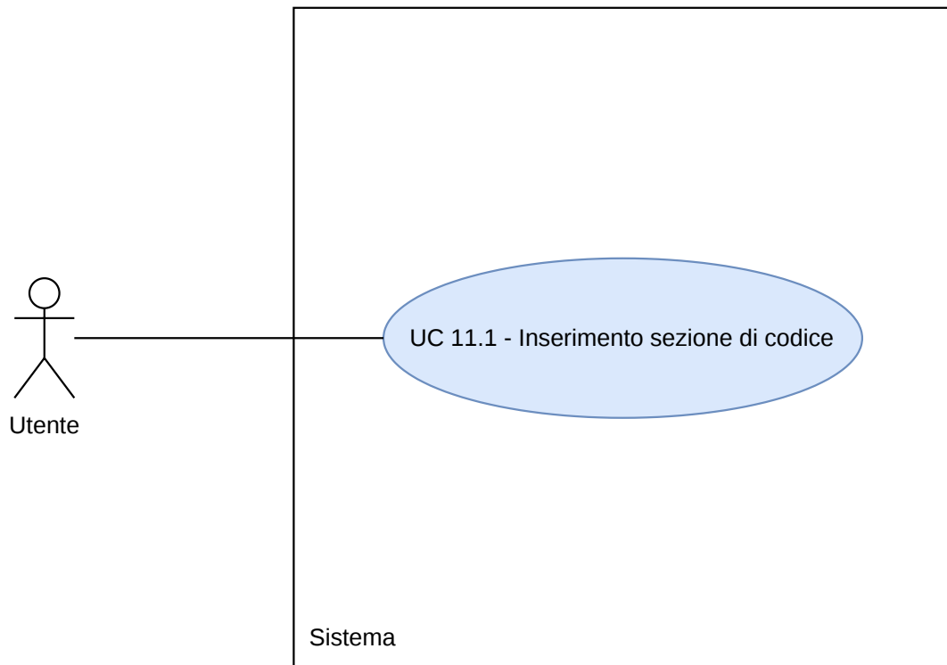
Figura 42: Diagramma UC11.1
