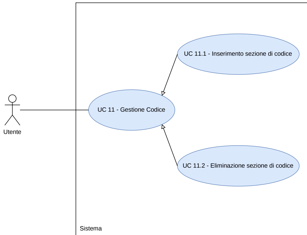
Figura 41: Diagramma UC11
