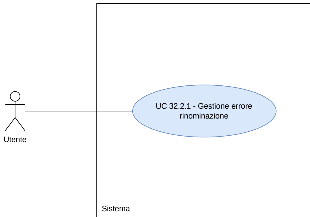
Figura 127: Diagramma UC32.2.1
