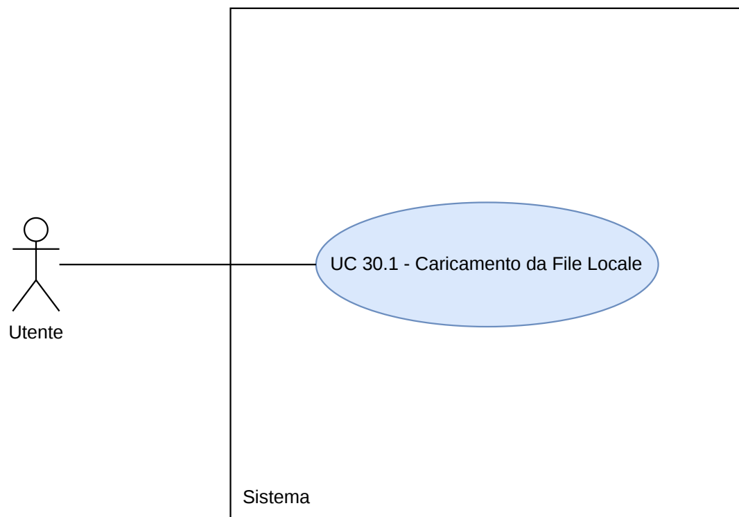
Figura 116: Diagramma UC30.1
