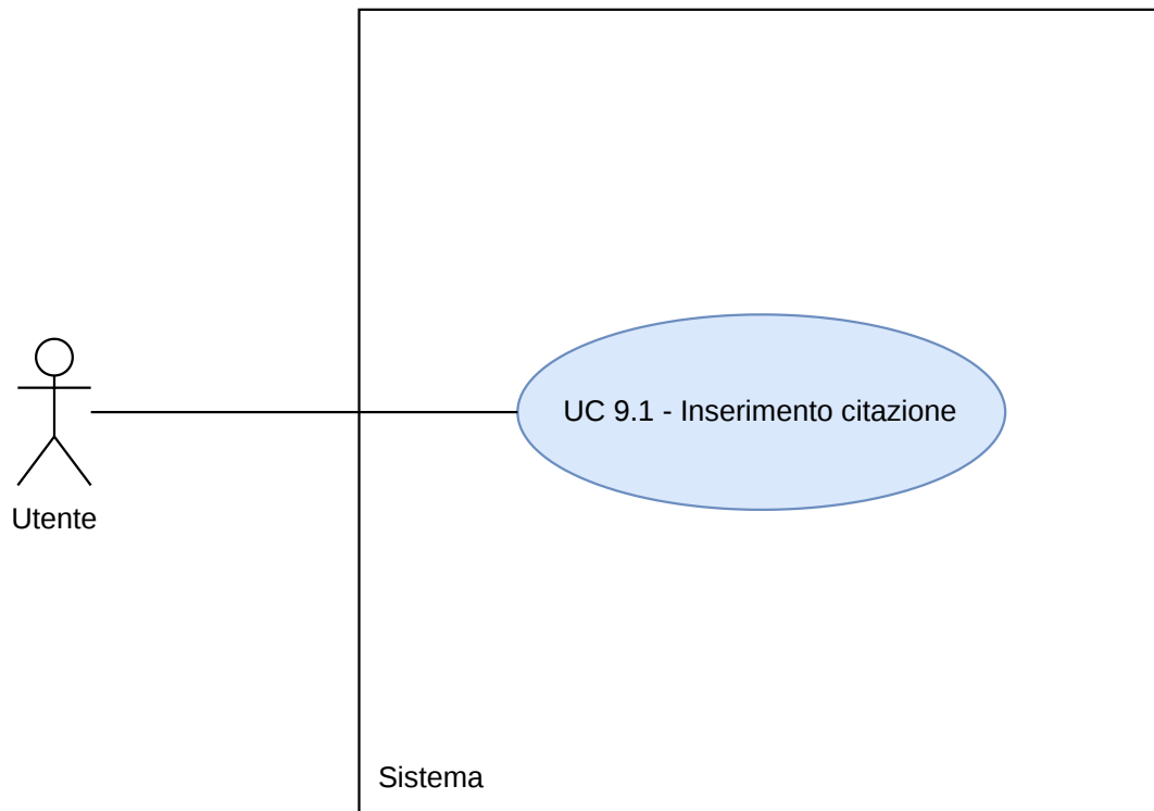
Figura 31: Diagramma UC9.1
