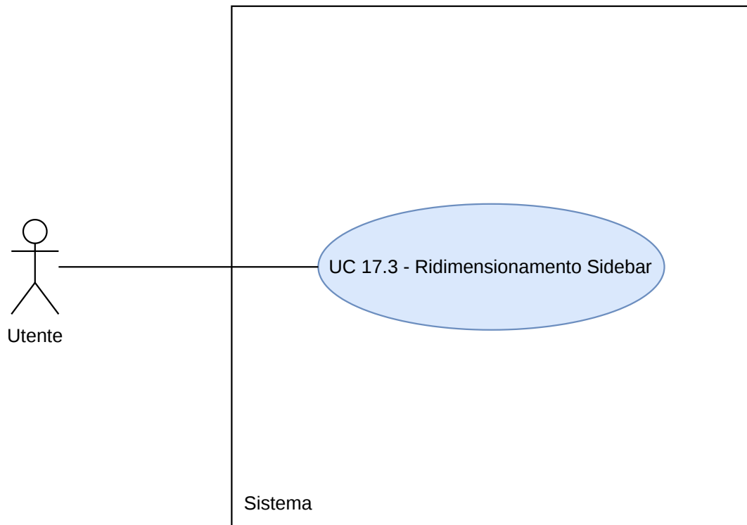
Figura 63: Diagramma UC17.3
