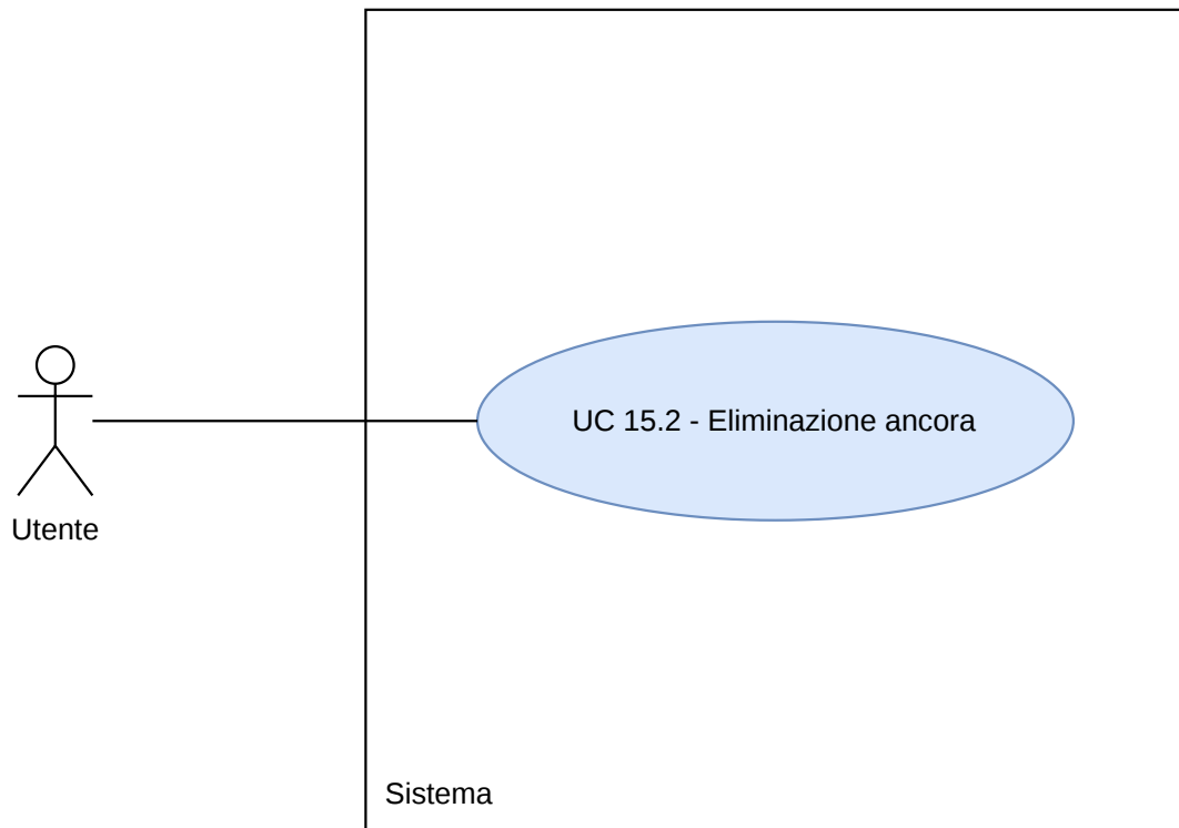
Figura 56: Diagramma UC15.2
