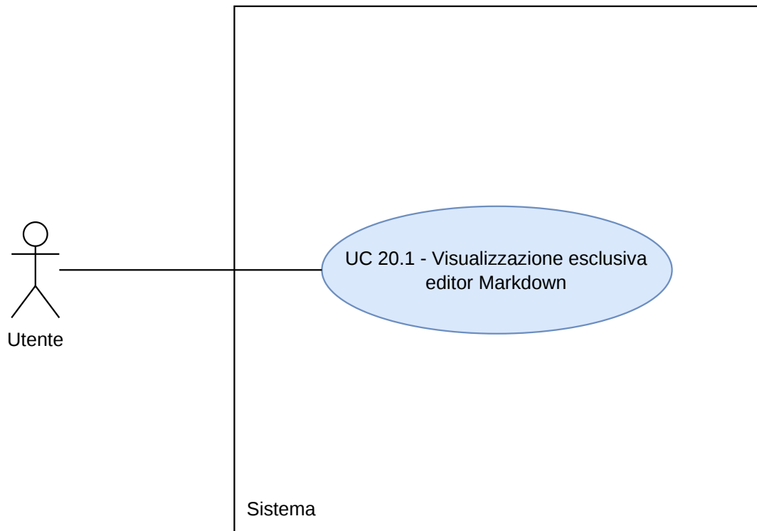
Figura 71: Diagramma UC20.1
