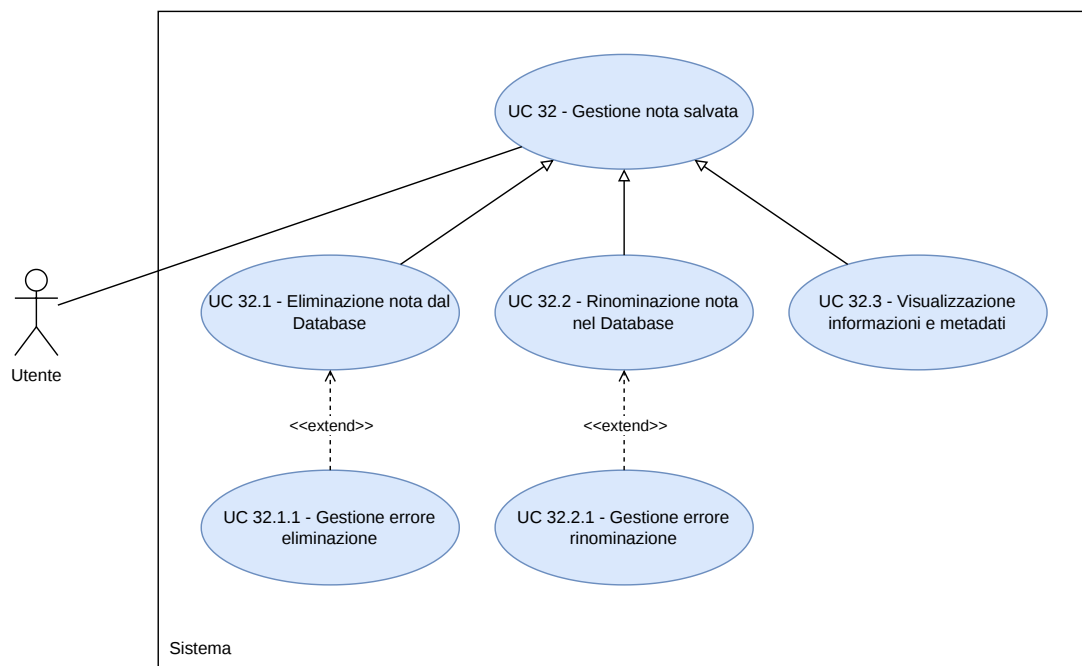
Figura 123: Diagramma UC32
