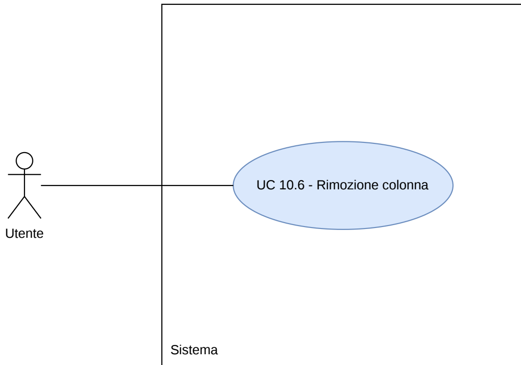
Figura 39: Diagramma UC10.6
