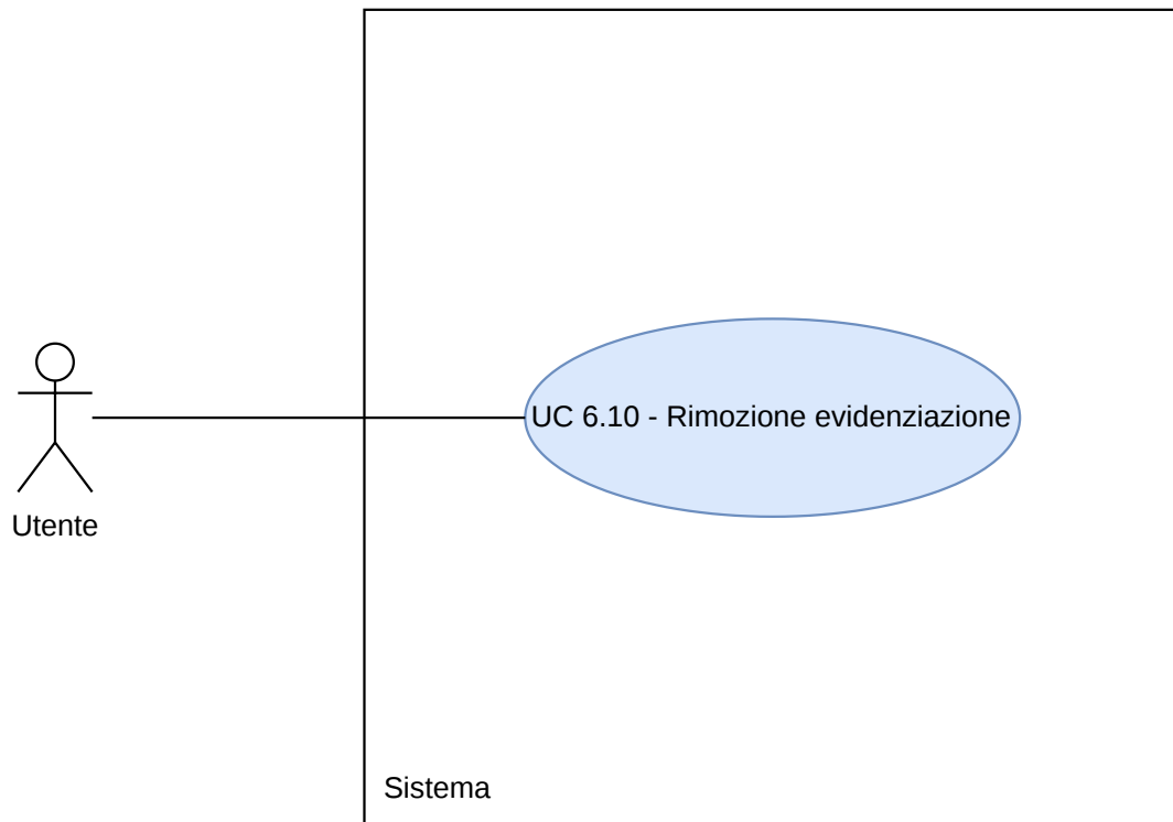
Figura 21: Diagramma UC6.10
