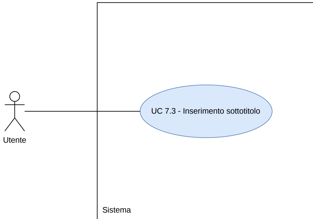
Figura 25: Diagramma UC7.3
