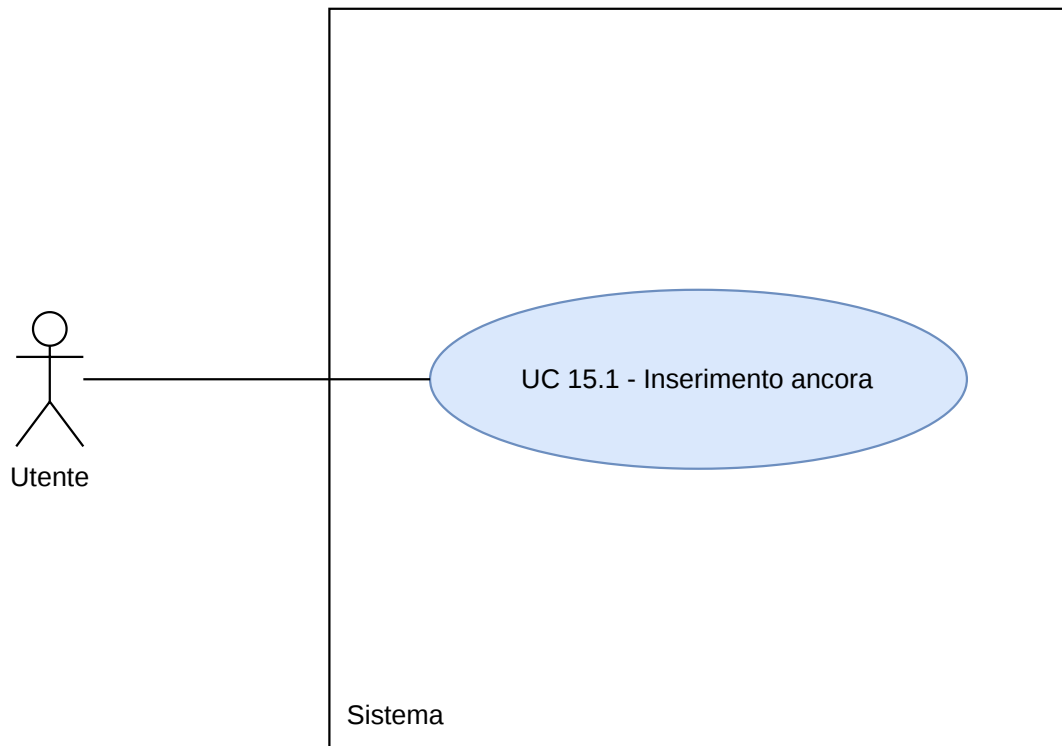
Figura 55: Diagramma UC15.1
