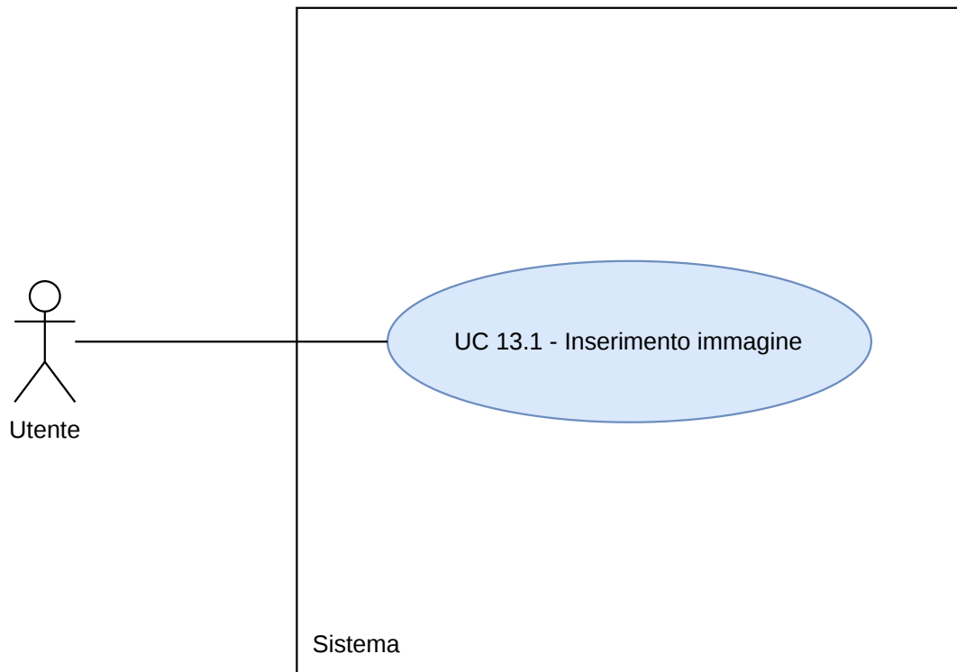
Figura 48: Diagramma UC13.1
