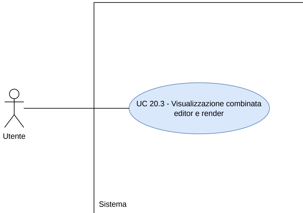
Figura 73: Diagramma UC20.3
