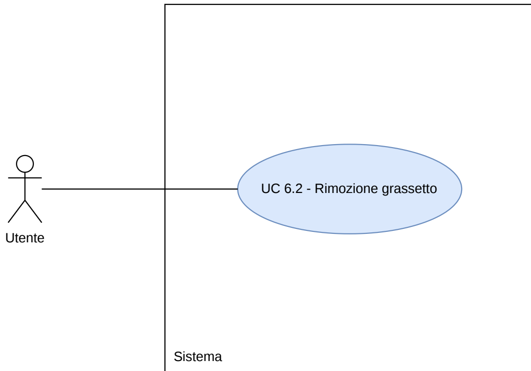
Figura 13: Diagramma UC6.2
