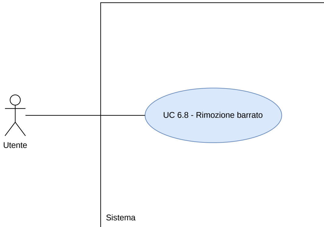
Figura 19: Diagramma UC6.8
