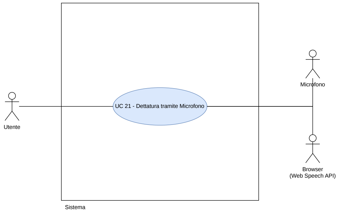
Figura 74: Diagramma UC21
