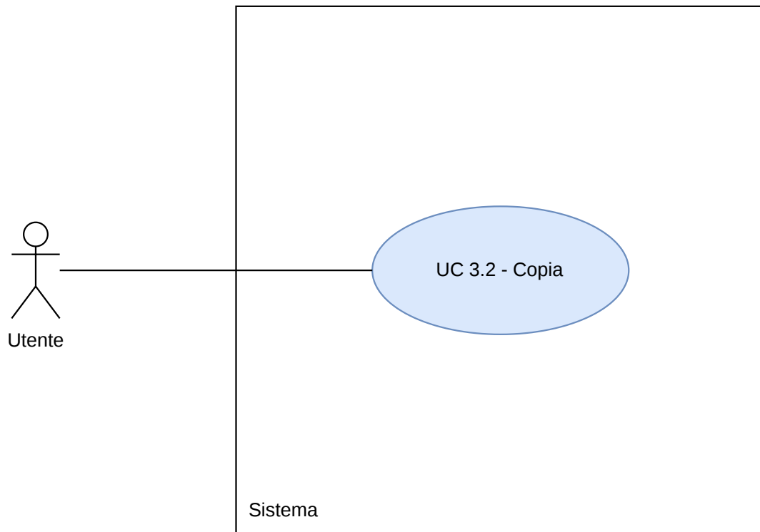
Figura 7: Diagramma UC3.2
