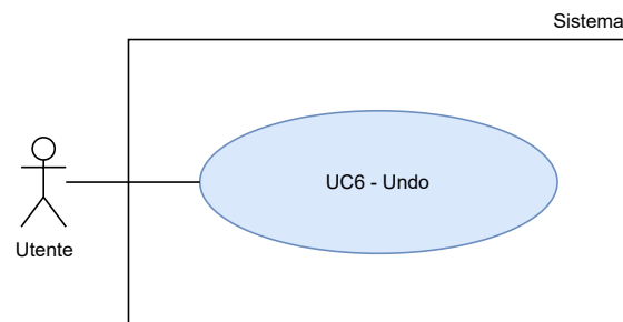
Figura 7: UC6 - Undo
