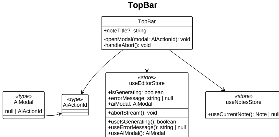
Figura 6: Diagramma UML 3.3.2-2 - TopBar
