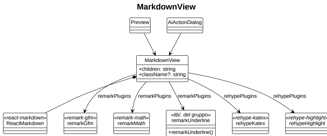
Figura 8: Diagramma UML 3.3.2-4 - MarkdownView
