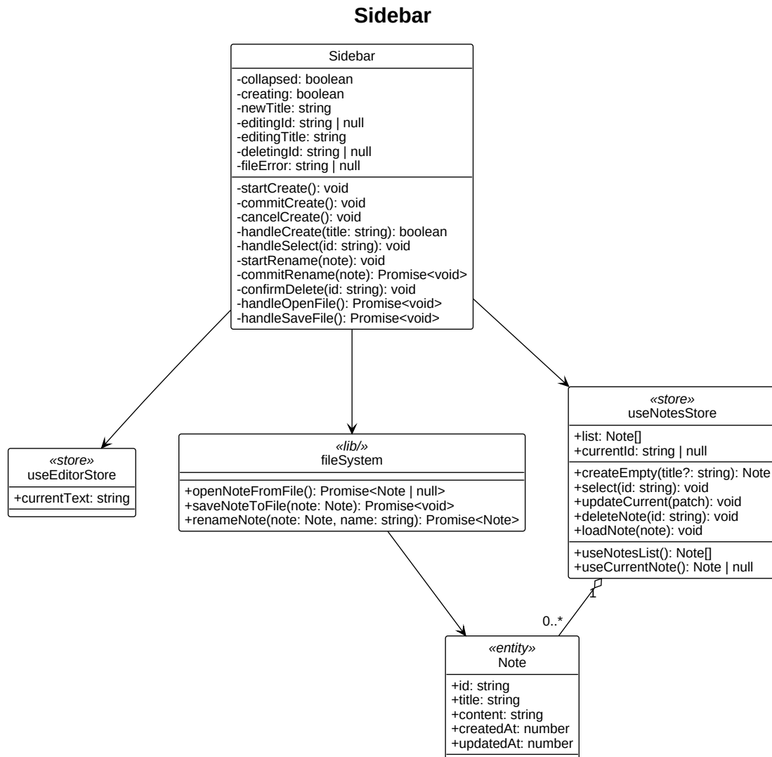
Figura 5: Diagramma UML 3.3.2-1 - Sidebar
