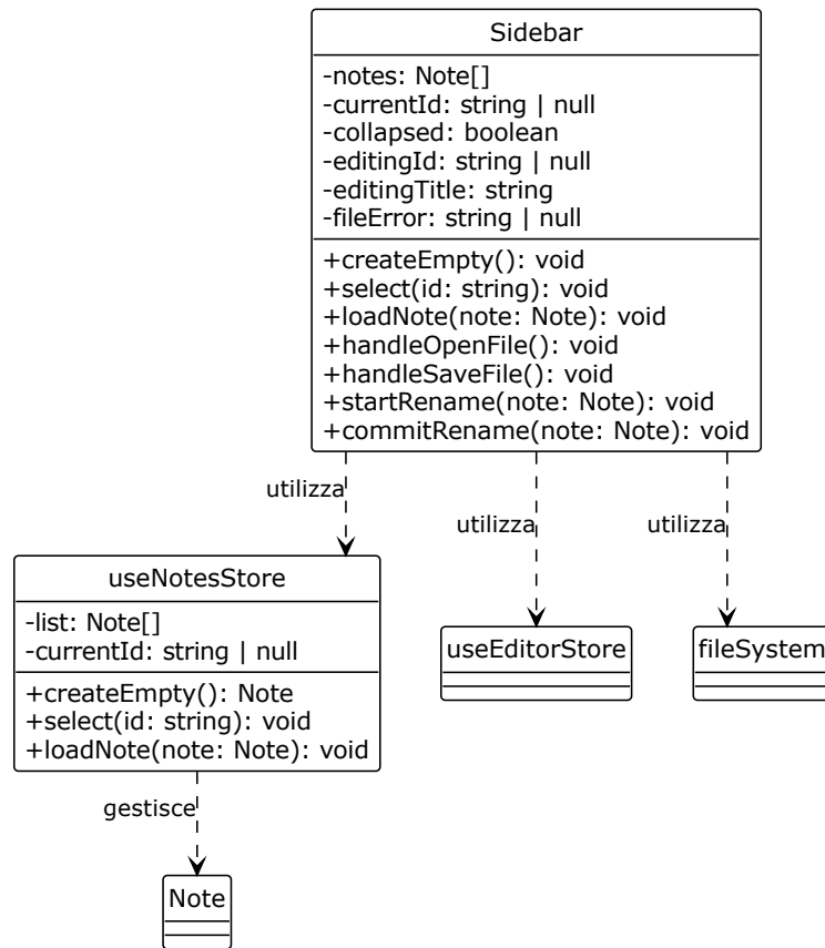
Figura 5: Diagramma UML 3.3.2-1 - Sidebar
