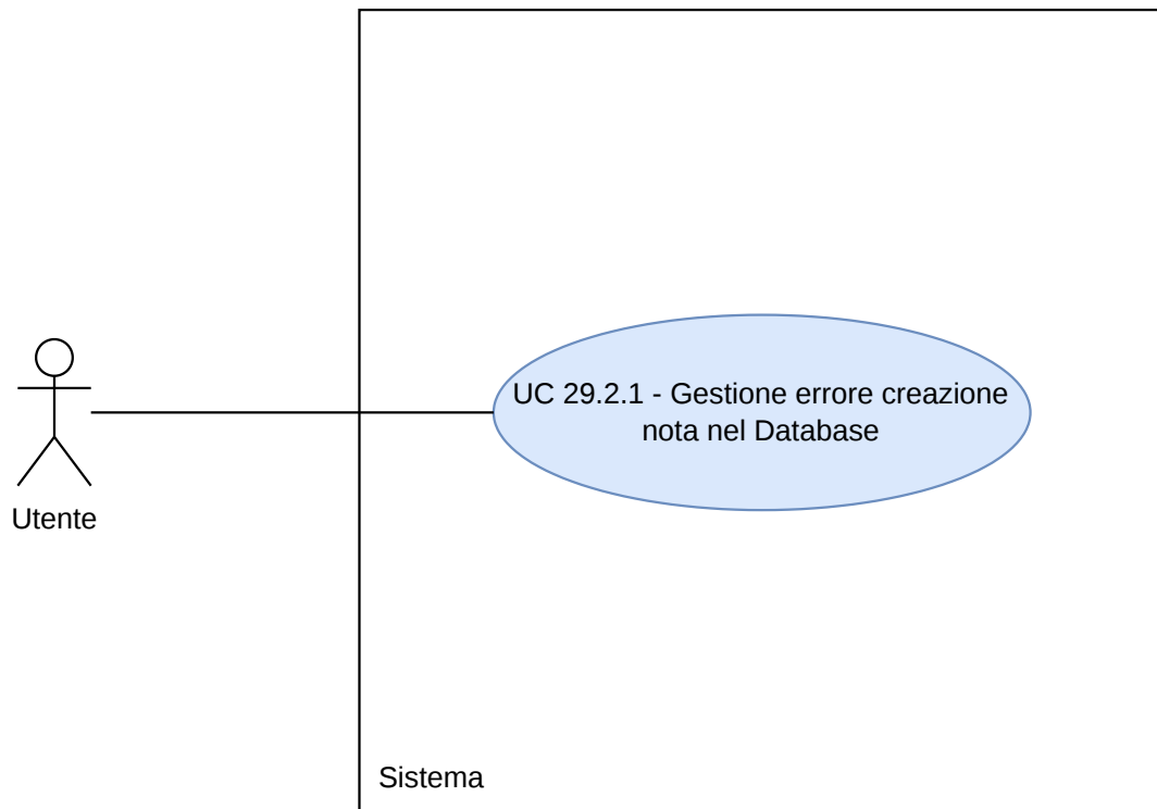
Figura 115: Diagramma UC29.2.1
