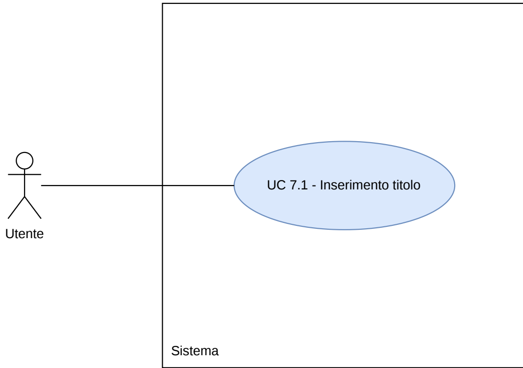
Figura 24: Diagramma UC7.1
