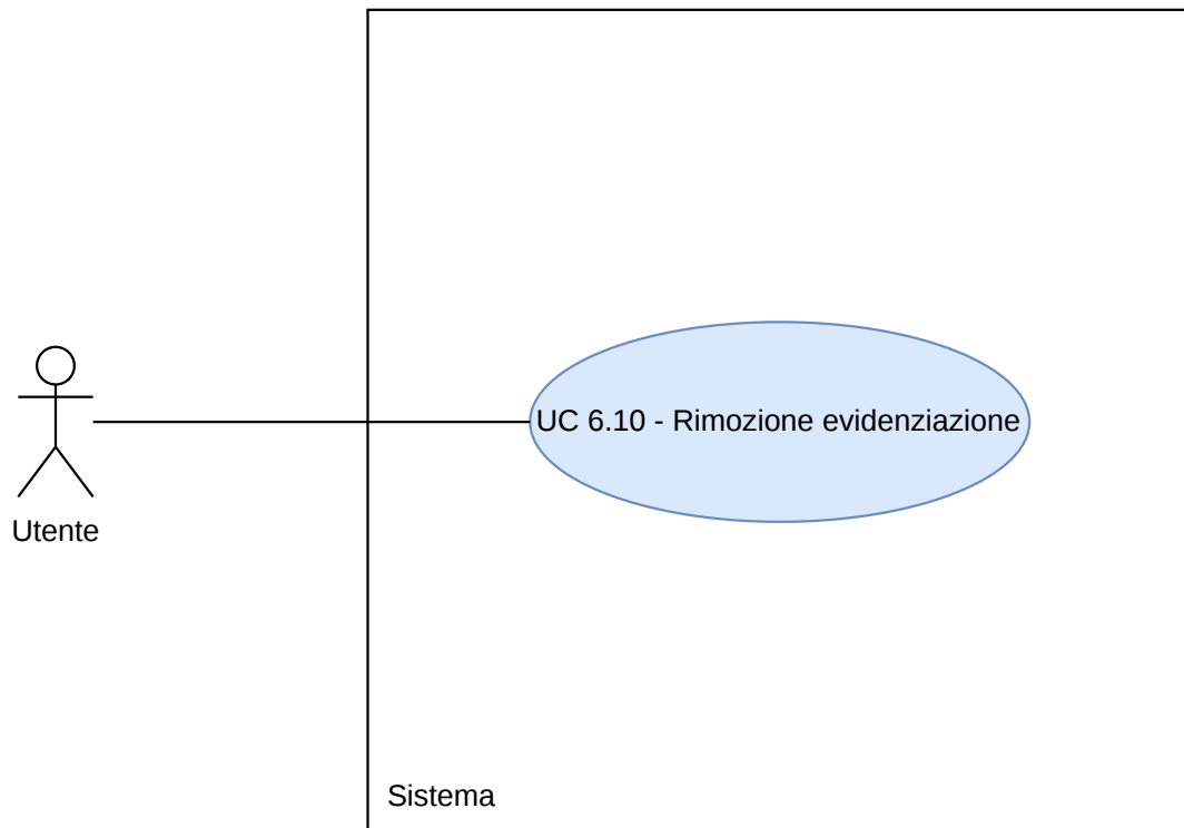
Figura 22: Diagramma UC6.10
