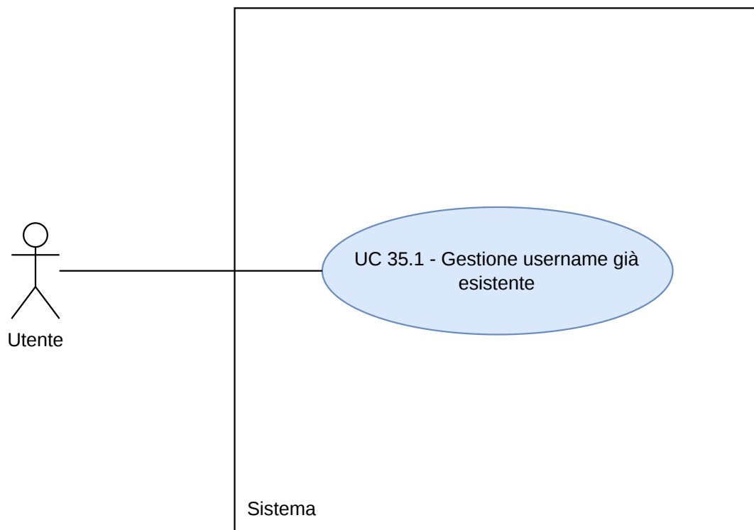
Figura 140: Diagramma UC35.1
