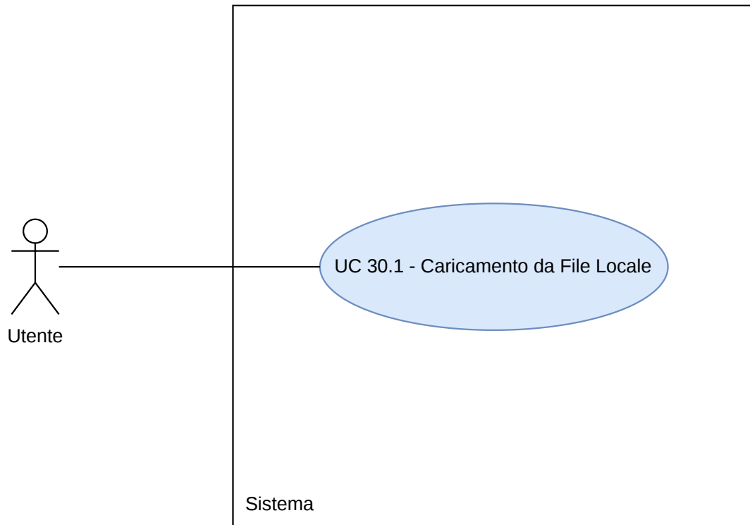
Figura 117: Diagramma UC30.1
