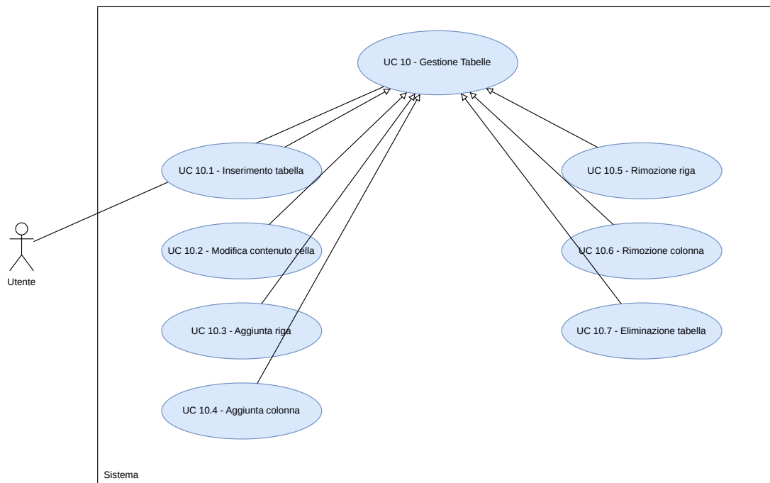
Figura 34: Diagramma UC10
