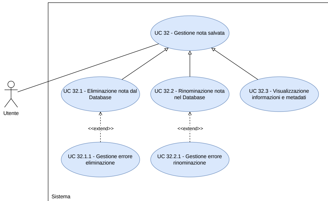
Figura 124: Diagramma UC32
