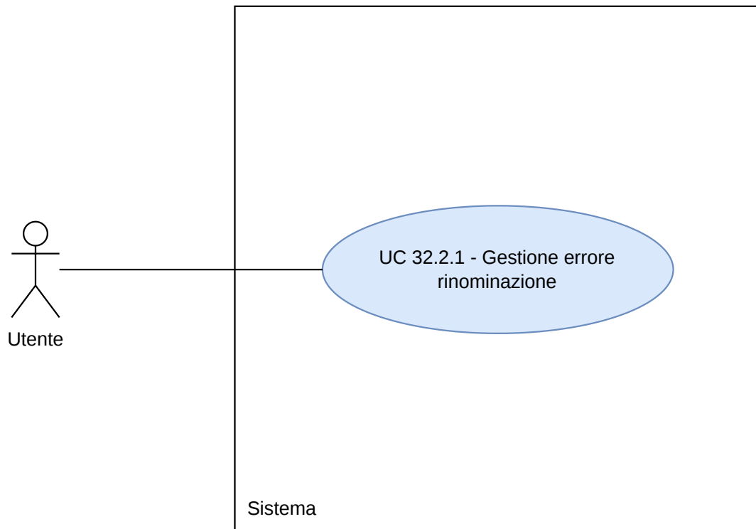
Figura 128: Diagramma UC32.2.1
