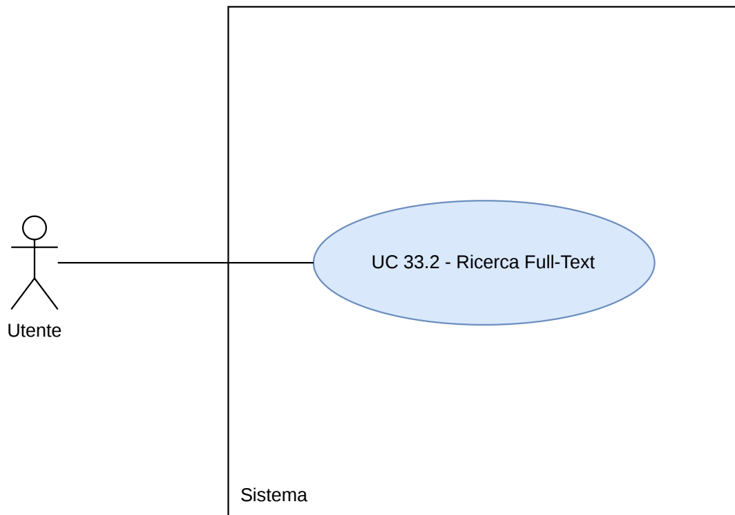
Figura 132: Diagramma UC33.2
