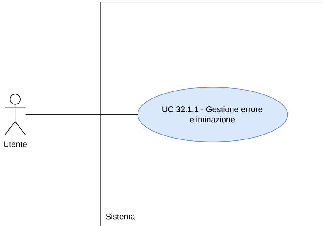
Figura 126: Diagramma UC32.1.1
