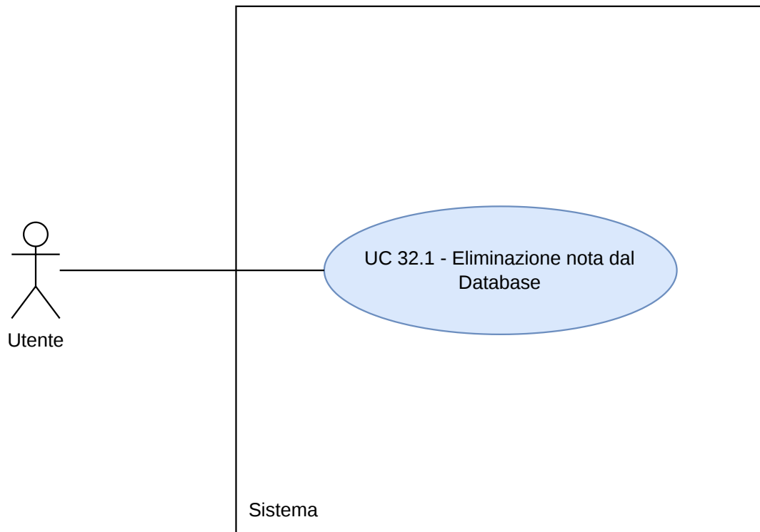
Figura 125: Diagramma UC32.1
