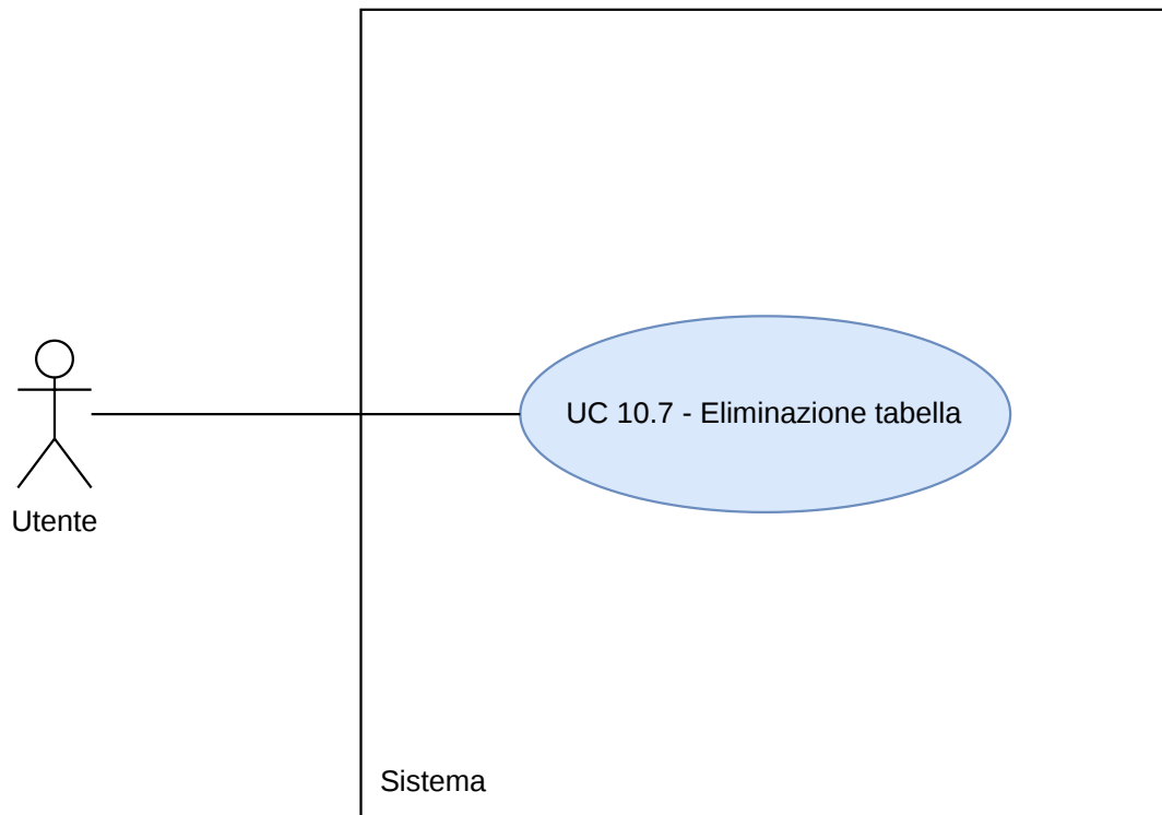
Figura 41: Diagramma UC10.7
