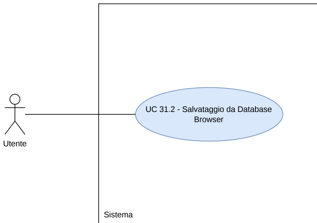
Figura 122: Diagramma UC31.2
