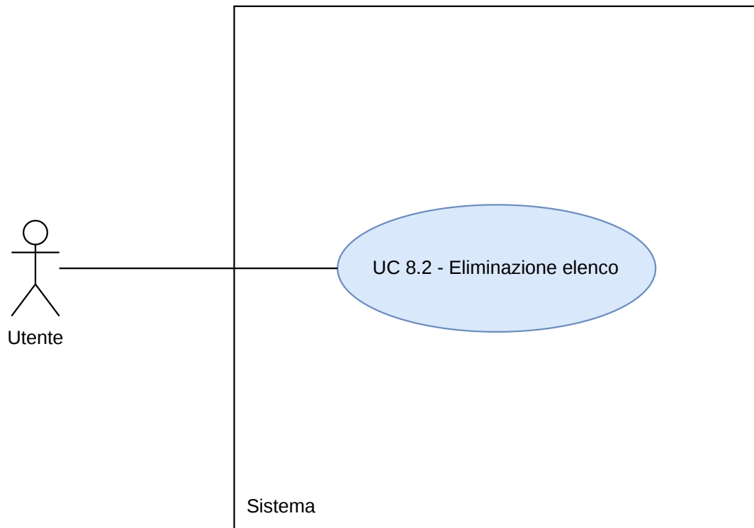
Figura 30: Diagramma UC8.2
