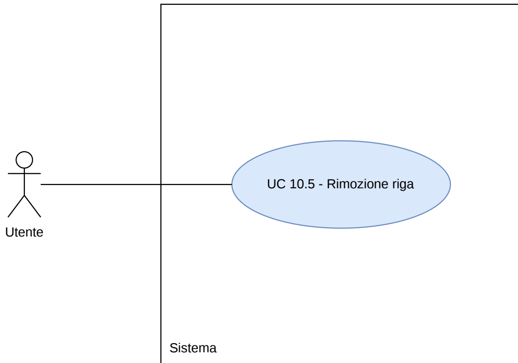
Figura 39: Diagramma UC10.5
