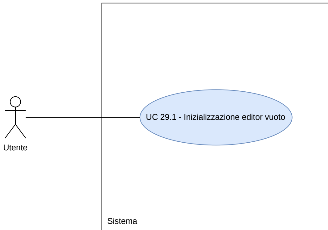
Figura 113: Diagramma UC29.1
