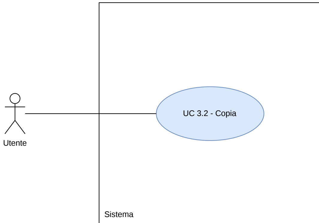
Figura 8: Diagramma UC3.2
