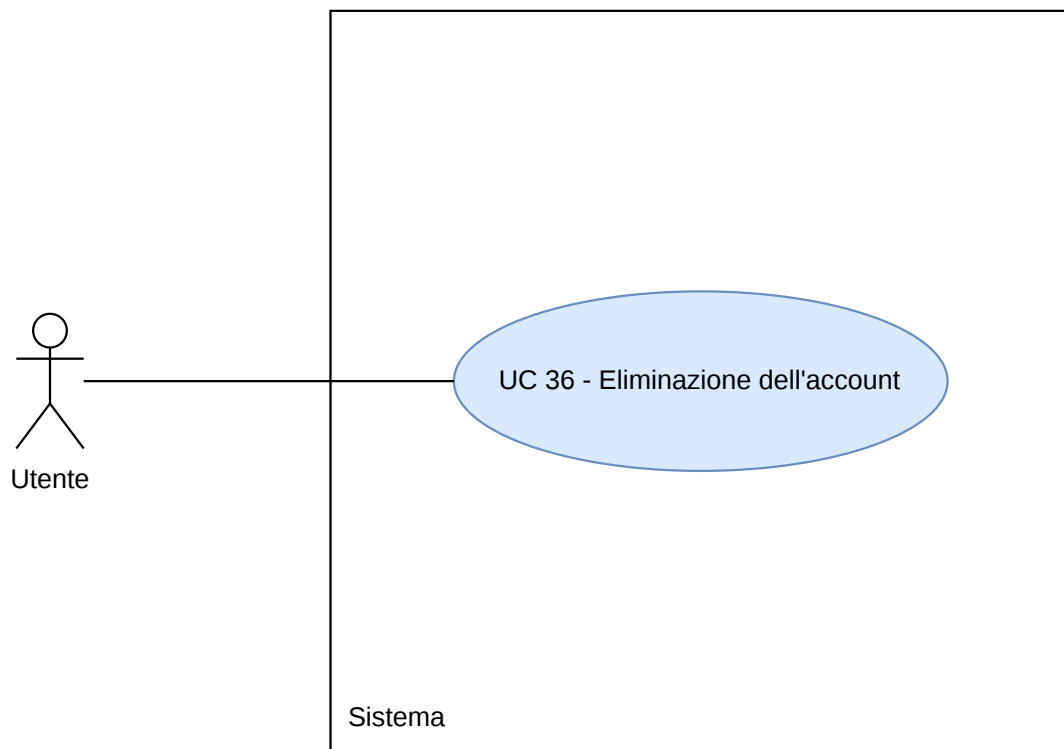
Figura 141: Diagramma UC36
