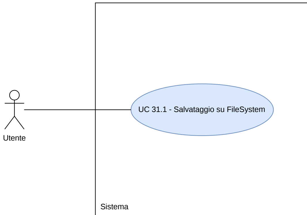
Figura 121: Diagramma UC31.1
