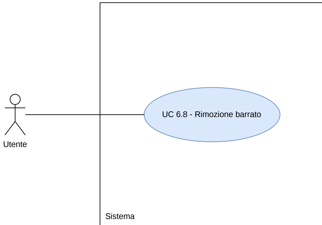
Figura 20: Diagramma UC6.8
