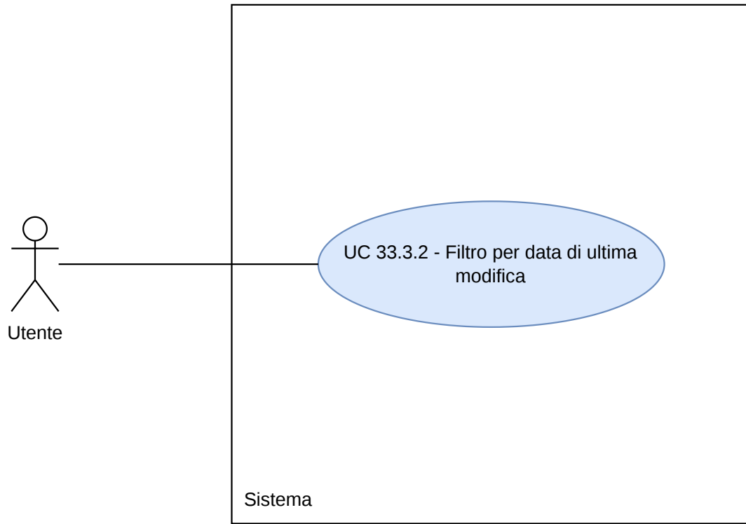
Figura 135: Diagramma UC33.3.2
