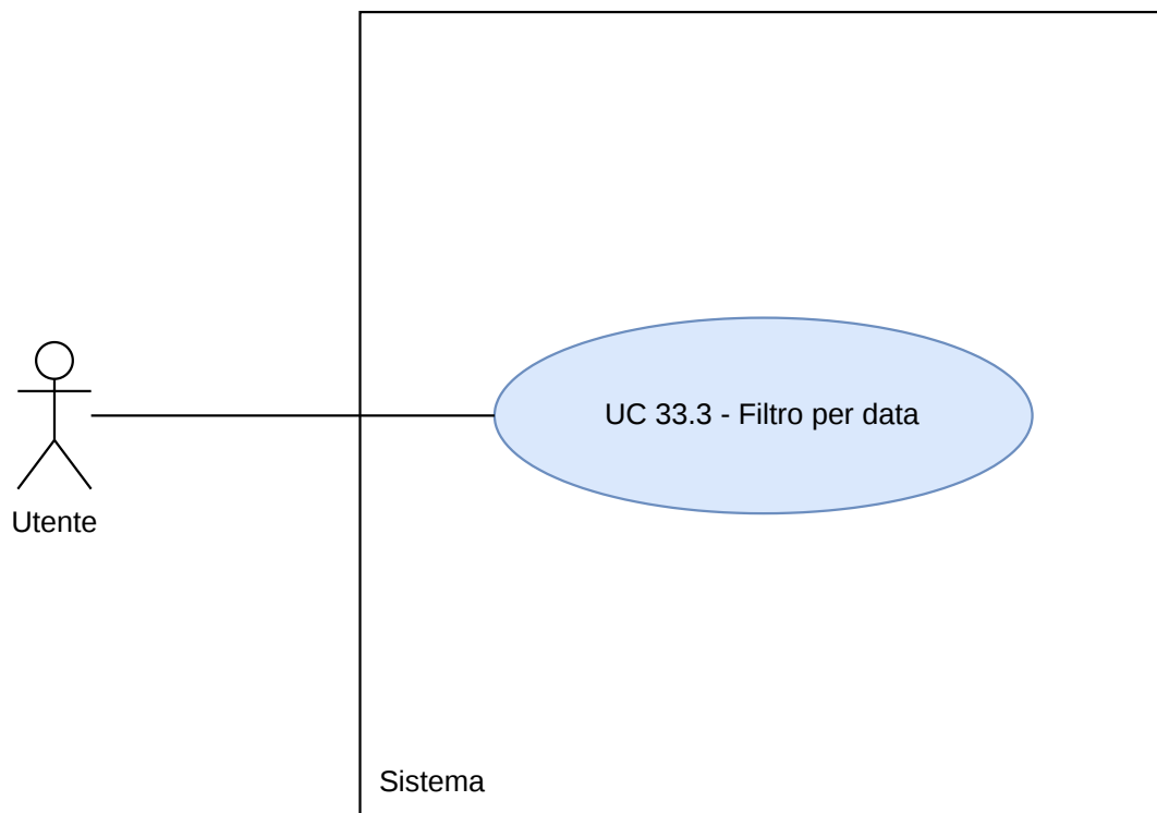
Figura 133: Diagramma UC33.3
