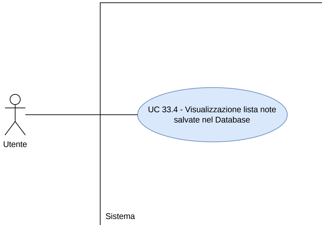
Figura 136: Diagramma UC33.4
