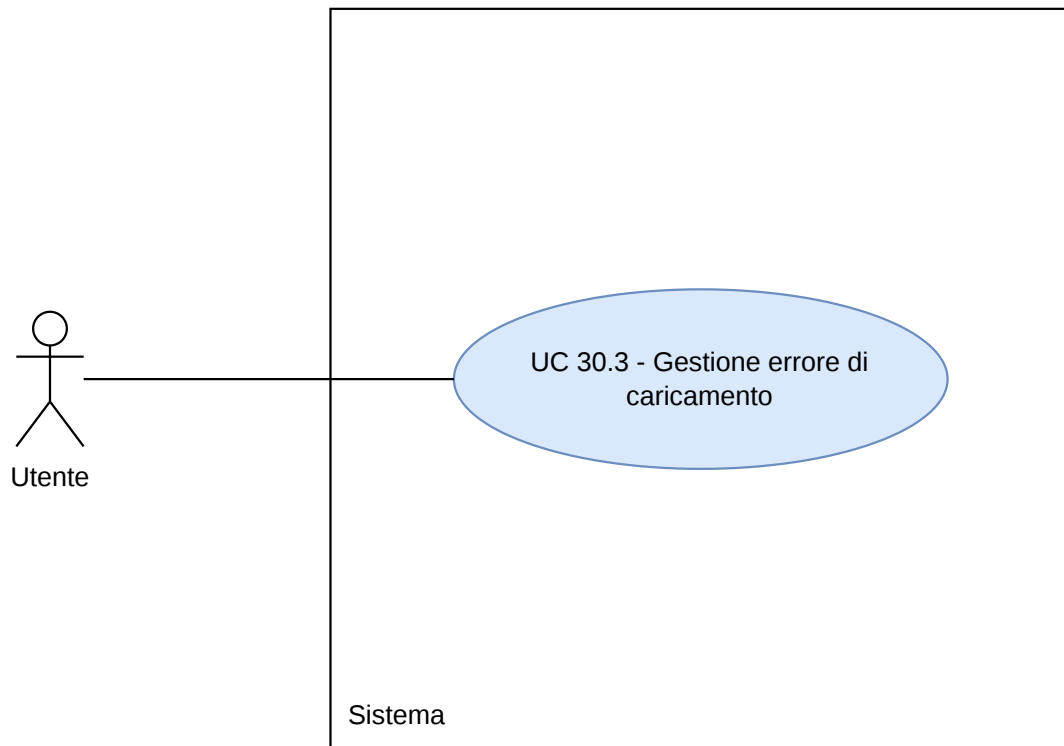
Figura 119: Diagramma UC30.3
