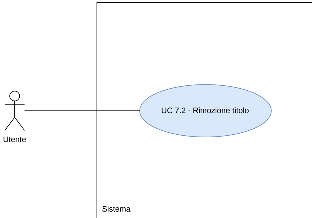
Figura 25: Diagramma UC7.2
