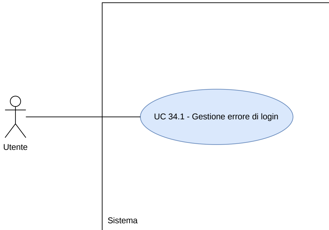
Figura 138: Diagramma UC34.1
