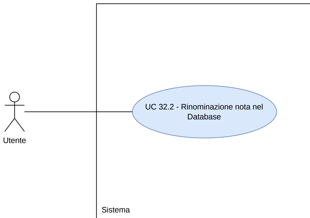
Figura 127: Diagramma UC32.2
