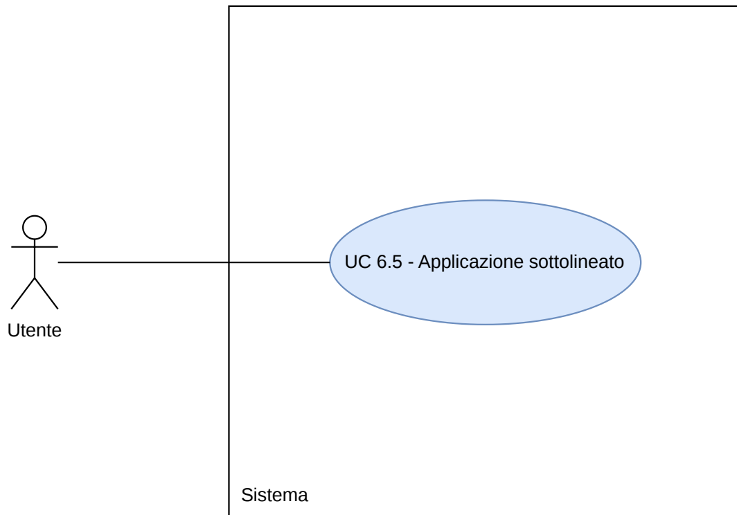
Figura 17: Diagramma UC6.5
