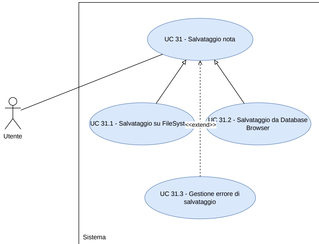
Figura 120: Diagramma UC31
