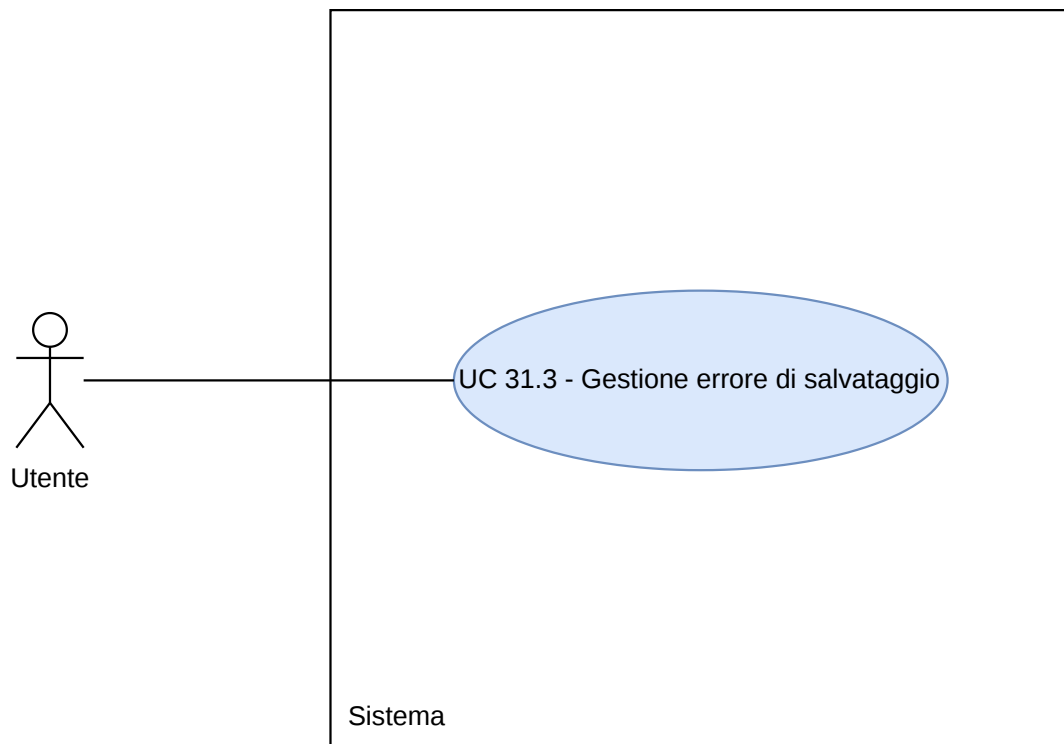
Figura 123: Diagramma UC31.3
