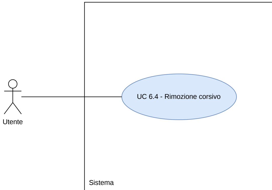
Figura 16: Diagramma UC6.4
