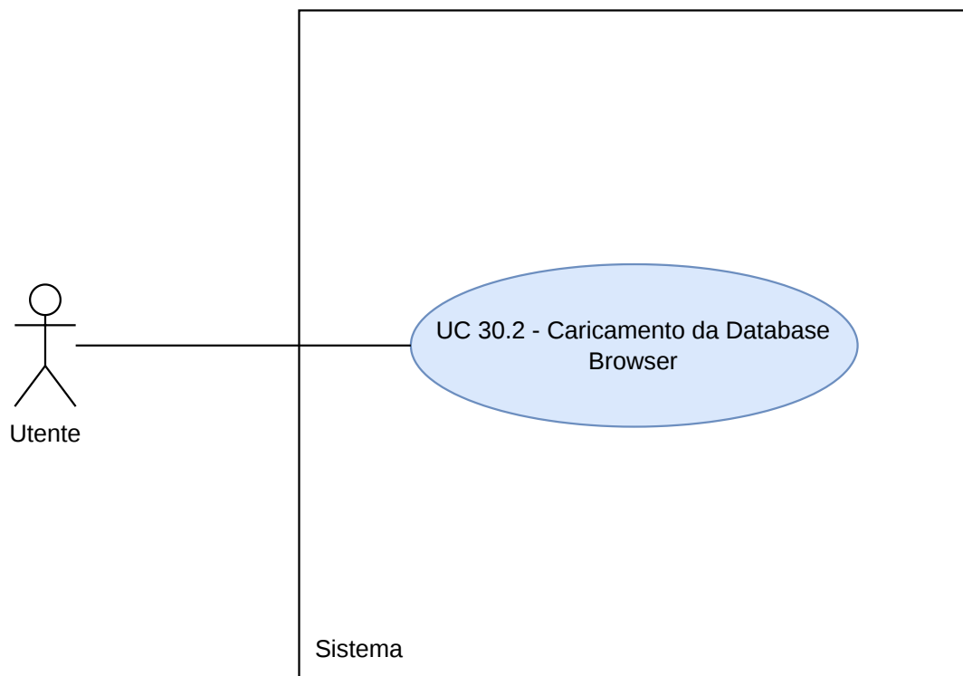
Figura 118: Diagramma UC30.2
