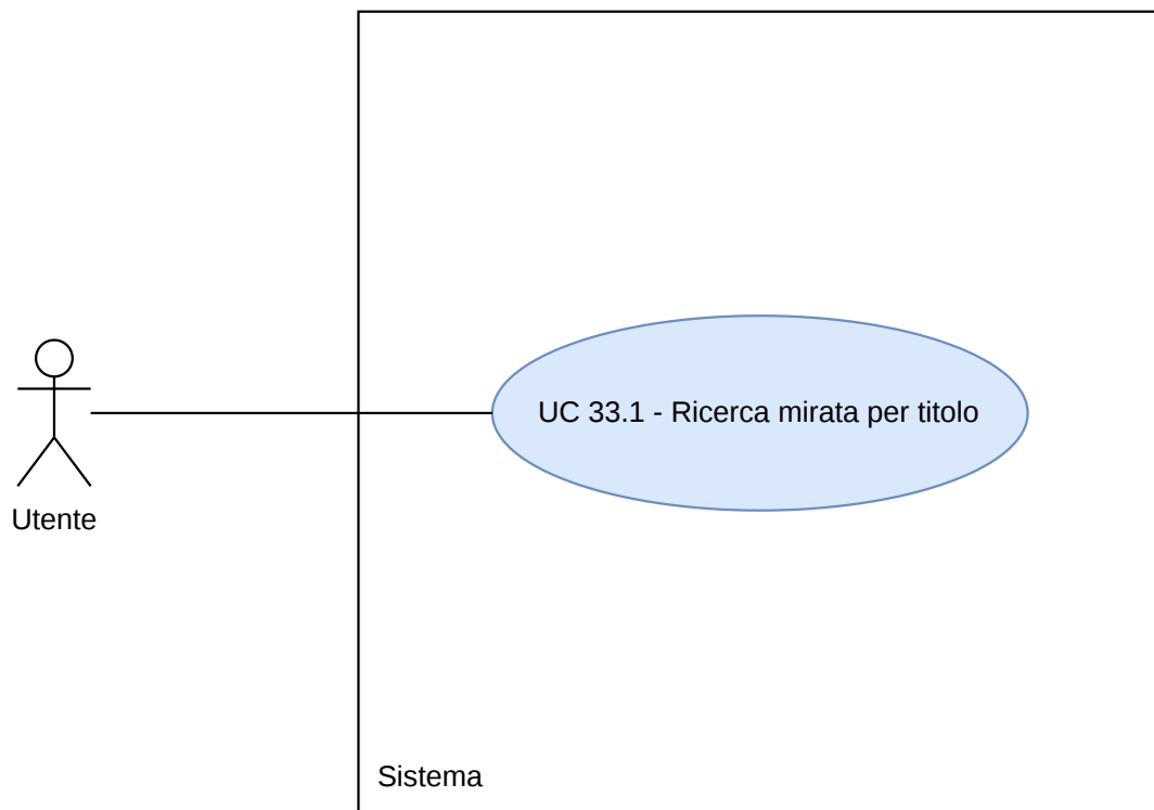
Figura 131: Diagramma UC33.1
