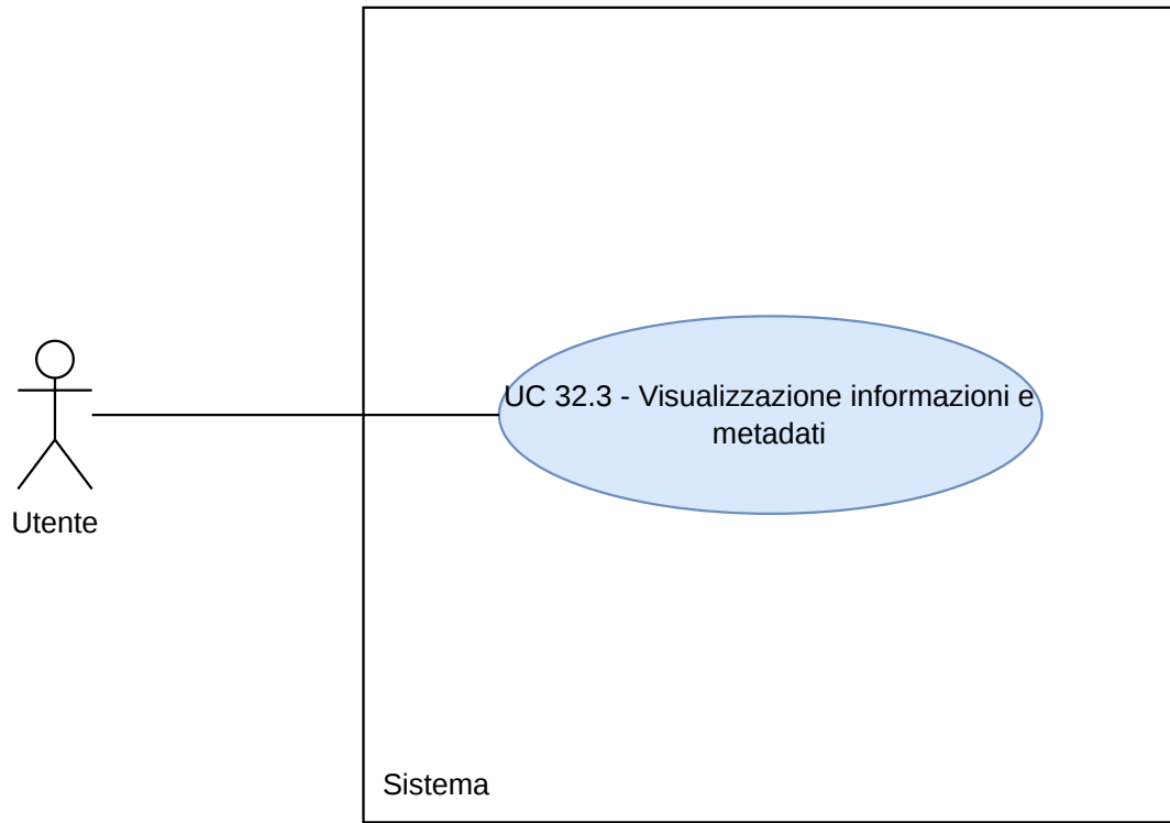
Figura 129: Diagramma UC32.3
