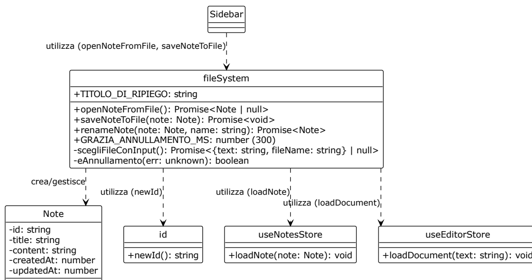
Figura 34: Diagramma UML 4.4.1-3 - openNoteFromFile
