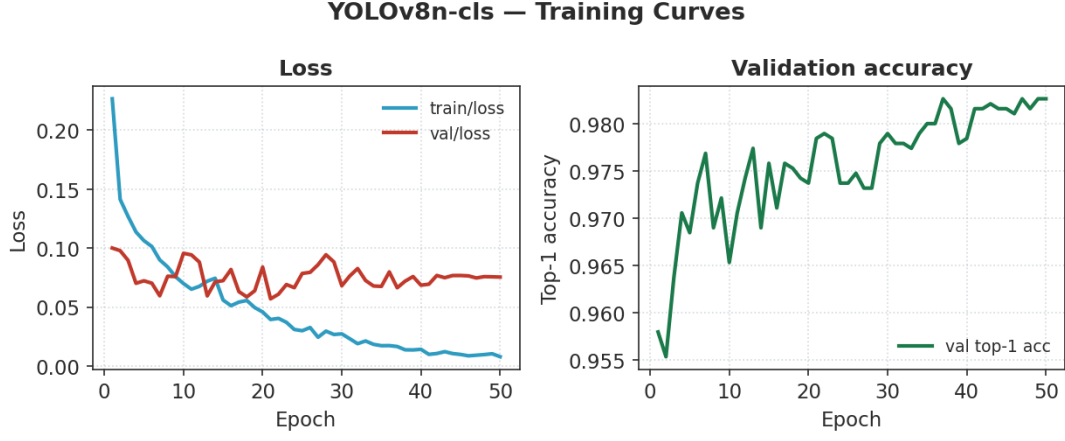
Figure 4: YOLOv8n-cls training curves on warped ACPDS patches ( runs/acpds_cls/yolov8n_stage2 ): train/validation loss and top-1 accuracy over 50 epochs.
