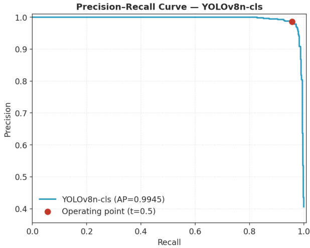
Figure 9: Precision-recall curve for YOLOv8n-cls on the test split (average precision 0.9945); the threshold-0.5 operating point is marked. Regenerated from the promoted checkpoint by ml/make_report_figures.py (make figures).
