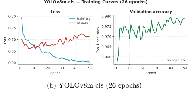
Figure 6: Training curves for the comparison variants: train/validation loss and validation top-1 accuracy.
