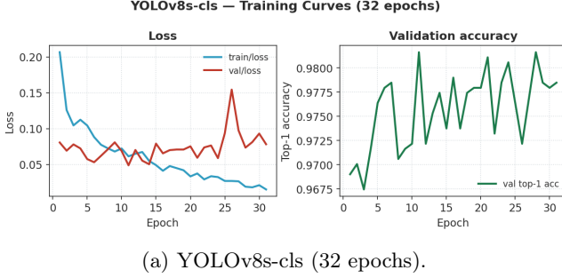
Figure 6: Training curves for the comparison variants: train/validation loss and validation top-1 accuracy.
