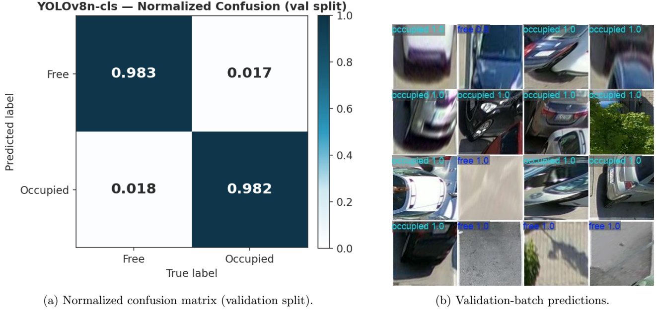
Figure 5: YOLOv8n-cls qualitative results on the validation split. The confusion matrix (a) shows balanced performance across the occupied and free classes (the held-out test -split matrix is reported separately in Figure 8); (b) shows predicted labels on warped validation patches.
