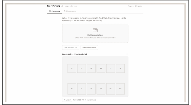
Figure 12: Owner setup (web): the photo-upload area and the resulting 12-spot layout panel (“Layout ready — 12 spots detected”), ready to publish as the lot map. The spots shown are a sample placeholder grid ( spot_source: placeholder_grid ) used to exercise the UI; real quadrilateral extraction on ACPDS imagery is shown in Figures 1 and 3.
