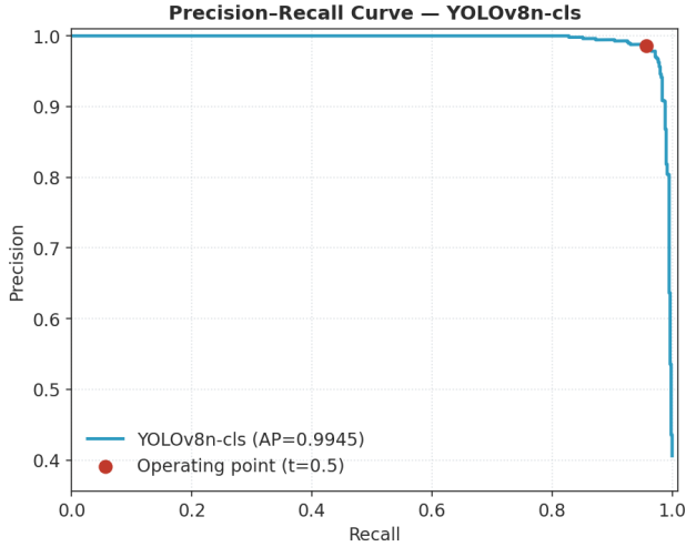
Figure 9: Precision-recall curve for YOLOv8n-cls on the test split (average precision 0.9945); the threshold-0.5 operating point is marked. Regenerated from the promoted checkpoint by ml/make_report_figures.py ( make figures ).
