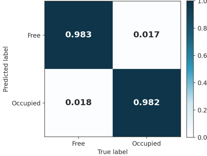
(a) Normalized confusion matrix.
