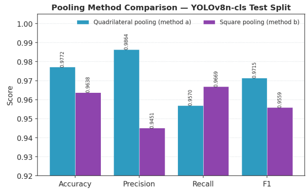
Figure 11: Quadrilateral vs. square pooling on the test split. Quad wins on all metrics except recall.
