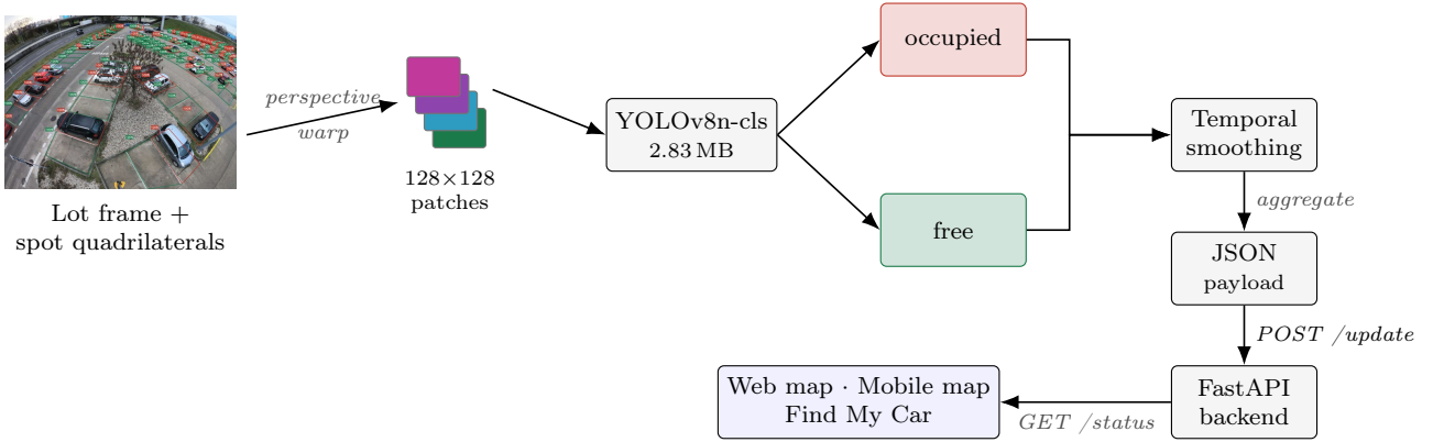
Figure 1: End-to-end system architecture. A lot frame with quadrilateral spot annotations is pooled into perspective-corrected 128 \times 128 patches, classified by YOLOv8n-cls, temporally smoothed, and reported as compact JSON to the FastAPI backend, which drives the web/mobile occupancy maps and Find My Car. Only the JSON leaves the edge device.
