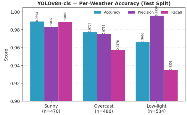
Figure 10: Per-weather accuracy, precision, and recall for YOLOv8n-cls on the test split.
