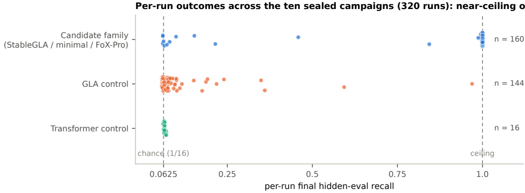
Figure 5: Recall acquisition is bimodal. Per-run final hidden-eval recall for all 320 runs of the ten sealed claim campaigns (m, q, r, t, u, ag, aj, ak, am, aq), by architecture family: outcomes sit at the ceiling or at the 1/16 chance floor. The few runs between are mid-transition candidates caught at budget exhaustion or GLA controls climbing at escalated budget (§4.4).
