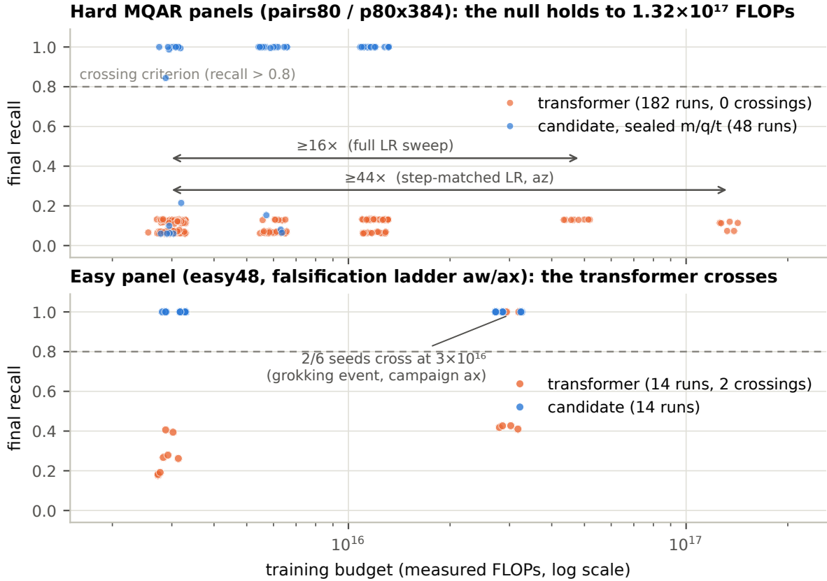
Figure 6: Where attention’s threshold lies, and where it does not. Top: on the hard MQAR panels the transformer crosses in none of 182 runs (recomputed from run artifacts by the released recount script) at budgets to 1.32 \times 10^{17} FLOPs, while the sealed candidate transitions from 3 \times 10^{15} — a tested separation of at least sixteenfold across the full learning-rate sweep and at least fortyfold at the step-matched rate (campaign az). Bottom: on the deliberately easy panel the same transformer crosses — 2 of 6 seeds at 3 \times 10^{16} FLOPs, a textbook grokking event (campaign ax) — so the null is a threshold claim, not an incapacity claim.
