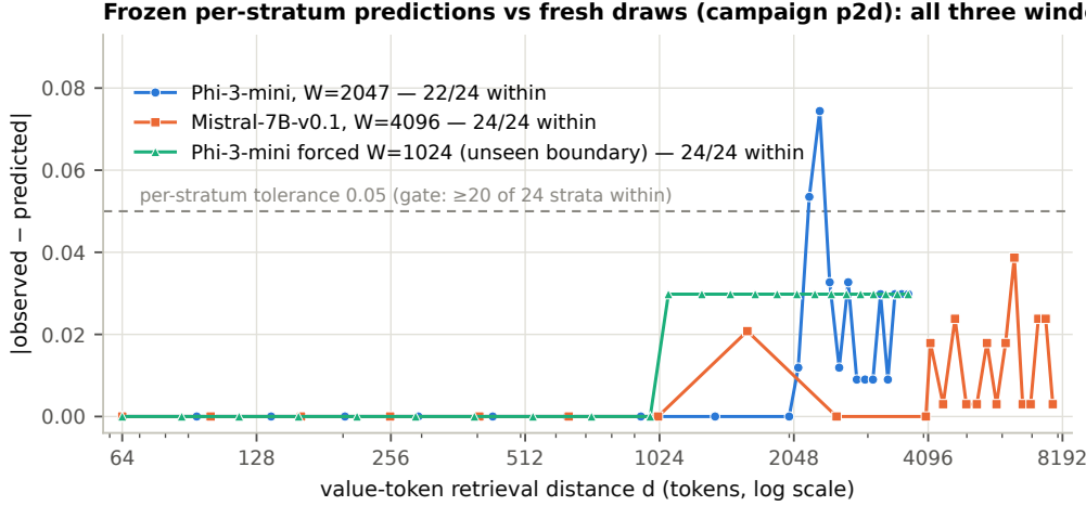
Figure 4: The frozen-prediction pass (campaign p2d). Per-stratum |\text{observed} - \text{predicted}| for the three windowed arms, with every numeric prediction frozen from p2c’s fitted instrument before any probe was scored, on fresh evaluation draws. All three arms pass the pre-registered gate ( \geq 20 of 24 strata within 0.05), including at the never-fitted boundary W = 1024 . The window-disabled control arm (not shown) triggered the campaign’s pre-registered confound branch, so the aggregate transfer claim stays suspended (§4.3).
