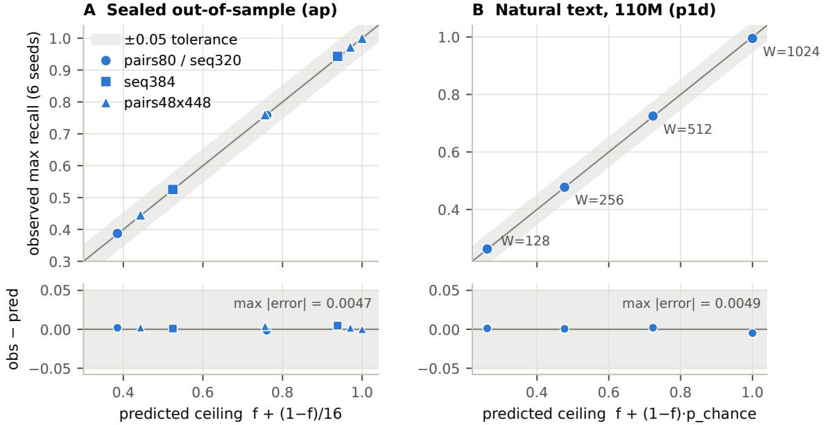
Figure 1: The window-provisioning law, predicted versus observed. (A) The eight sealed out-of-sample cells of campaign ap, across three task geometries: numeric ceilings f + (1 - f)/16 were committed to an append-only ledger before any training result existed, and the observed max-over-6-seeds recall matches every cell within 0.005 (residual strip, bottom) against a pre-registered \pm 0.05 tolerance. (B) The same law on natural text at 110M parameters (campaign p1d, seed 2100): all four windowed cells calibrate inside 0.005, at 8\times the parameter count of the synthetic test.
