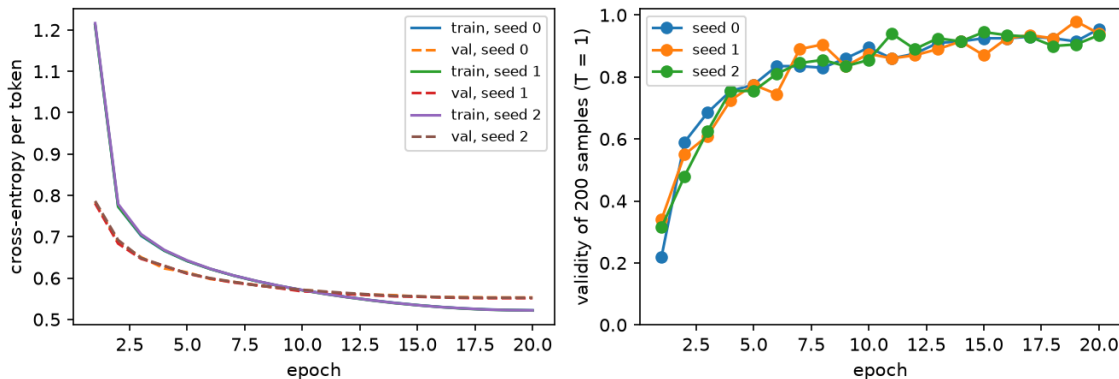
Figure 2. Training and validation cross-entropy per epoch, and the validity of 200 raw samples per epoch.
