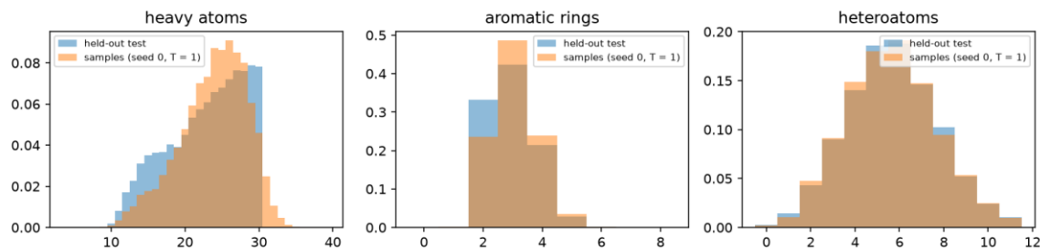
Figure 3. Sample distributions against the held-out test set.
