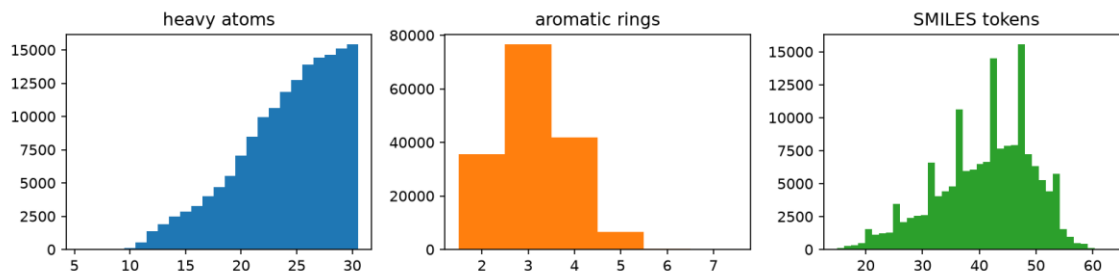
Figure 1. Heavy-atom, aromatic-ring and token-length distributions of the frozen set.
