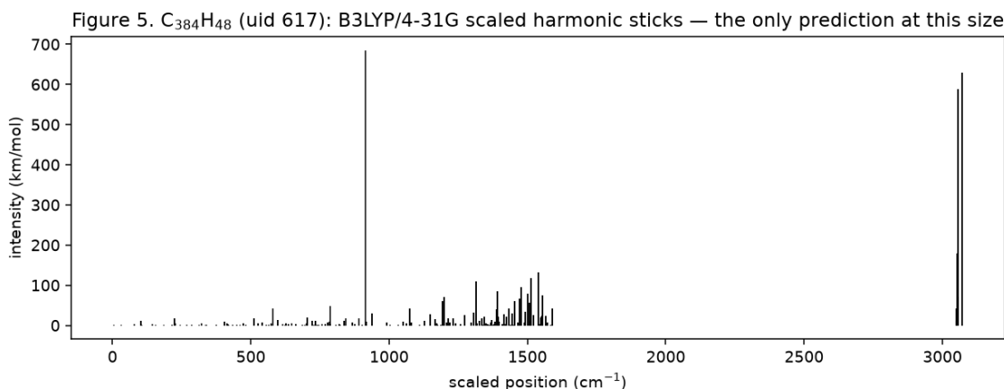
Figure 5. C_{384}H_{48} (uid 617): the scaled harmonic stick spectrum at B3LYP/4-31G, 1,290 modes.
