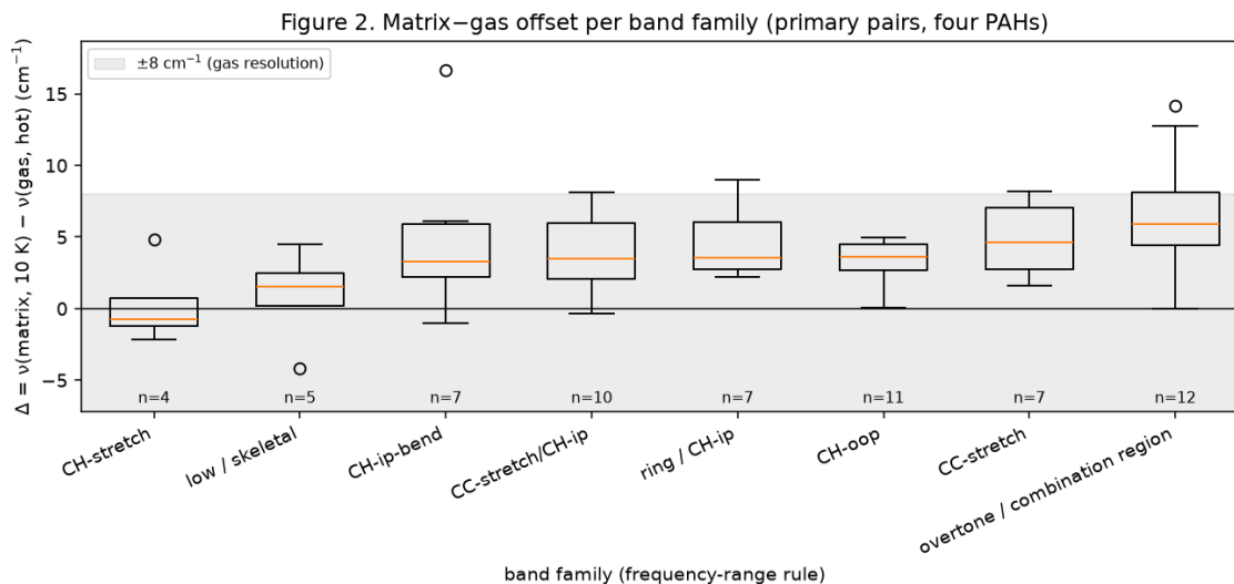
Figure 2. Offset \Delta = v(\text{matrix}, 10 \text{ K}) - v(\text{gas}, \text{hot vapour}) per band family, primary pairs of four PAHs; the grey band is \pm 8 \text{ cm}^{-1} , the gas resolution.
