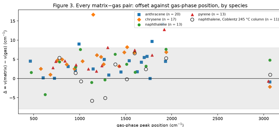
Figure 3. Every pair's offset against its gas-phase position, by species; hollow circles are naphthalene against the 245 °C Coblenz record (secondary column).
