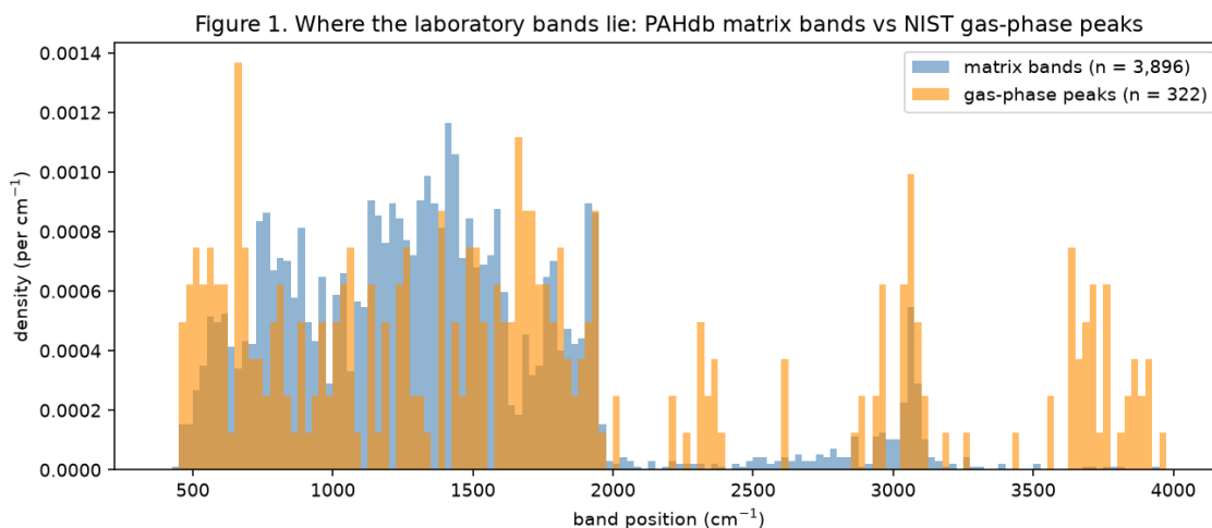
Figure 1. Band positions of the matrix library and the gas-phase peaks (densities per \text{cm}^{-1} , 25 \text{ cm}^{-1} bins).
