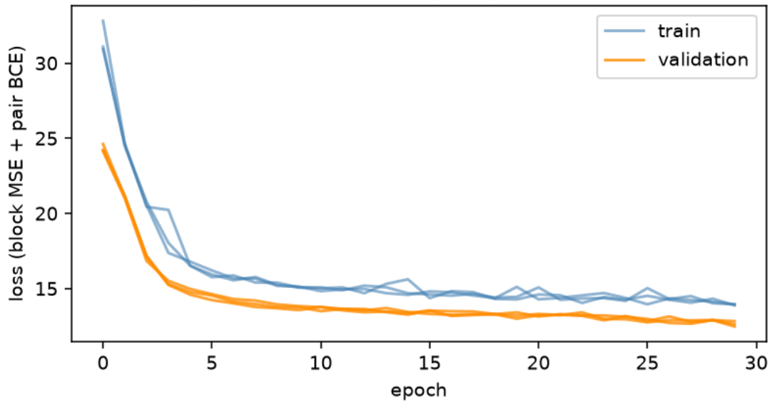
Figure 1. Baseline: training and validation loss per epoch.
