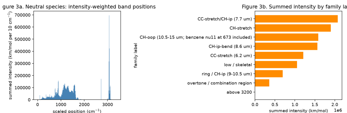
Figure 3. Neutral species: intensity-weighted band positions (left) and summed intensity per frequency-range family label (right).
