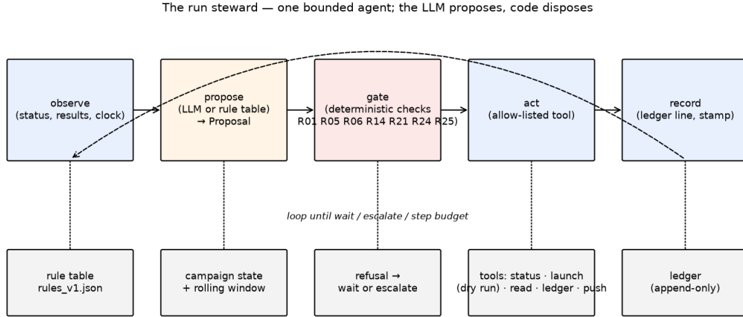
Figure 1. The run steward: one bounded agent. The reasoning node proposes; the deterministic gate disposes; every step is recorded.
