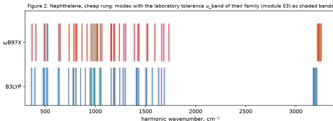
Figure 2. Naphthalene at the cheap rung: modes of both functionals with the laboratory tolerance of their family shaded; no predicted band is drawn.
