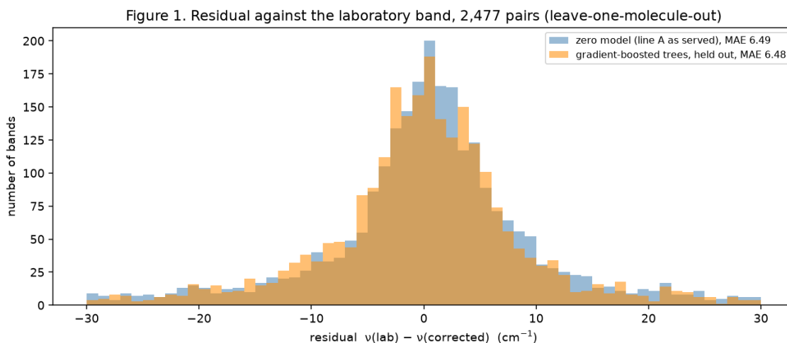
Figure 1. Residual of the corrected band position against the laboratory band: uncorrected library versus gradient-boosted trees (held out).
