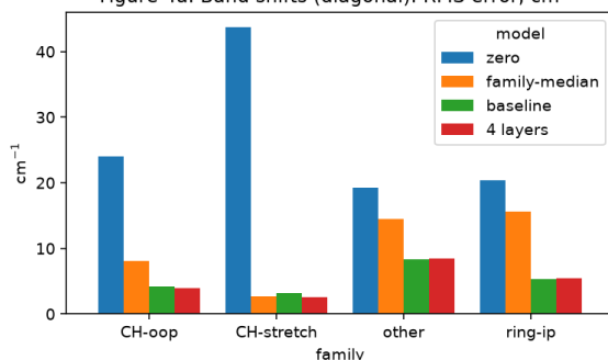
Figure 4a. Band shifts (diagonal): RMS error, \text{cm}^{-1}
