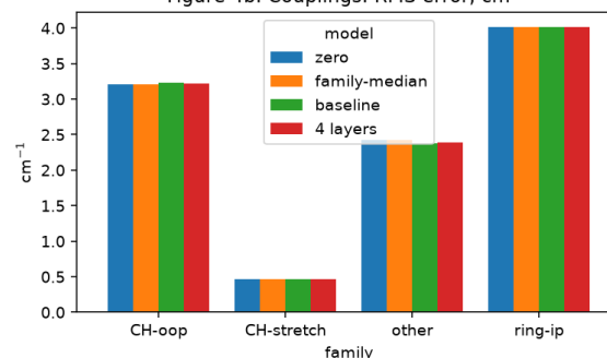
Figure 4b. Couplings: RMS error, \text{cm}^{-1}
