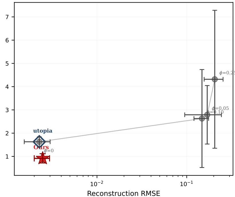
(b) Brusselator
