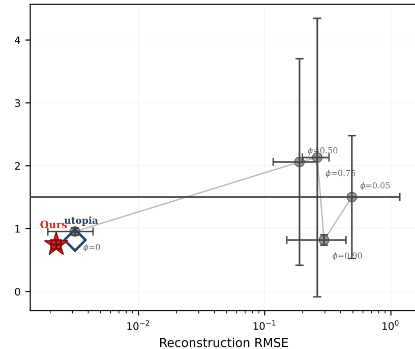
(c) Duffing
