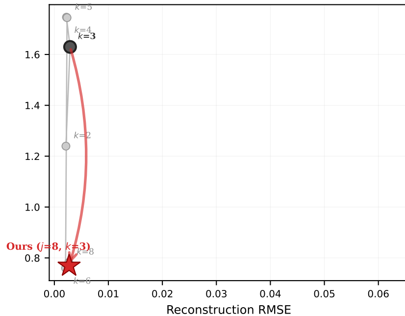
(b) Brusselator
