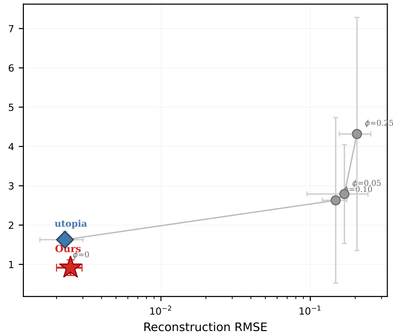
(b) Brusselator
