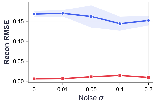
Coupled Harmonic
