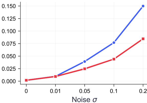
Brusselator
