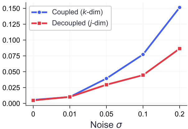
Duffing
