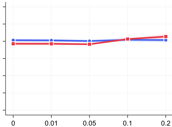
Duffing
