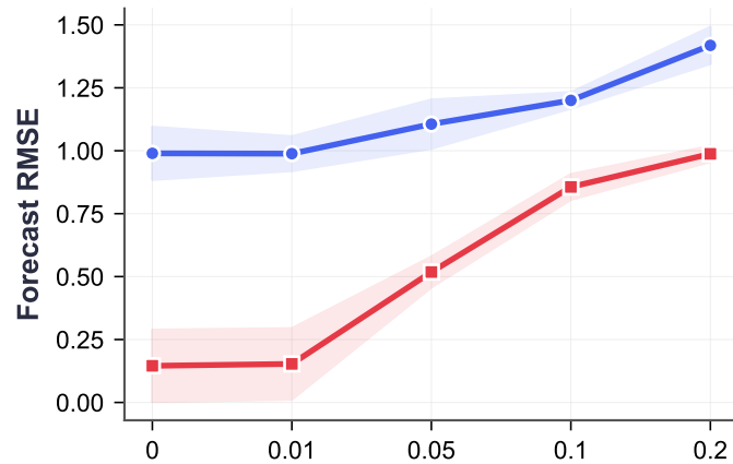
Coupled Harmonic
