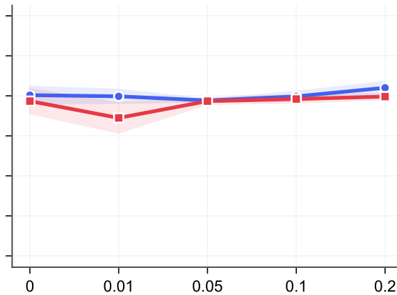
Brusselator
