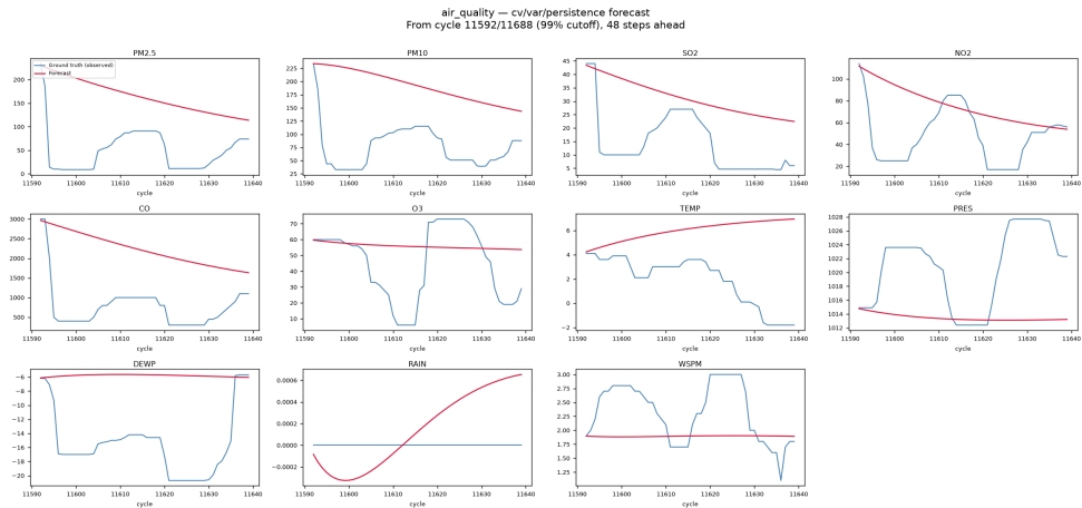
Figure 20: Air-quality decoded forecasts (red) versus ground truth (blue) from a mid-trajectory cutoff, per variable.
