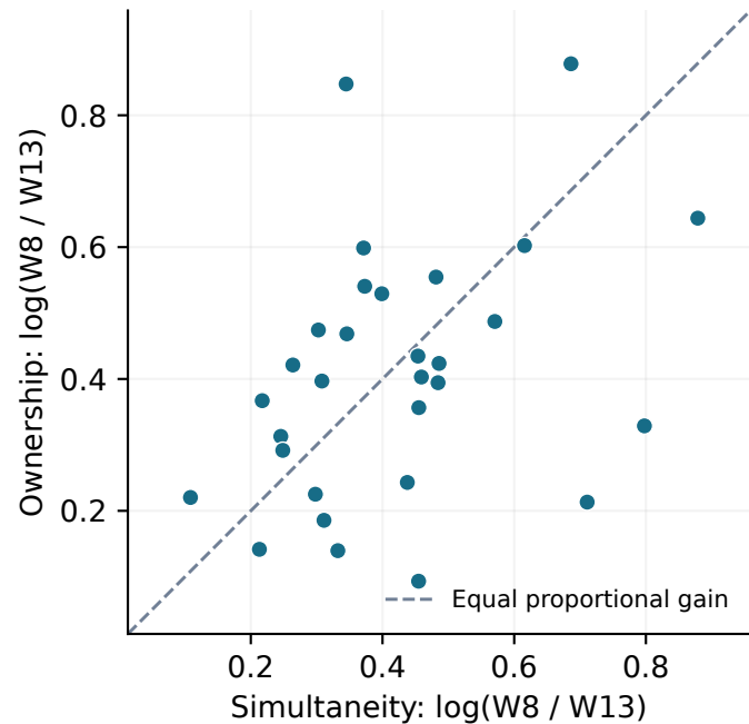
A Released participant estimates
