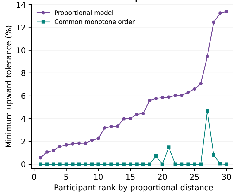
B Exact distances of point estimates
