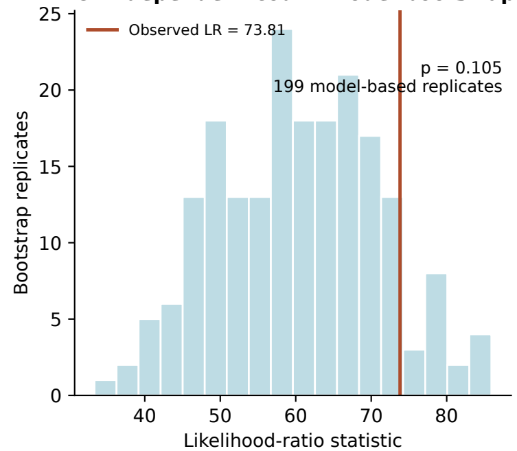
C Independent count-model bootstrap
